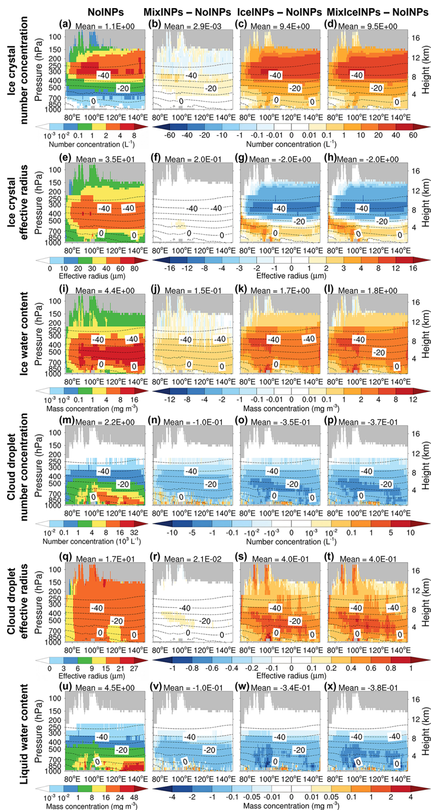
Figure 5. Simulated meridional mean vertical cross-sections of (a–d) ice crystal number concentration, (e–h) ice crystal effective radius, (i–l) ice water content, (m–p) cloud droplet number concentration, (q–t) cloud droplet effective radius, and (u–x) liquid water content, for the NoINPs (first column), MixINPs – NoINPs (second column), IceINPs – NoINPs (third column), and MixIceINPs – NoINPs (fourth column) scenarios. Dashed lines indicate isotherms, and grey shading denotes missing values due to terrain or filtering of non-cloud grid cells (where the sum of ice and liquid water mixing ratios is less than 10^{-6} \text{ kg kg}^{-1} ). The mean value over the plotted region is shown above each panel. The simulated results are averages of hourly values from March to May 2018.
