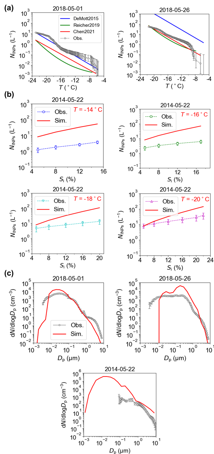
Figure 2. Comparison of simulated and observed dust INP number concentrations and particle number size distributions (PNSDs). (a) Simulated dust INP number concentrations in mixed-phase clouds compared with observations on 1 and 26 May 2018 at the Peking University Atmosphere Environment Monitoring Station (116.31° E, 39.99° N). N_{\text{INPs}} denotes the number concentration of dust INPs, and T denotes the temperature. (b) Simulated dust INP number concentrations in ice clouds compared with observations at -14 , -16 , -18 , and -20 ^{\circ}\text{C} on 22 May 2014 at the Kuqa Meteorological Bureau (83.04° E, 41.43° N) in the Aksu region of Xinjiang, China. S_i denotes ice supersaturation, Obs. denotes observations, and Sim. denotes simulations. (c) Simulated PNSDs compared with observations from the same stations and dates as in panels (a) and (b). N denotes the aerosol number concentration, and D_p denotes the aerosol diameter. Error bars indicate the 95 % confidence intervals for the observations. The simulated results are from the MixIceINPs scenario and represent averages of hourly values.
