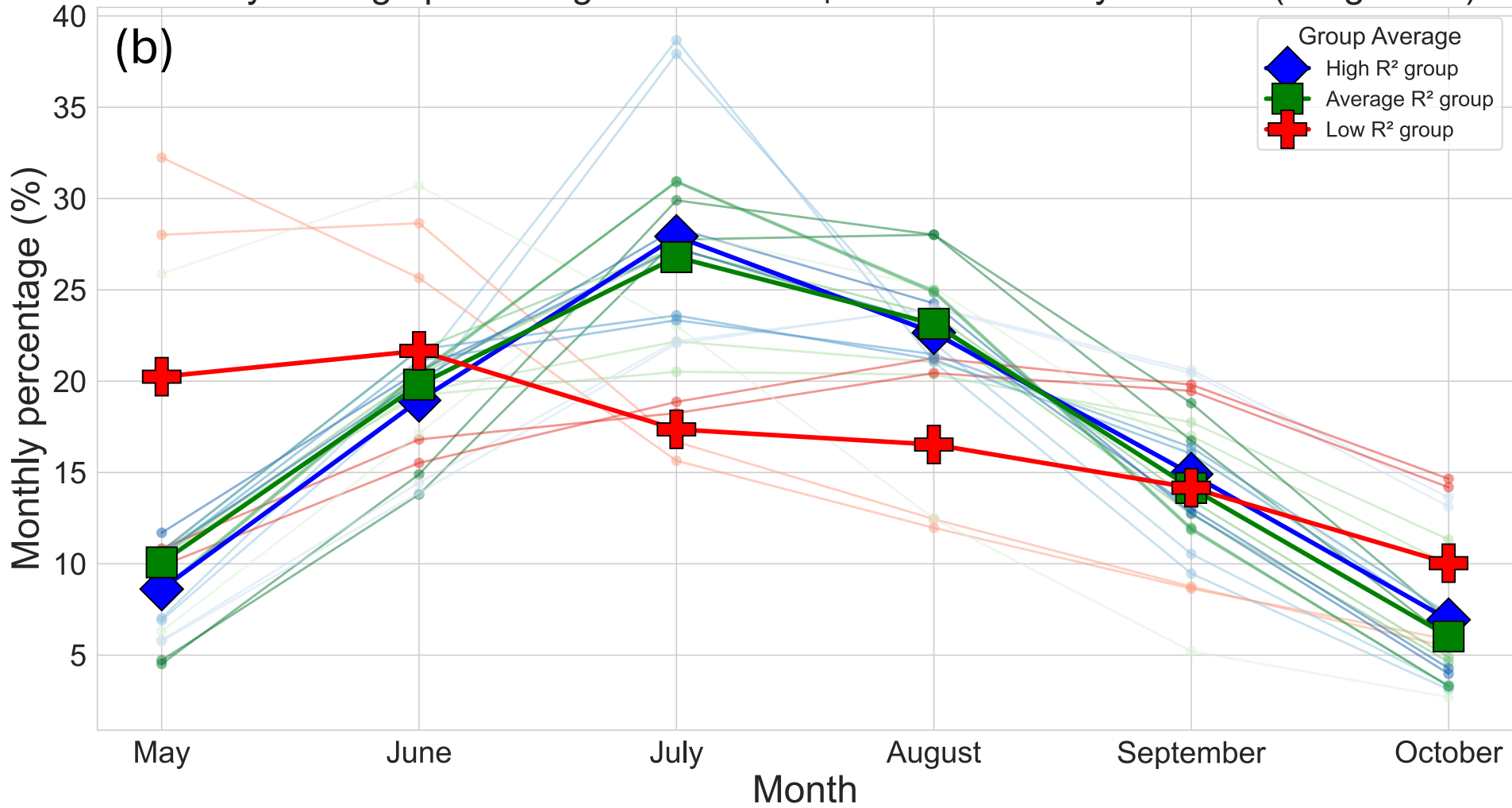
Monthly average percentage of GCP CH 4 fluxes from May-October (Prognostic)
