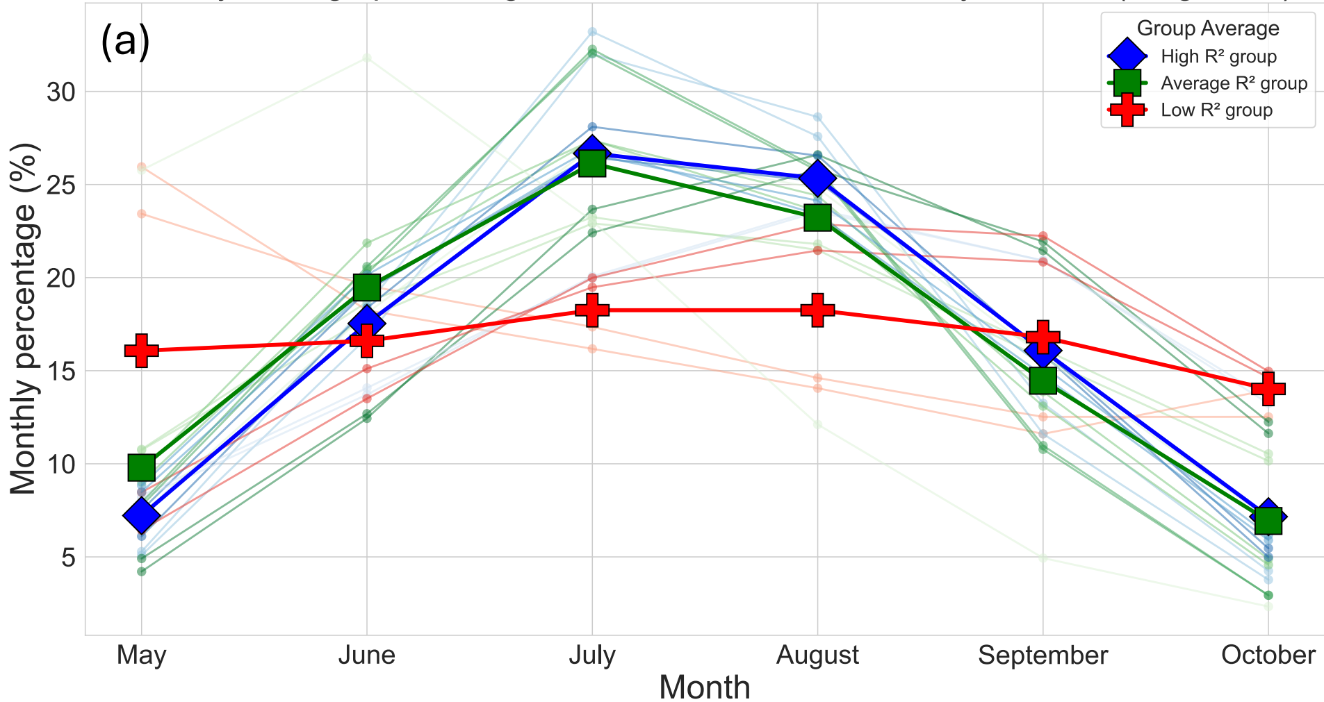
Monthly average percentage of GCP CH 4 fluxes from May-October (Diagnostic)
