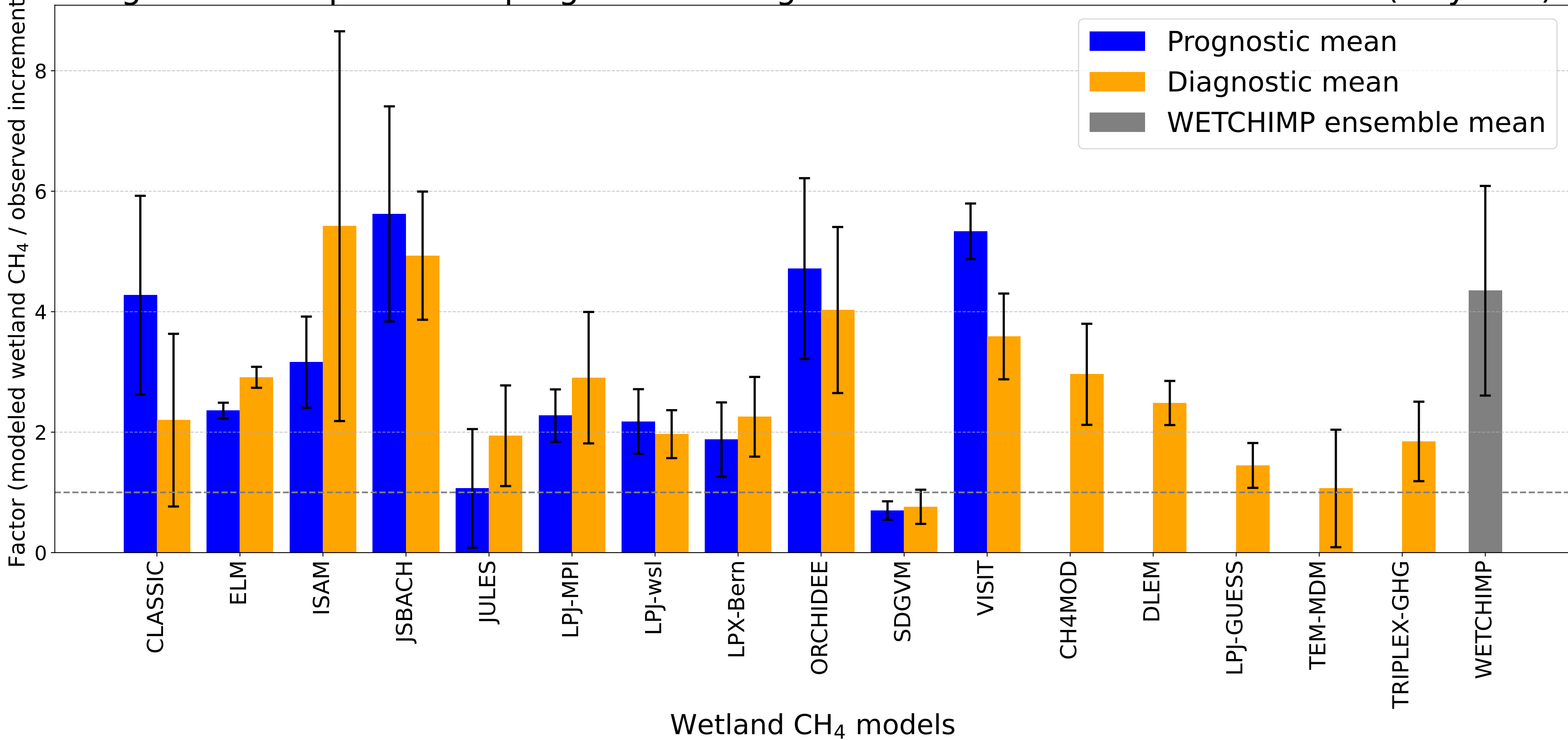
Magnitude comparison of prognostic & diagnostic GCP models with WETCHIMP (May-Oct)
