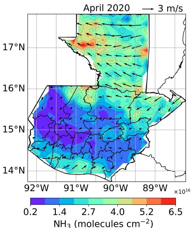
Figure 9. Monthly mean area-wide of NH 3 total column ( \times 10^{16} molecules \text{cm}^{-2} ) from the concatenated IASI A, B and C, and wind mean vectors from ERA5 over Guatemala (April 2020).
