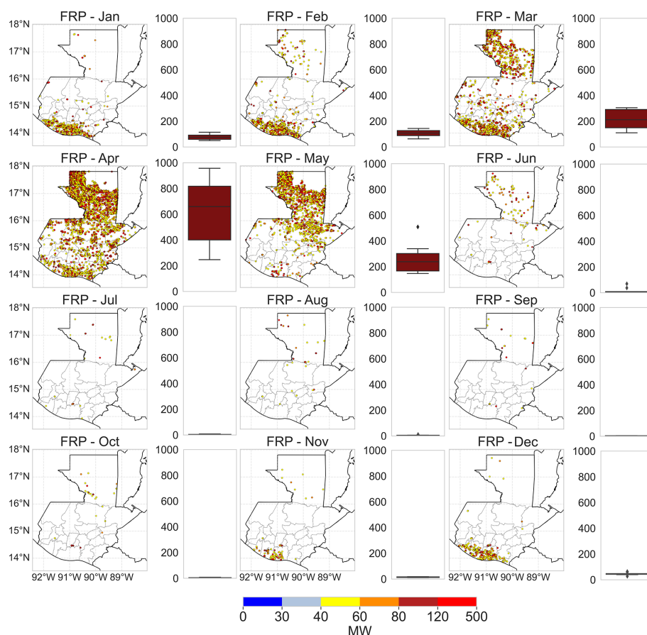
Figure 7. Monthly climatology of MODIS active-fire detection and distribution of fires count over Guatemala (2015–2023). Maps show detected fire location for each calendar month, colored according to FRP (MW), fire detection were filtered by nominal confidence level \geq 70\% and \text{FRP} \geq 40 MW, the boxplots represent the distribution area-wide of fire counts for each calendar month across all years.
