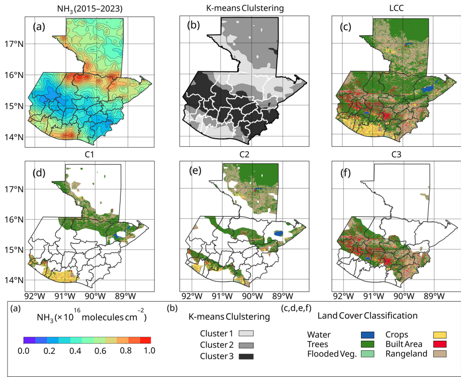
Figure 4. (a) Concatenated NH 3 total column (× 10 16 molecules cm -2 ) (2015–2023), (b) k -means cluster analysis with Cluster 1 (black color), Cluster 2 (gray color) and Cluster 3 (light gray color). (c) ESRI Land Use Land Cover across Guatemala, categorized into three clusters based on k -means combined with land cover types: water, trees, flooded vegetation, crops, built area, and rangeland, (d) C1 related to cluster 1, (e) C2 to cluster 2, and (f) C3 to cluster 3.
