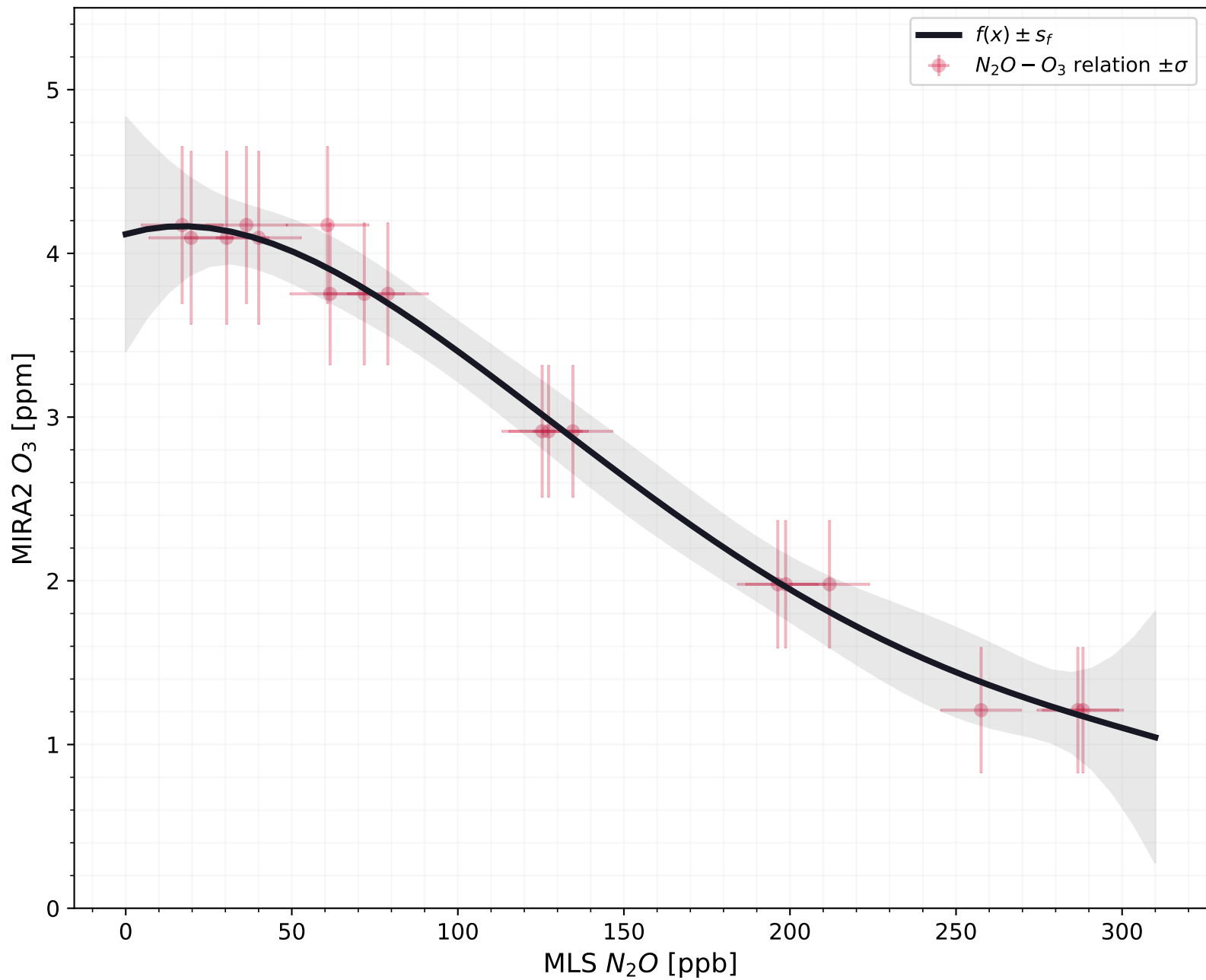
N_2O - O_3 relation on 2019-12-09 in 400 \leq \theta \leq 600 K
