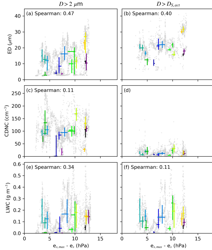
Figure S17. Campaign-based Spearman correlation of cooling (difference between water saturation vapor pressure corresponding to the maximum temperature of the day and that to the current temperature) and fog microphysical parameters. (a) and (b) correlation with the effective diameter (ED). (c) and (d) correlation with the cloud droplet number concentration (CDNC). (e) and (f) correlation with the liquid water content (LWC). (a), (c), and (e) for D_{\text{wet}} > 2 \mu\text{m} , (b), (d), and (f) for D_{\text{wet}} > D_{\text{wet,act,S}} . The interquartile ranges of the fog events are shown, color-coded by the number of the fog events. The Spearman correlation is based on all underlying data points (grey dots) and given if p < 0.01 . The LWC is taken from the PVM measurements. The data is based on 1 min averages.
