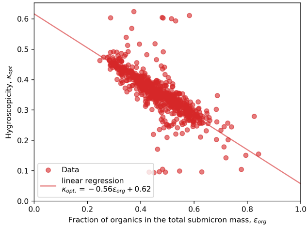
Figure S2. Hygroscopicity parameter \kappa_{\text{opt}} vs. the organic fraction measured out of fog during FAIRARI. The red line denotes a least-squared linear regression.
