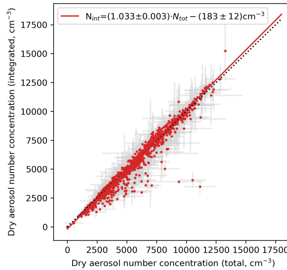
Figure S4. Closure between the dry aerosol number concentration measured by the total Condensation Particle Counter (CPC) and the integrated size distribution. Mean values of 1 h are shown with the standard deviations shown as gray bars. The weighted bivariate linear fits were calculated following York et al. (2004).
