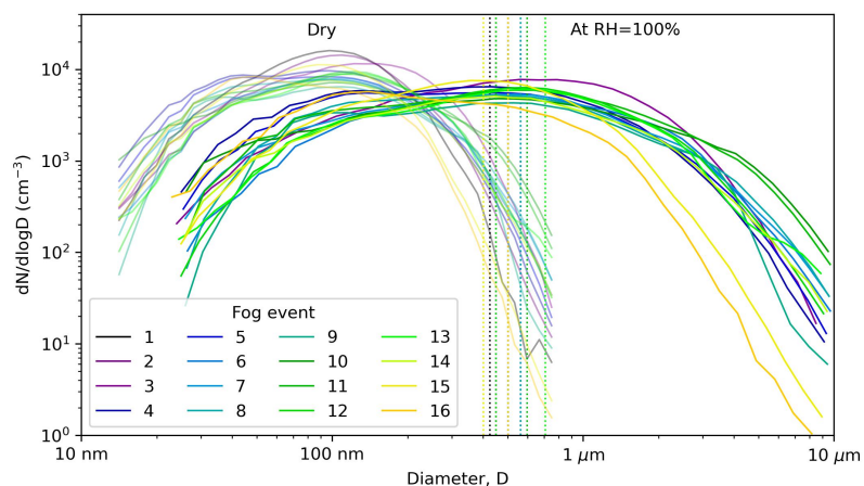
Figure S7. Median size distributions (dry and at 100 % relative humidity) for the fog events measured during FAIRARI. The median dry activation diameters are shown as vertical lines.
