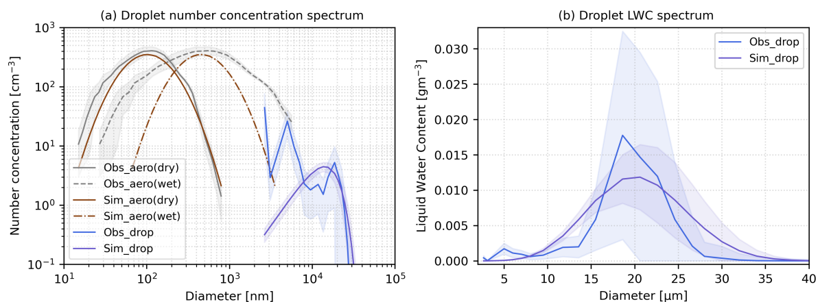
Figure S9. Mean size distributions of (a) aerosol and cloud droplet number concentrations and (b) droplet LWC from observations (obs) and simulations (sim), averaged over the last 4 hours of fog event 7. “Dry” and “wet” refer to aerosol states before and after hygroscopic growth, respectively. Shaded areas indicate \pm 1 standard deviation.
