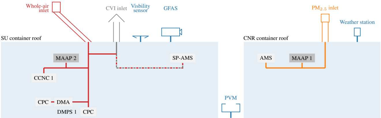
Figure S1. Schematic of the experimental setup used for this study during Fog and Aerosol InteRAction Research Italy (FAIRARI) (adapted from Neuberger et al., 2025). Instruments behind a drier are indicated by a light gray background. Inlets/tubings of ambient air are colored. Ambient measurements are in blue. A list of acronyms can be found at the end of the main manuscript.
