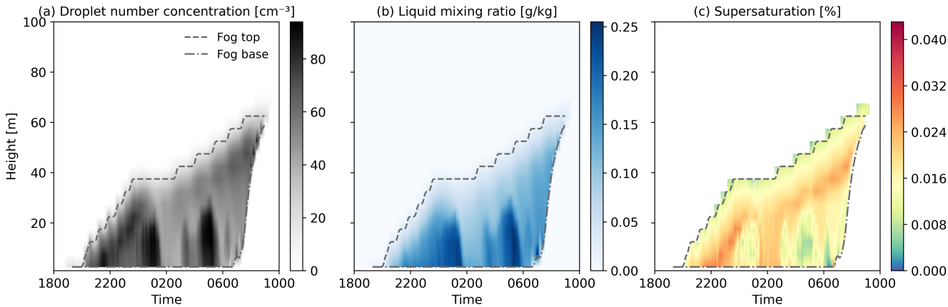
Figure S8. Vertical cross-sections of (a) droplet number concentration, (b) liquid water mixing ratio, and (c) supersaturation from simulations for the fog event on 18–19 February 2022. The dashed lines indicate the fog base and top, defined as the height range where the droplet number concentration is \geq 1 \text{ cm}^{-3} and the liquid water mixing ratio is \geq 0.01 \text{ g kg}^{-1} .
