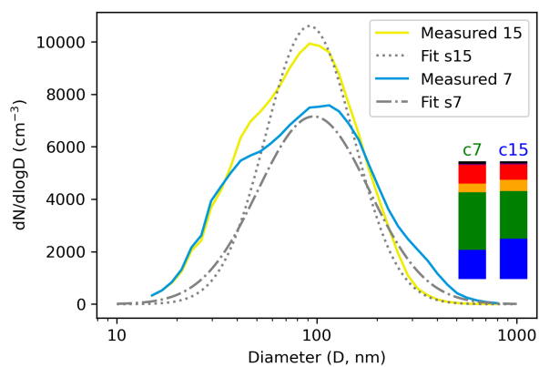
Figure S10. Input parameters for LES modeling. Measured dry aerosol number size distribution (together with a single lognormal fit) and chemical composition for fog event 7 and 15.
