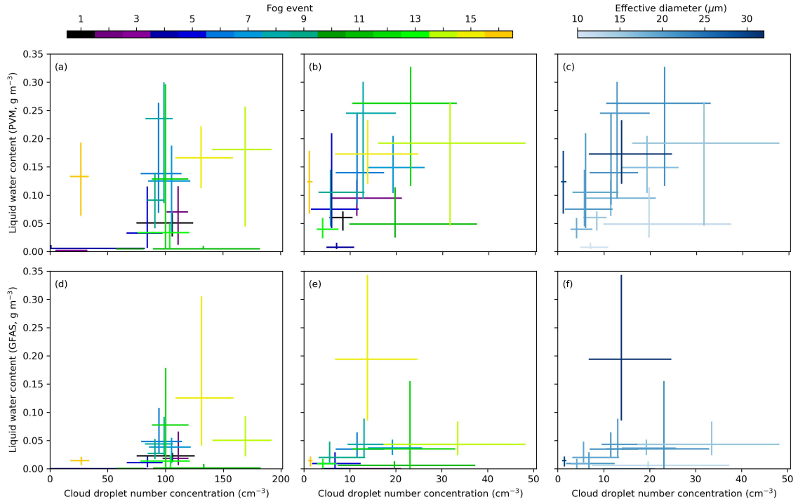
Figure S13. Effect of hydrated aerosol particles on cloud droplet number concentration (CDNC). The interquartile ranges are shown for each fog event. (a) and (d) CDNC is calculated for D_{\text{wet}} > 2 \mu\text{m} . (b) and (e) CDNC is calculated for D_{\text{wet}} > D_{\text{wet,act,S}} . (c) and (f) as (b) and (e) but colorcoded by the median effective diameter (ED). (a) – (c) Liquid water content as measured by the PVM, (d) – (f) liquid water content as measured by the GFAS. Only times where both instruments were measuring are included. The peak seen in Fig. 6(b) at \text{CDNC} = 0 \text{ cm}^{-3} is excluded.
