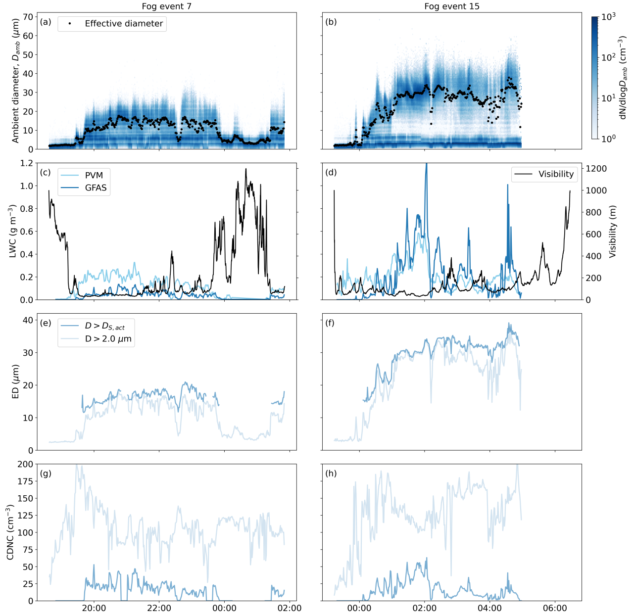
Figure S12. Fog development during event 7 and 15. (a) and (b) Ambient particle number size distributions. (c) and (d) LWC measured by the GFAS (darkblue) and the Particle Volume Monitor (PVM) (lightblue) and measured visibility. Effective diameter (ED) and cloud droplet number concentration (CDNC) are calculated with two different lower diameters ( D_{\text{wet}} > 2 \mu\text{m} and D_{\text{wet,act,s}} ) in (e)–(h).
