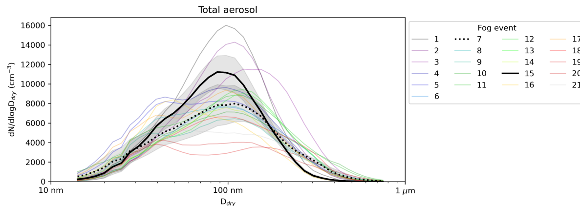
Figure S6. Mean dry particle number size distributions for the 21 fog events measured during FAIRARI. The two example fog events are highlighted in black with their standard deviation shaded in gray.
