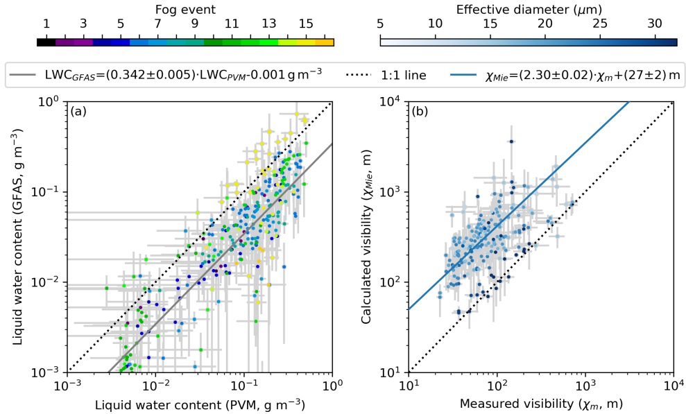
Figure S5. (a) Comparison of the liquid water content measurements by the Ground-based Fog and Aerosol Spectrometer (GFAS) and the Particle Volume Monitor (PVM) based on 10 min averages. The spearman correlation is 0.82, p \ll 0.01 . (b) Measured vs. calculated visibility using Mie theory and the GFAS observations. The weighted bivariate linear fits were calculated following York et al. (2004).
