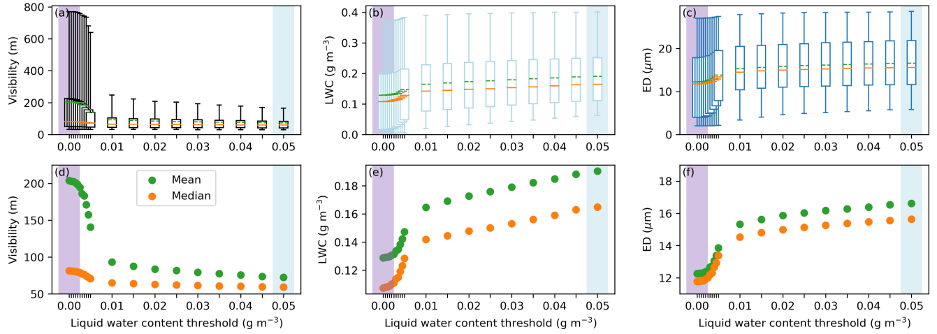
Figure S15. Effect of different fog definitions on fog microphysical parameters. In addition to the visibility criteria, a liquid water content threshold is added and varied between 0 and 0.05 \text{ g m}^{-3} to define a fog event. (a) and (d) Effect on visibility range, (b) and (e) effect on liquid water content, and (c) and (f) effect on effective diameter. In the upper panel, the boxes represent the 25 and 75 percentiles and the whiskers the 5 and 95 percentiles. The mean is given in green, the median in orange.
