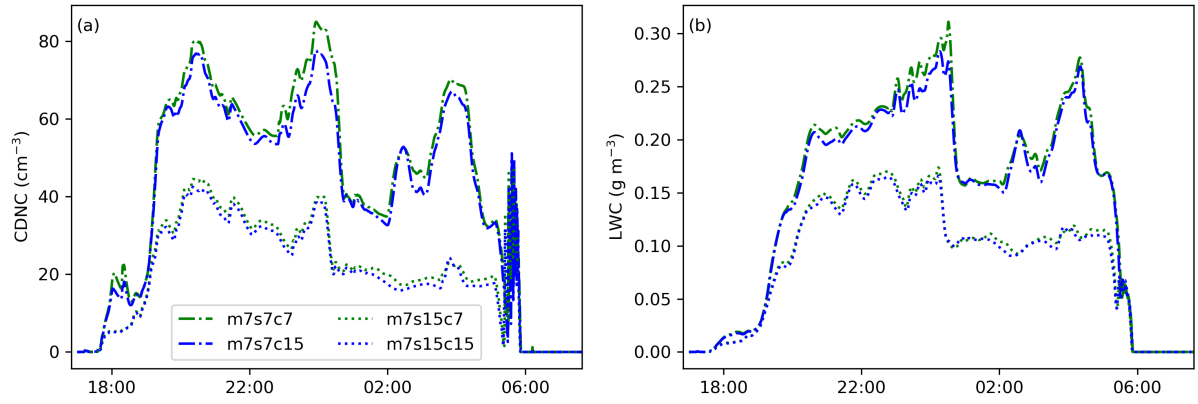
Figure S11. Sensitivity of LES code MIMICA to physicochemical aerosol properties. (a) cloud droplet number concentration (CDNC), (b) liquid water content (LWC) for different combinations of the dry aerosol number size distribution and \kappa , using the meteorology of fog event 7, as described in Fig. S10.
