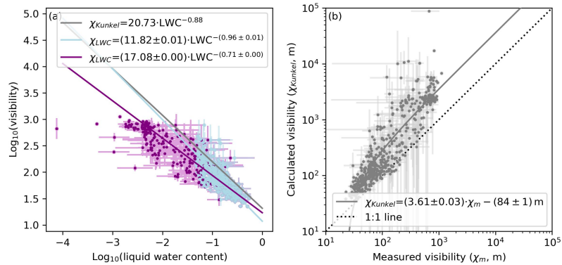
Figure S14. Visibility derived from LWC measurements with and without hydrated aerosol particles. (a) 10 min averages are shown for the visibility-only definition of fog (purple) and an additional liquid water content (LWC) threshold of 0.05 \text{ g m}^{-3} (lightblue). The visibility is calculated with a bivariate linear fit (following York et al., 2004) on the logarithm of the LWC. The parameterization by Kunkel (1984) is shown as gray line for comparison. (b) Derived visibility vs. measured visibility using the parameterization by Kunkel (1984).
