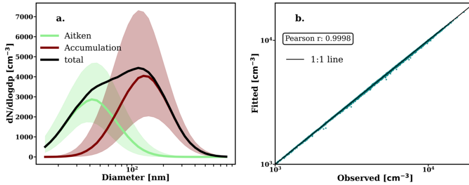
Figure S3. Separation of particle number size distribution into an Aitken and an accumulation mode. (a) median number size distributions for the Aitken (light green) and accumulation modes (red), as well as the total distribution (black). The shaded regions represent the interquartile range (25 th –75 th percentiles) for both modes. The log-normal size distributions were calculated from the fit parameters obtained after applying the algorithm by Hussein et al. (2005) on observed size distributions. (b) Scatter plot of the total particle concentration from fitting versus the total particle concentration from observation with a 1:1 line (black).
