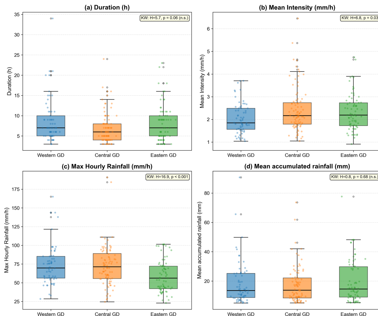
Figure 3. Statistical distributions of WSHR characteristics across three sub-regions: (a) event duration, (b) mean rainfall intensity, (c) maximum hourly rainfall, and (d) mean accumulated rainfall. The boxes show the median and interquartile range (IQR); whiskers extend to 1.5 \times \text{IQR} . The Kruskal–Wallis H statistic and the p -value are annotated in each panel.
