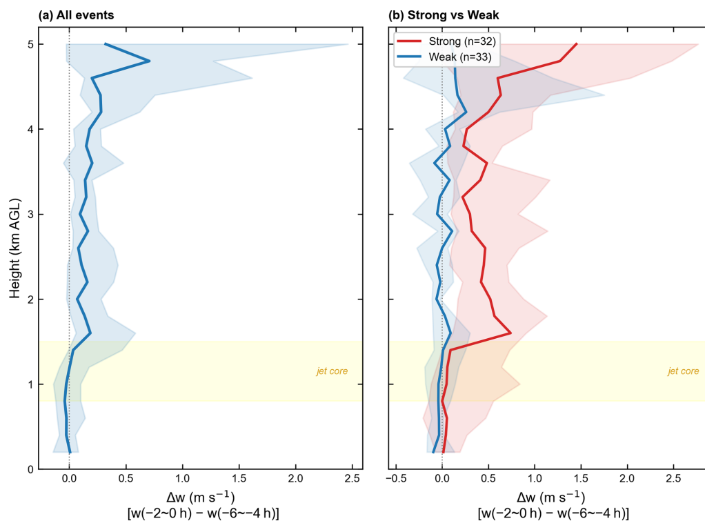
Figure 13. Vertical profiles of the pre-onset vertical velocity change ( \Delta w = \text{mean } w \text{ at } t = -2 \text{ to } 0 \text{ h} \text{ minus mean } w \text{ at } t = -6 \text{ to } -4 \text{ h} ) in western GD. (a) All events: solid line shows the composite median and shading shows the bootstrap 95 % confidence interval. (b) Strong-rainfall (red) and weak-rainfall (blue) events. The yellow band marks the jet core layer (0.8–1.5 km a.g.l.) identified from Fig. 11a.
