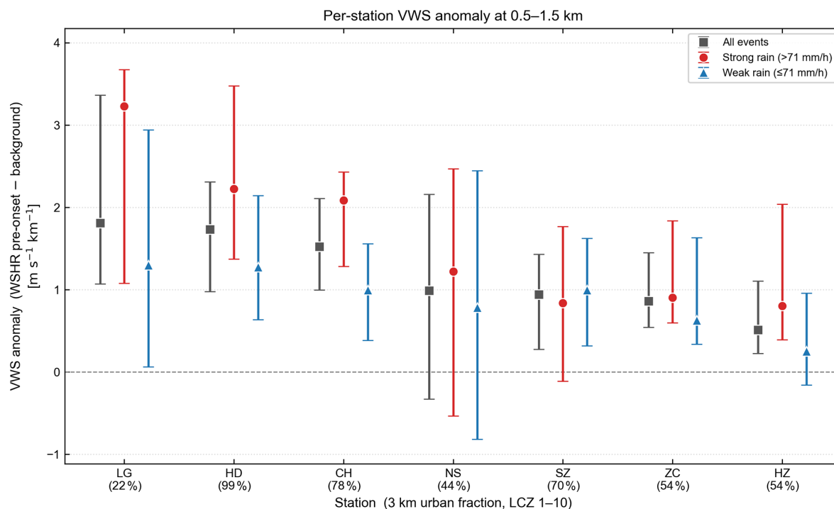
Figure 16. Per-station VWS anomaly composites at 0.5–1.5 km (3 h pre-onset mean) for the seven profiler stations in central GD, based on WSHR events during 2016–2020. Stations are ordered by the all-events median (grey squares); error bars denote bootstrap 95 % confidence intervals ( N = 2000 ). Red circles and blue triangles show medians for events with hourly peak rainfall above and below the 71 \text{ mm h}^{-1} split, respectively. x -axis labels include each station's 3 km urban fraction. Station codes: NS (Nansha), LG (Luogang), HD (Huadu), CH (Conghua), ZC (Zengcheng), SZ (Shenzhen), HZ (Huizhou Longmen).
