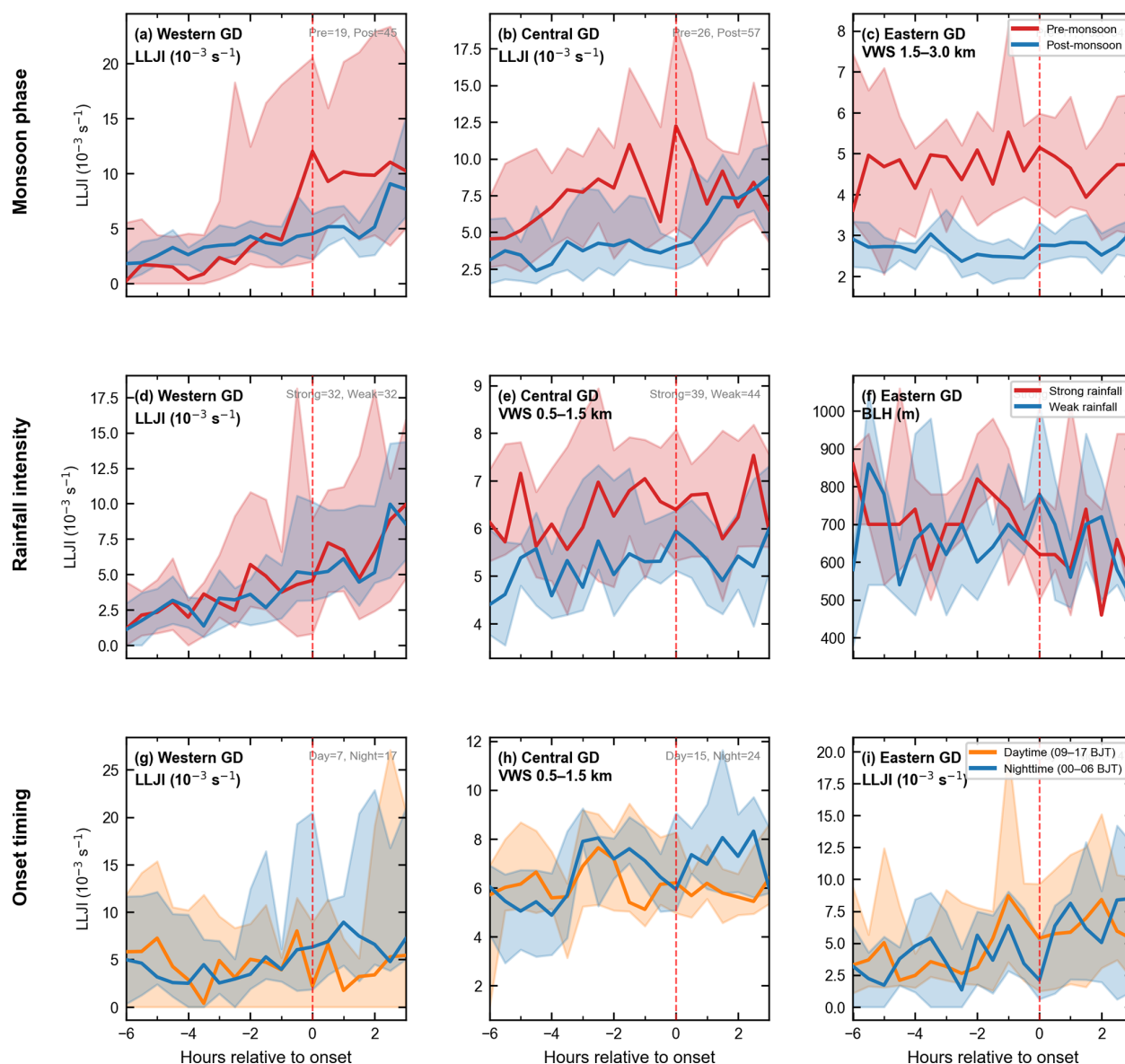
Figure 10. Stratified composite time series of selected precursor indices for the most physically interpretable index–stratification combinations (complete results in Figs. S1–S3 in the Supplement). Row 1 (a–c): pre-monsoon (red) versus post-monsoon (blue) for LLJI in western and central GD and VWS at 1.5–3.0 km in eastern GD. Row 2 (d–f): strong-rainfall (red) versus weak-rainfall (blue) events for LLJI in western GD, VWS at 0.5–1.5 km in central GD, and BLH in eastern GD. Row 3 (g–i): daytime versus nighttime onset events, where daytime and nighttime are defined following the onset-hour distributions in Sect. 3, for LLJI in western GD, VWS at 0.5–1.5 km in central GD, and LLJI in eastern GD. Lines show medians; shading shows the bootstrap 95 % CI. Event counts for each group are annotated.
