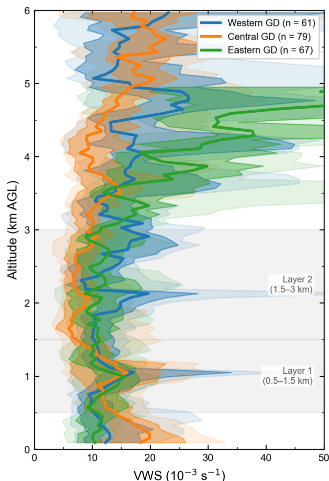
Figure 7. Composite VWS profiles averaged over t = -3 to 0 h for the western GD (blue, n = 61 ), central GD (orange, n = 79 ), and eastern GD (green, n = 67 ) regions. Lines show medians; dark and light shading show the 25–75 percentile range and 10th–90th percentile ranges. The gray bands mark the two layers used in Sect. 4.2: 0.5–1.5 km (Layer 1) and 1.5–3.0 km (Layer 2).
