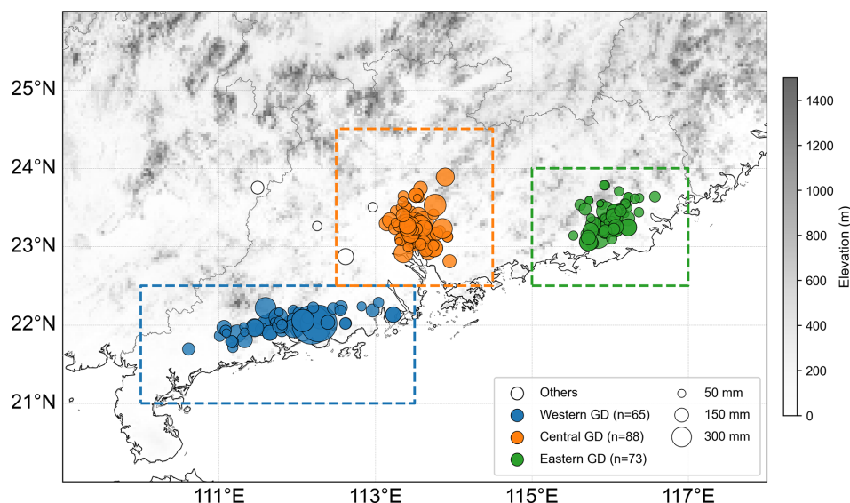
Figure 2. Spatial distribution of the WSHR precipitation centers in Guangdong Province during 2016–2020. The size of the marker is proportional to the maximum accumulated precipitation; white markers indicate invalid events. Dashed rectangles delineate the western (blue, n = 65 ), central (orange, n = 88 ), and eastern (green, n = 73 ) sub-regions. Gray shading shows the elevation of the terrain (m).
