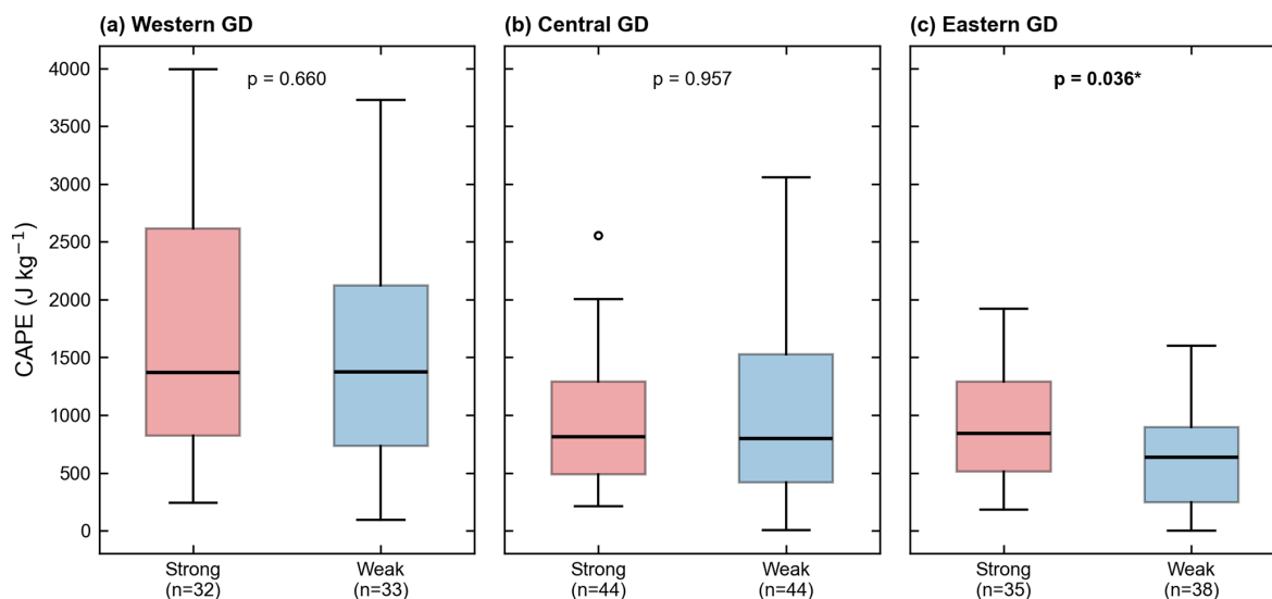
Figure 14. Pre-onset CAPE (ERA5, averaged over t = -6 \text{ to } -2 \text{ h} ) for strong-rainfall (red) and weak-rainfall (blue) events in (a) western GD, (b) central GD, and (c) eastern GD. The box plots show the median, interquartile range, and whiskers extending to 1.5 \times \text{IQR} . The p value of the Mann-Whitney U -test is annotated; an asterisk denotes p < 0.05 .
