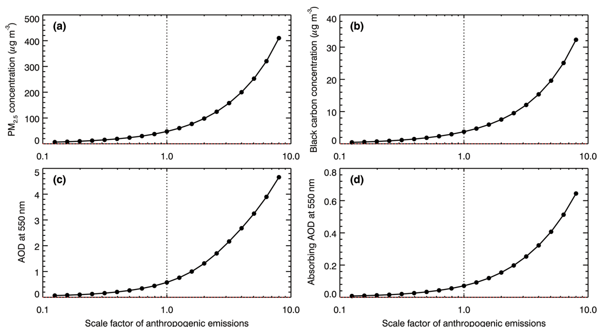
Figure 6. Average (a) near-surface \text{PM}_{2.5} , (b) black carbon mass concentration, (c) AOD at 550 nm, and (d) absorbing AOD at 550 nm in GZB + GZBs from 26 to 28 January 2022, as a function of the scale factor of anthropogenic emissions.
