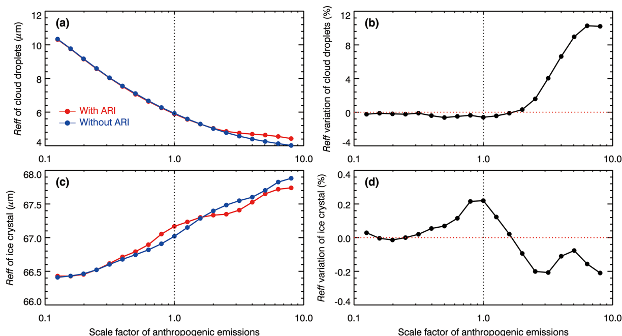
Figure 10. (a) p -mean of R_{\text{effc}} , (b) variation of p -mean of R_{\text{effc}} due to ARIs, (c) p -mean of R_{\text{effi}} , and (d) variation of p -mean of R_{\text{effi}} due to ARIs over GZB + GZBs from 26 to 28 January 2022, as a function of the scale factor of anthropogenic emissions.
