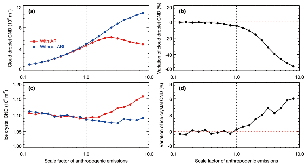
Figure 8. Average (a) cloud droplet CND, (b) variation of cloud droplet CND due to ARIs, (c) ice crystal CND, and (d) variation of ice crystal CND due to ARIs over GZB + GZBs from 26 to 28 January 2022, as a function of the scale factor of anthropogenic emissions.
