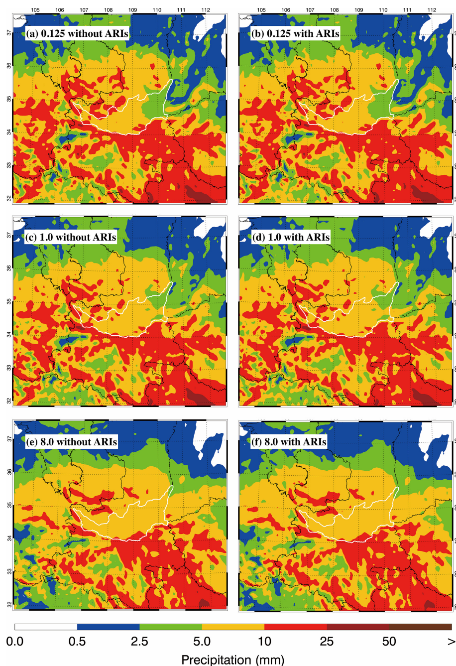
Figure 14. Distribution of accumulative precipitation from 26 to 28 January 2022 for various scale factor of anthropogenic emissions when ARIs are (a, c, e) excluded and (b, d, f) included. The white contour outlines the GZB. The white contour outlines the GZB and the area outside of GZB in panels is referred to as GZBs.
