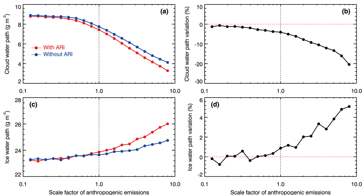
Figure 9. Average (a) CWP, (b) variation of CWP due to ARIs, (c) IWP, and (d) variation of IWP due to ARIs over GZB + GZBs from 26 to 28 January 2022, as a function of the scale factor of anthropogenic emissions.
