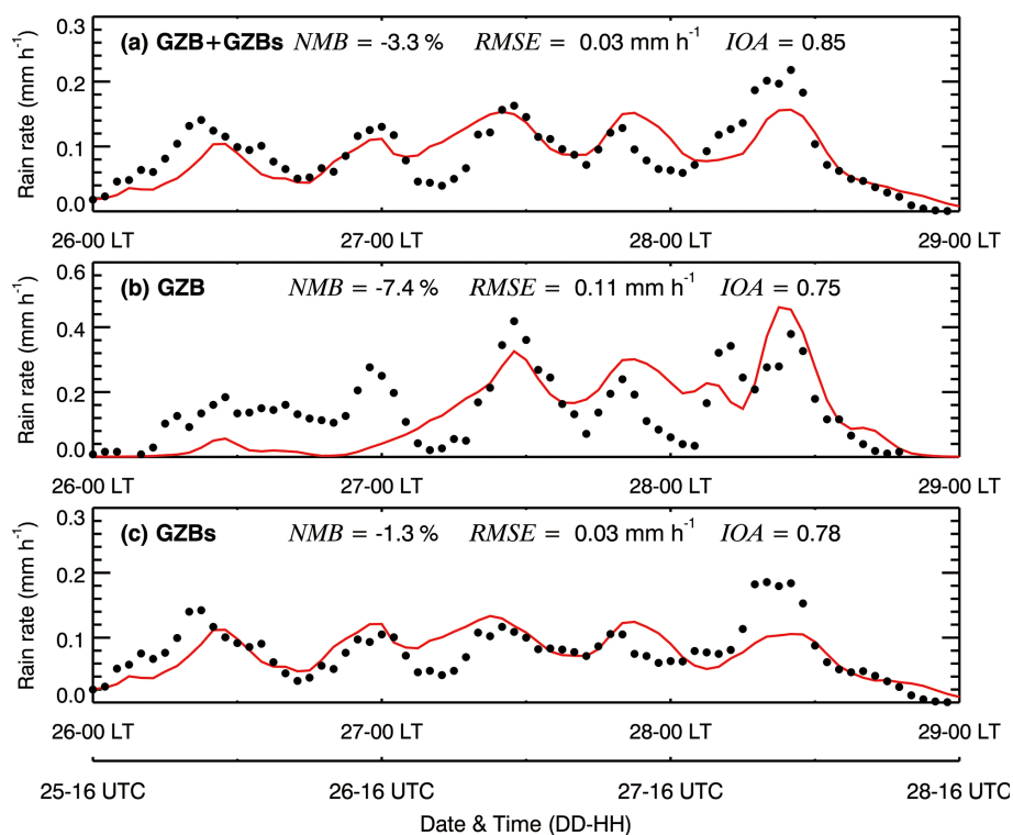
Figure 4. Comparison of observed (black dots) and simulated (solid red lines) diurnal profile of hourly rain rate averaged at monitoring sites in (a) GZB + GZBs, (b) GZB, and (c) GZBs from 26 to 28 January 2022.
