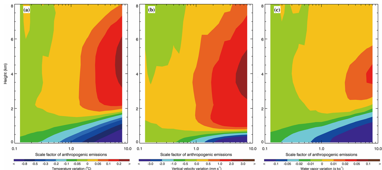
Figure 7. Profile variation of average (a) air temperature, (b) vertical velocity, and (c) water vapor over GZB + GZBs from 26 to 28 January 2022 caused by ARIs, as a function of the scale factor of anthropogenic emissions.
