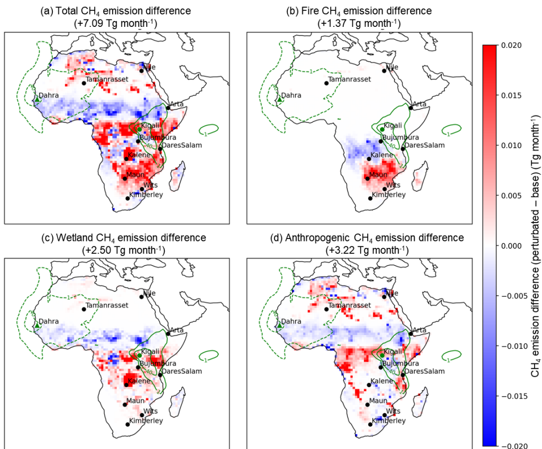
Figure S11. Spatial differences in July CH 4 prior emissions between the perturbed prior and the base prior over Africa. Panels show (a) total, (b) fire, (c) wetland, and (d) anthropogenic CH 4 . Colors denote the grid-cell emission difference (perturbed-base). Black markers indicate optimal selected sites common to both priors, green circles indicate sites included only in base prior (Kigali), and green triangles indicate sites included only in perturbed prior test (Dahra). Green contour lines overlay the 3-day footprints for sites unique to each condition (solid for base prior; dashed for perturbed prior test), with numbers denoting the corresponding footprint values.
