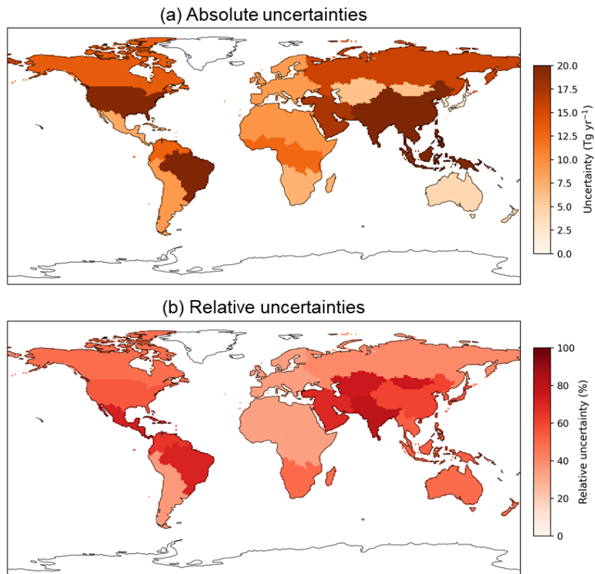
Figure S1. Regional annual prior uncertainty budget for CH 4 emissions derived from the prior error covariance matrix \mathbf{B} used in this study. The uncertainty for each region is calculated as \sigma^2 = \mathbf{l}^T \mathbf{B} \mathbf{l} , where \mathbf{l} represents the vector converting grid-scale emissions into regional totals. The upper panel shows the absolute annual uncertainty (Tg yr -1 ), and the lower panel shows the corresponding relative uncertainty (%), defined as the ratio of the uncertainty to the regional annual prior emissions.
