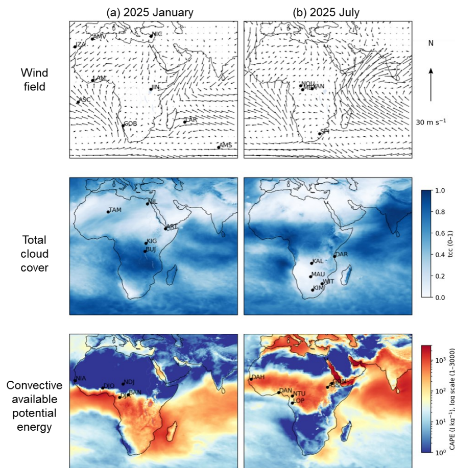
Figure S7. Meteorological conditions over Africa in January (left column) and July (right column) 2025. The top row shows 10-m wind fields, the middle row presents total cloud cover (TCC), and the bottom row displays convective available potential energy (CAPE). Black dots indicate 34 sites listed in Table S2, with their first three letters for clarity here. Data are from ERA5 dataset ( https://cds.climate.copernicus.eu/datasets ).
