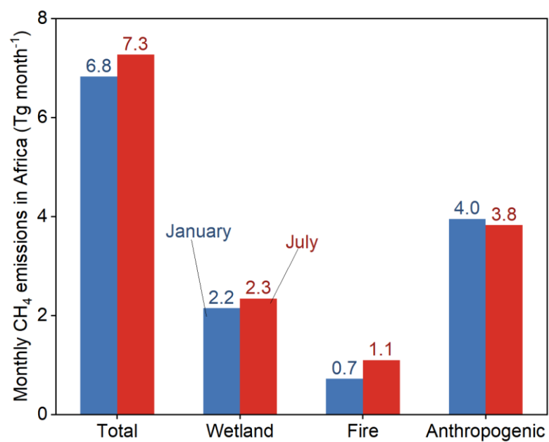
Figure S4. Comparison of African CH 4 emissions across sectors between January and July in 2023.
