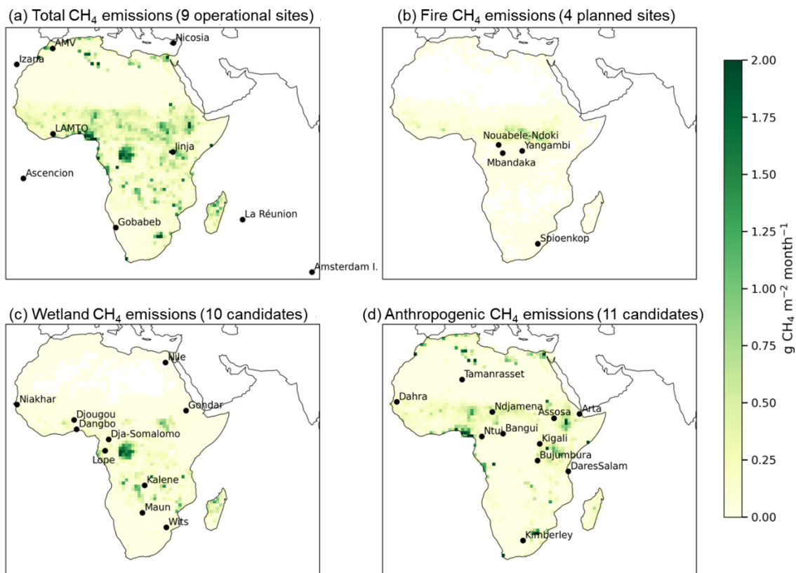
Figure S3. Sectoral CH 4 emissions and observation coverage over Africa in January. (a) total CH 4 emissions with current 9 operational sites (La Réunion, Nicosia, Ascension, Izaña, LAMTO, AMV, Gobabeb, Jinja, Amsterdam Island); (b) fire CH 4 emissions with 4 planned observation sites (Yangambi, Mbandaka, Nouabele-Ndoki, Spienkop); (c) wetland CH 4 emissions with 10 candidate sites (Dja-Somalomo, Wits, Niakhar, Nile, Djougou, Dangbo, Kalene, Gondar, Lope, Maun); and (d) anthropogenic CH 4 emissions with the remaining 11 candidate sites (Dahra, Ntui, Kigali, Bujumbura, Arta, Assosa, Bangui, Kimberley, Tamanrasset, Ndjamen, DaresSalam).
