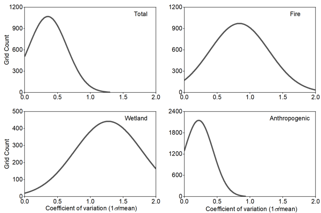
Figure S5. The coefficient of variation for sectoral CH 4 prior emissions adopted in this study.
