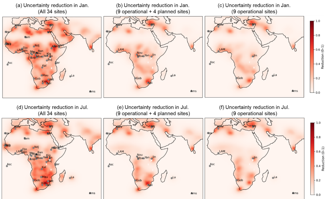
Figure S6. Spatial distribution of uncertainty reduction for total CH 4 emissions under different site deployments and months.
