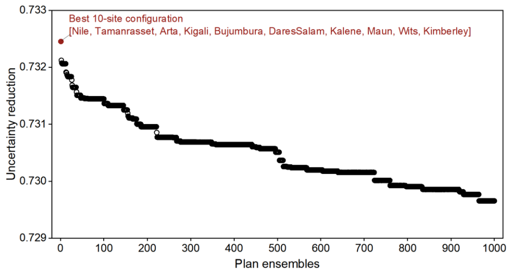
Figure S10. The best site configuration selection among 10-site plans (top 1000 plans are plotted).
