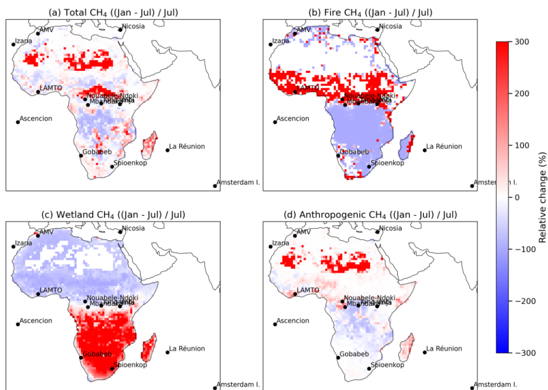
Figure S8. Spatial difference between January and July for (a) total; (b) fire; (c) wetland; and (d) anthropogenic CH 4 emissions. Here presents the relative difference calculated as (January - July)/July. Dots denote 9 operational and 4 planned sites.
