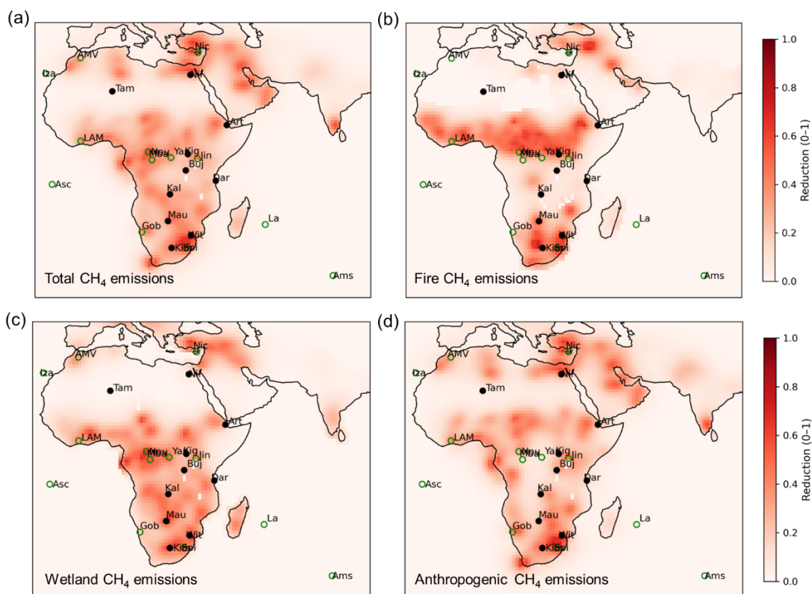
Figure S9. Spatial distribution of uncertainty reduction for (a) total; (b) fire; (c) wetland; and (d) anthropogenic CH 4 emissions with the 10 optimal sites configuration in 2025 January. The 10 optimal sites in this case include Nile, Tamanrasset, Arta, Kigali, Bujumbura, DaresSalam, Kalene, Maun, Wits, and Kimberley. All the site names are abbreviated with first three letters. The green open circles are 9 operational and 4 planned sites, and the closed black circles are optimized new 10 sites.
