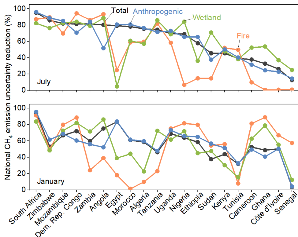
Figure S13. Country-specific CH 4 emission uncertainty reduction with the 10 optimal site configurations. Only 20 countries are presented here for clarity, with more country results listed in Table S5.
