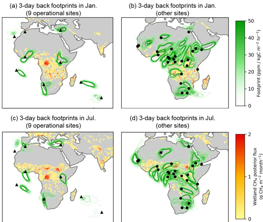
Figure S2. Spatial distribution of 3-day backward transport footprints over Africa for January (top row) and July (bottom row). (a) and (c) show footprints associated with the 9 operational sites, while (b) and (d) correspond to other 25 sites. Green contours represent footprint sensitivities ( \text{ppm kgC m}^{-2} \text{ hr}^{-1} ), indicating the influence of surface methane emissions on the column observations. The background shows wetland \text{CH}_4 emissions ( \text{g CH}_4 \text{ m}^{-2} \text{ month}^{-1} ), emissions less than 0.05 \text{ g CH}_4 \text{ m}^{-2} \text{ month}^{-1} are gray-shaded for clarity. Black dots (triangles and circles) denote the locations of surface observation sites.
