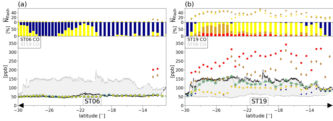
Figure S1: Simulated and observed CO mixing ratios. Equivalent to Fig. 04.
