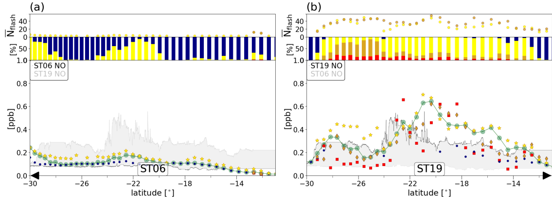
Figure S2: Simulated and observed NO mixing ratios. Equivalent to Fig. 04.
