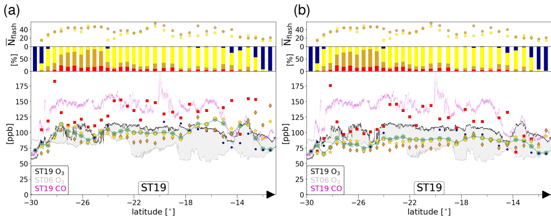
Figure S3: Simulated and observed O_3 mixing ratios for the experiments CAPE_{high} (a) and EMAC_{noBB} (b).
