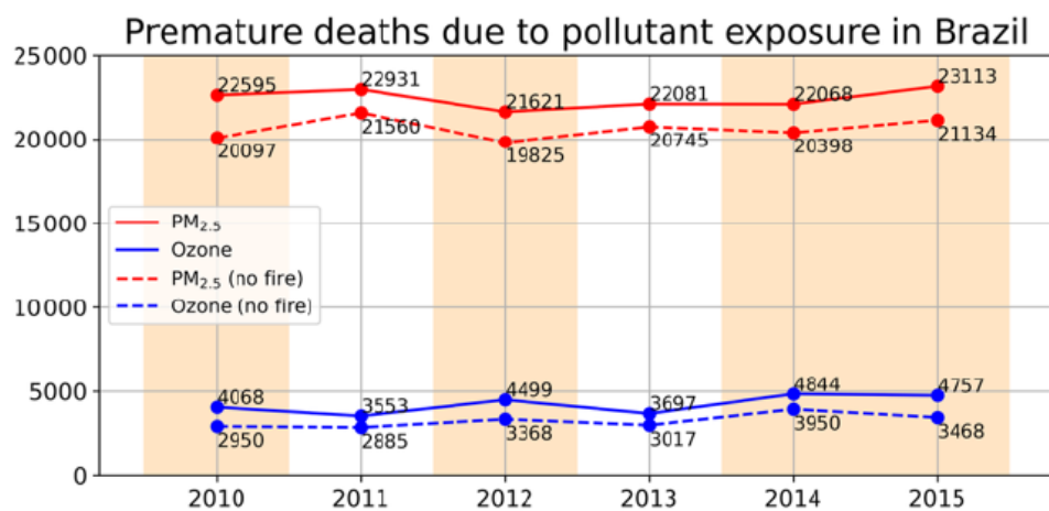
Figure 7. Timeseries of annual excess mortalities due to exposure to PM 2.5 (red) and ozone (blue) in “fire-on” (solid line) and “fire-off” (dotted line) simulations. Shaded area indicated years with more than 3 months which 20th percentile of regional SPEI index smaller than -1.5 .
