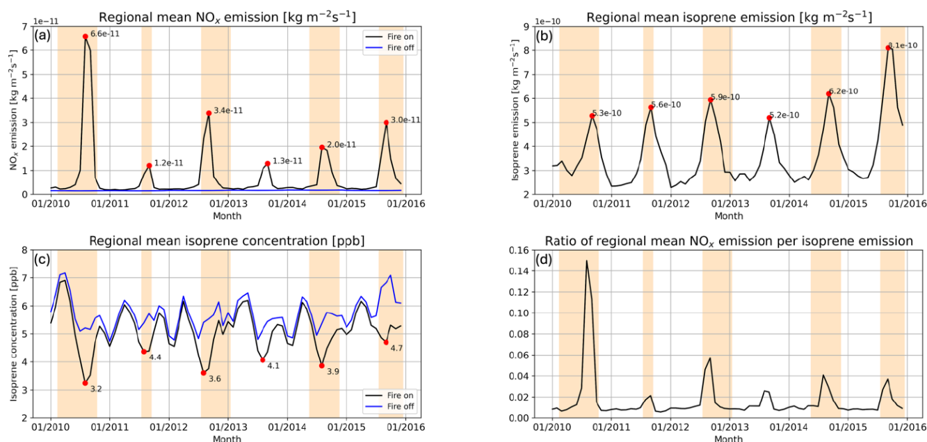
Figure 4. Simulated monthly mean (a) nitrogen oxide (NO x ) emission, (b) isoprene emission and (c) isoprene concentration from January 2010–December 2015 in Brazilian Amazon. (d) Time series of NO x and isoprene emission ratio from 2010–2015. Red dots are the annual peak (low) and shaded area indicated dry months where 20th percentile of regional SPEI index smaller than -1.5 .
