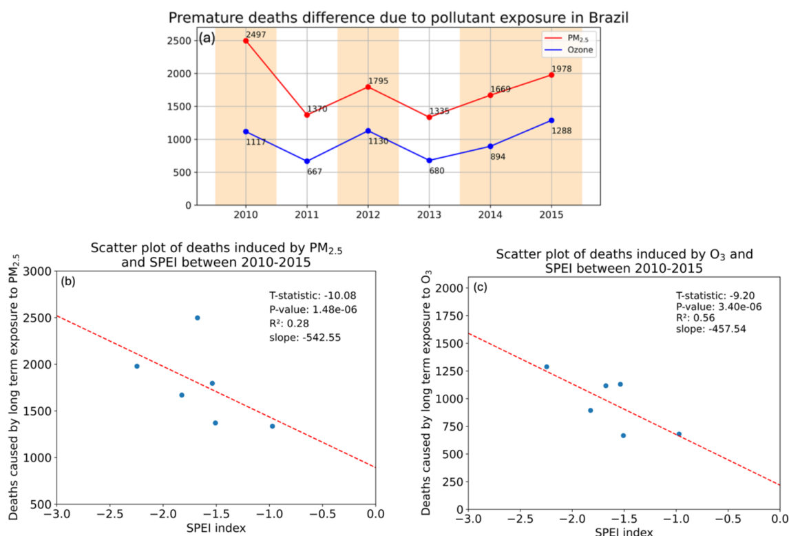
Figure 9. (a) Fire-induced premature mortalities due to exposure to PM 2.5 (red) and ozone (blue). Shaded area indicated years with more than 3 months which 20th percentile of regional SPEI index smaller than -1.5 . Scatter plots between SPEI drought index and fire-induced premature mortalities due to exposure to (b) PM 2.5 and (c) ozone.
