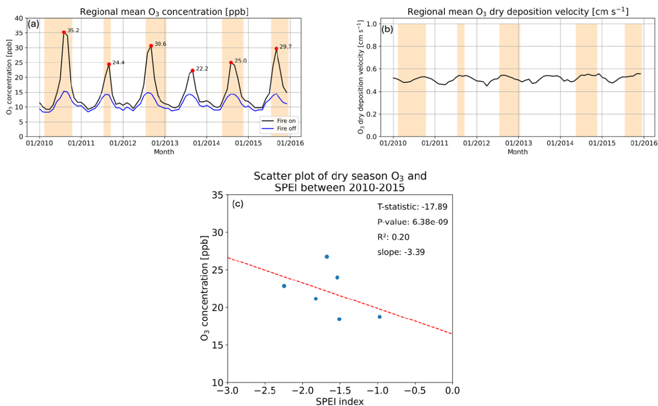
Figure 5. (a) Simulated monthly mean ozone concentration and (b) dry deposition from January 2010–December 2015 in Brazilian Amazon. Shaded area indicated dry months where 20th percentile of regional SPEI index smaller than -1.5 . (c) Scatter plot of dry season regional mean ozone and the dry season mean SPEI index.
