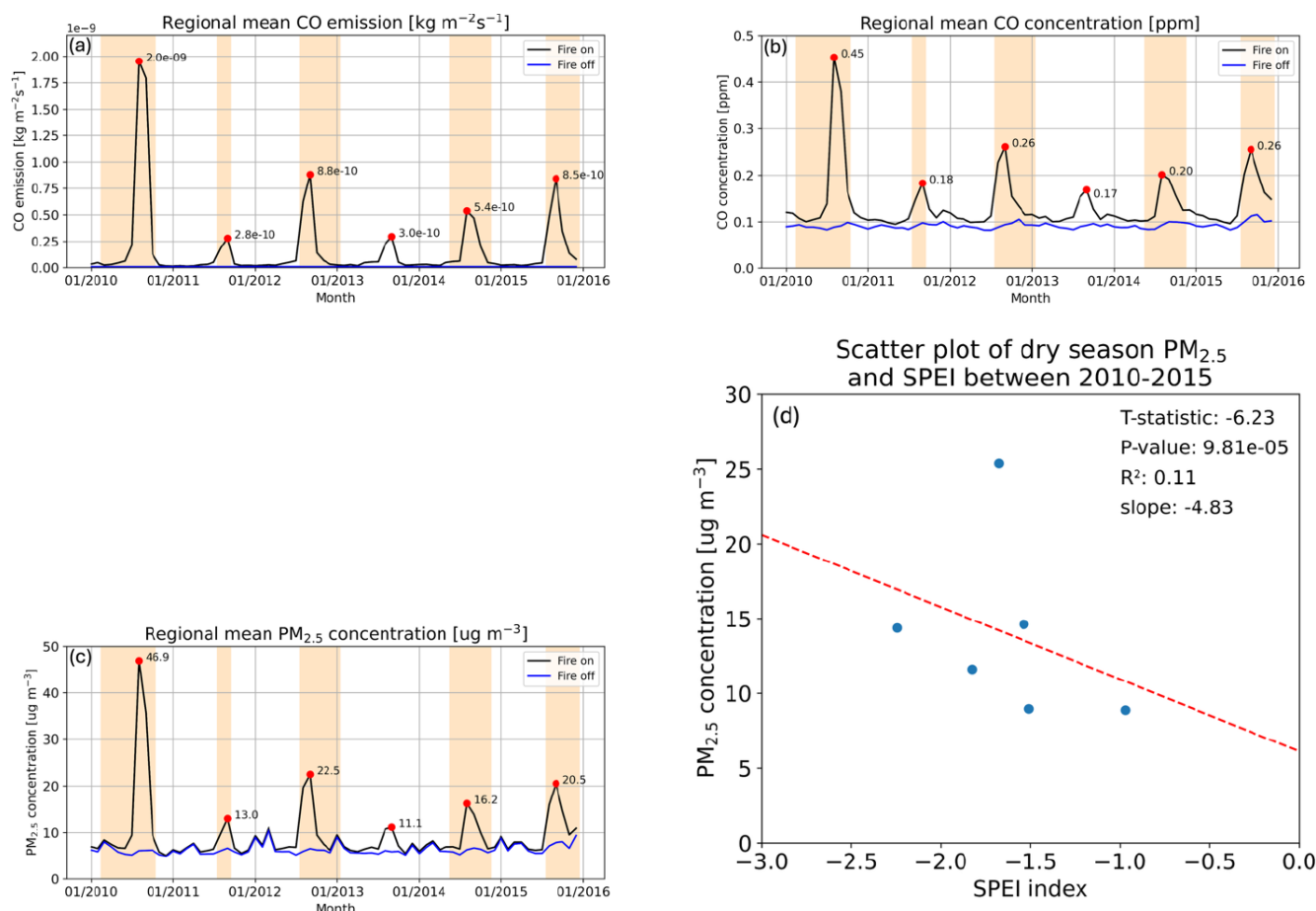
Figure 2. Simulated monthly mean carbon monoxide (CO) (a) emission, (b) concentrations and (c) \text{PM}_{2.5} concentrations from January 2010–December 2015 in Brazilian Amazon. Red dots are the annual peak and the shaded area indicated dry months where 20th percentile of regional SPEI index smaller than -1.5 . (d) Scatter plot of dry season regional mean \text{PM}_{2.5} and the dry season mean SPEI index.
