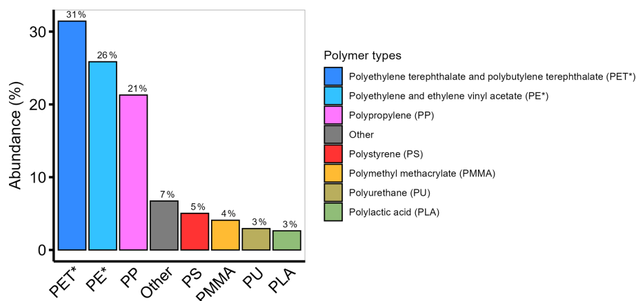
Figure 3. Percentage of different polymer types comprising the microplastic particles ( n = 7150 ) detected in wet and dry deposition collected between May 2024 and May 2025 in Zurich (urban), Duebendorf (suburban), Magadino (rural), Payerne (rural) and Chaumont (mountainous), Switzerland. The polymer type “other” includes polyacrylonitrile, silicone, polyvinyl chloride, acrylonitrile butadiene styrene, ethylene vinyl alcohol, polyoxymethylene and polyether ether ketone.
