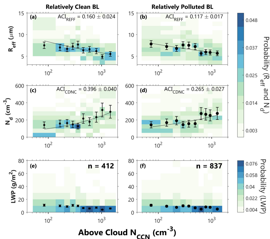
Figure 8. Results of from CE data set ( n = 1249 ) show the relationship between above-cloud N_{CCN} and (a–b) R_{eff} , (c–d) N_d , and (e–f) LWP for cases with a relatively clean BL (below-cloud N_{CCN} \leq 350 \text{ cm}^{-3} ) and a relatively polluted BL (below-cloud N_{CCN} > 350 \text{ cm}^{-3} ). The shading, scatter points, ACI metrics, and fit lines are calculated and displayed in the same way as Fig. 4.
