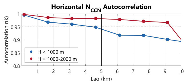
Figure 1. The autocorrelation coefficient of in situ N_{\text{CCN}} observed in horizontal flight legs is given as a function of lag distance. The dark blue line represents observations from flight legs at altitudes ( H ) < 1000 m, and the red line represents observations from flight legs between H = 1000 –2000 m. The black dashed line depicts an autocorrelation coefficient of 0.95, and the solid vertical line depicts the 5 km over which we assume that below-cloud N_{\text{CCN}} is approximately constant.
