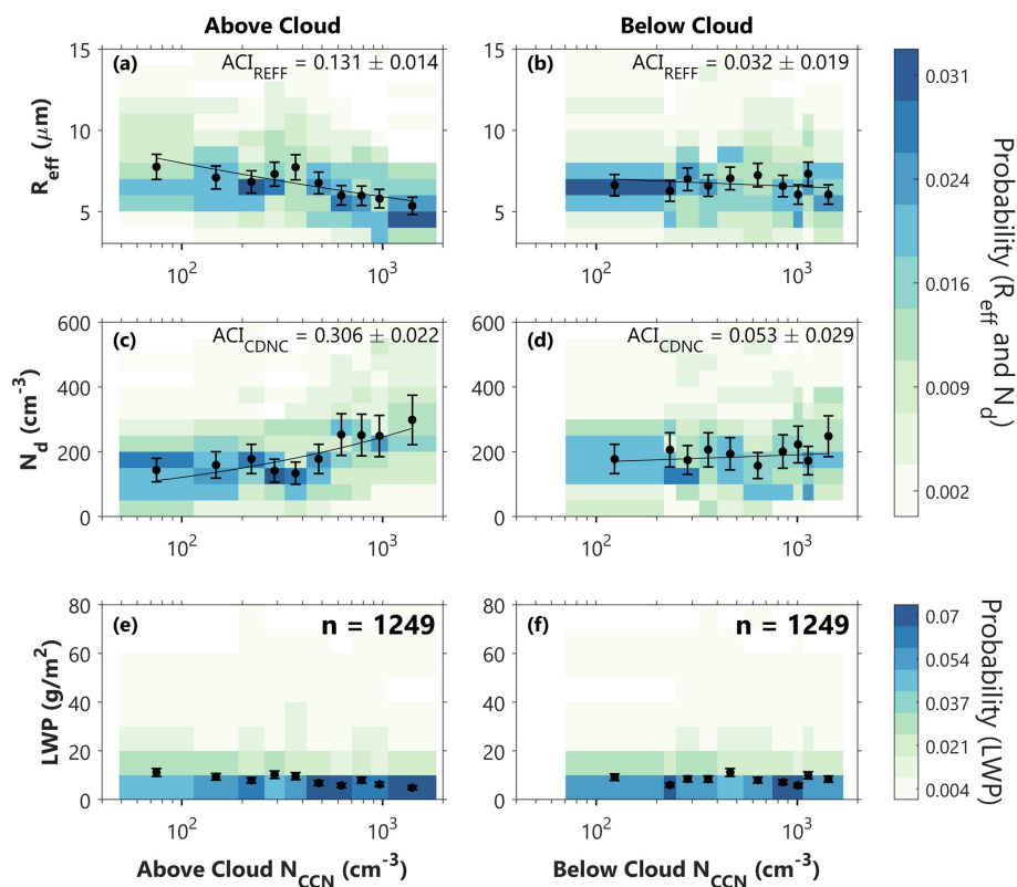
Figure 7. Results of from CE data set ( n = 1249 ) show the relationship between (a, c, e) above- and (b, d, f) below-cloud N_{\text{CCN}} and (a–b) R_{\text{eff}} , (c–d) N_d , and (e–f) LWP. The shading, scatter points, ACI metrics, and fit lines are calculated and displayed in the same way as Fig. 4.
