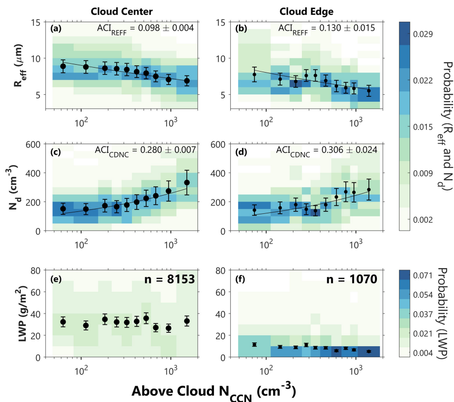
Figure 11. Results from cloud center and CE data sets show the relationship between above-cloud N_{\text{CCN}} and (a–b) R_{\text{eff}} , (c–d) N_d , and (e–f) LWP. The shading, scatter points, ACI metrics, and fit lines are calculated and displayed in the same way as Fig. 4.
