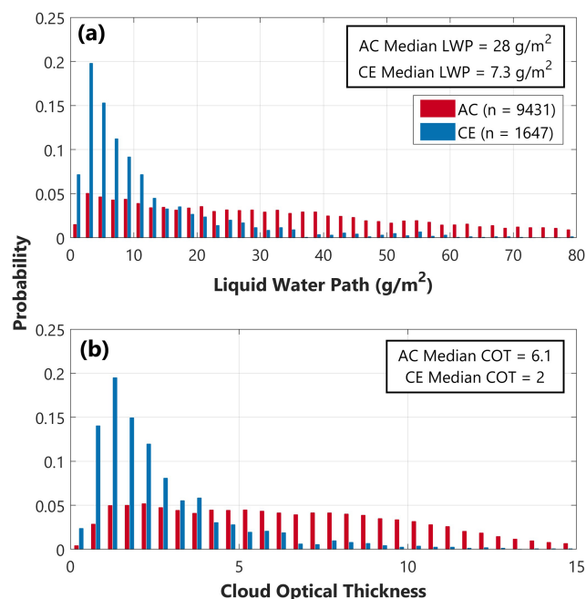
Figure 10. Distributions of (a) LWP and (b) COT for all AC data points (red) and CE data points (blue). Median values for both variables and both subsets of data are also shown.
