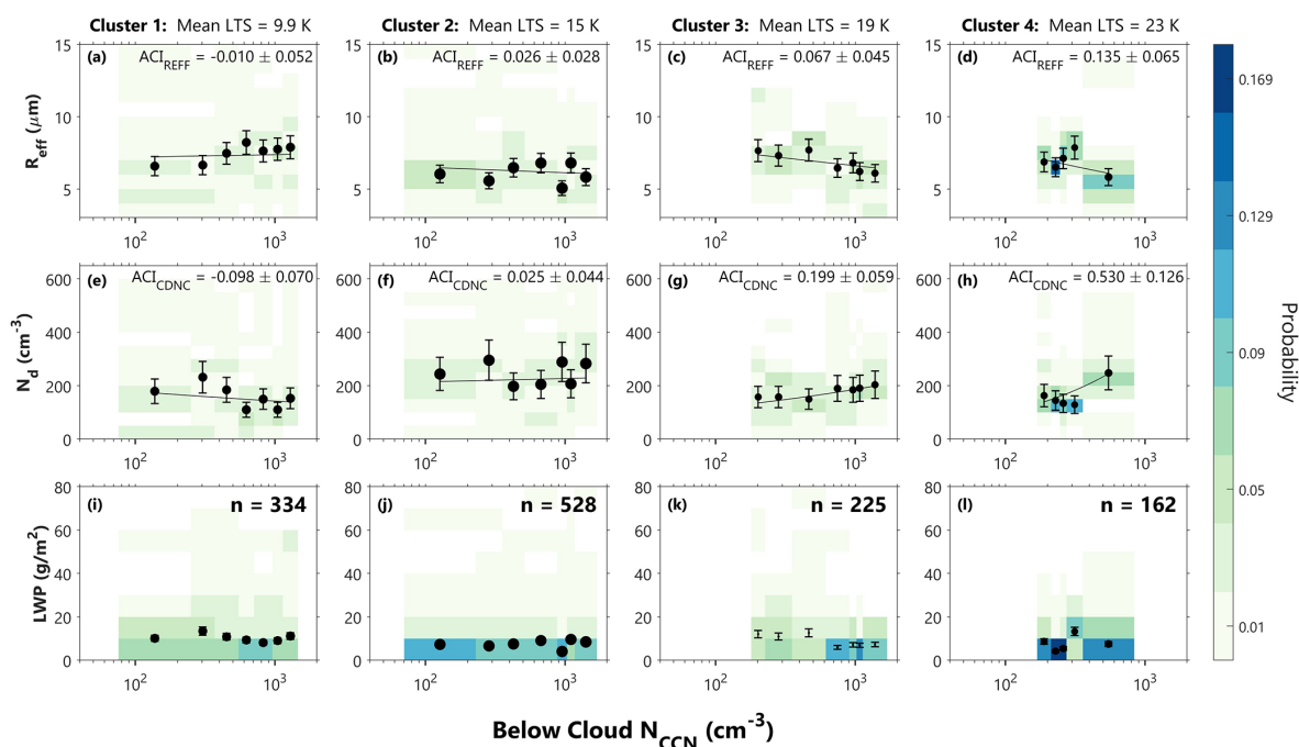
Figure 9. Below-cloud observations from Fig. 7 are assigned to clusters determined in Fig. 5. Results of this clustering show the relationship between below-cloud N_{\text{CCN}} and (a–d) R_{\text{eff}} , (e–h) N_d , and (i–l) LWP. Average LTS in each cluster increases from left to right. The shading, scatter points, ACI metrics, and fit lines are calculated and displayed in the same way as Fig. 4.
