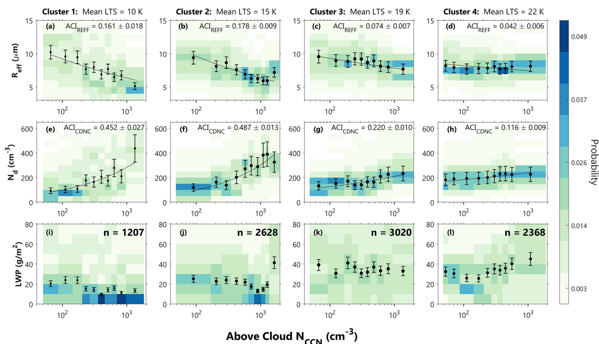
Figure 5. Relationship between above-cloud N_{\text{CCN}} and (a–d) R_{\text{eff}} , (e–h) N_d , and (i–l) LWP across LTS clusters determined using k -means clustering. The shading, scatter points, ACI metrics, and fit lines are calculated and displayed in the same way as Fig. 4.
