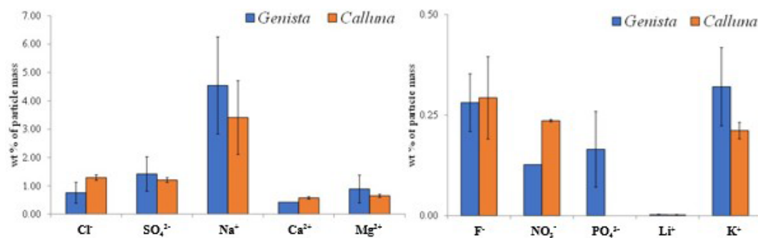
Figure 3. Water-soluble ions, expressed as wt % (mass fraction of the species times 100 of particle mass), in Calluna and Genista burnings.
