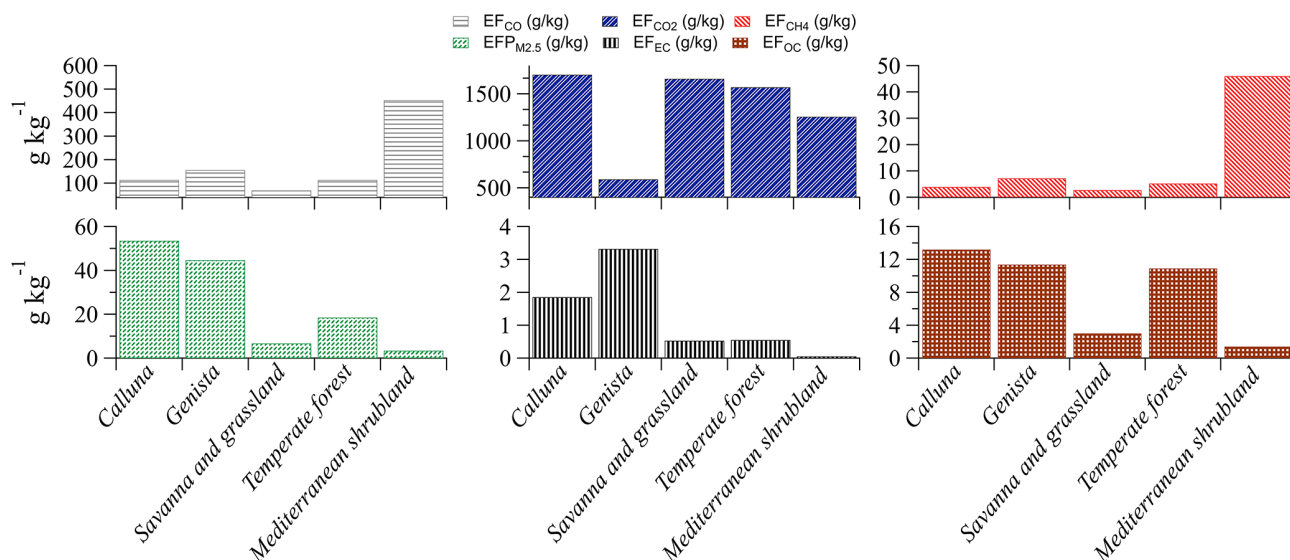
Figure 2. Comparison of emission factors (EF) for \text{CO} , \text{CO}_2 , \text{CH}_4 , \text{PM}_{2.5} , organic carbon (OC) and elemental carbon (EC) during Calluna and Genista prescribed fires with Mediterranean shrubland wildfire values from Garcia-Hurtado et al. (2013) and literature-average values for savannas/grasslands and temperate forests (Andreae, 2019). The Andreae (2019) values are compiled averages from multiple biomass-burning studies and represent a mixture of fire types and measurement conditions, including field and laboratory burns.
