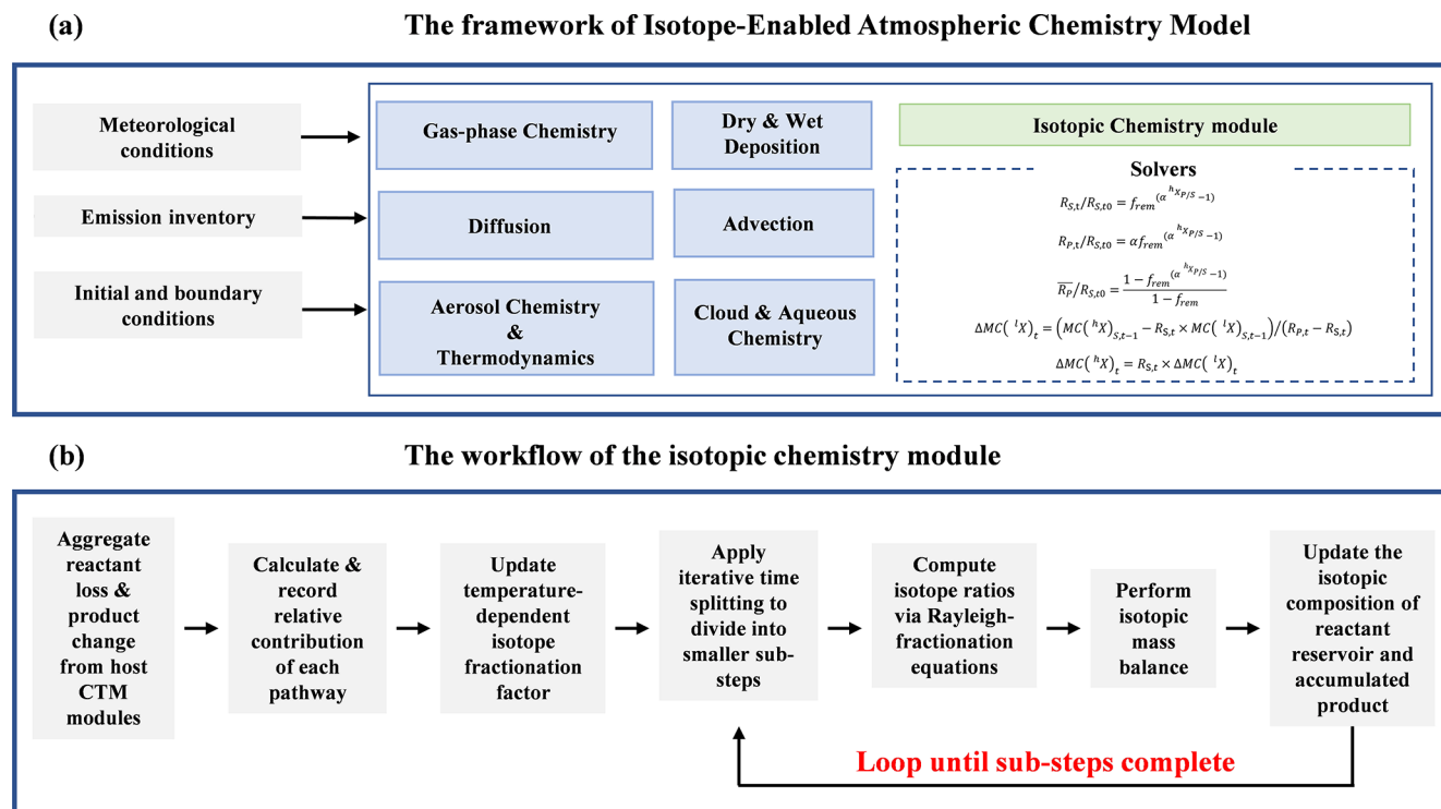
Figure 2. Algorithmic framework of the isotope-enabled CTM and the isotopic chemistry module. (a) Host CTM framework, including the main physical and chemical modules (gas-phase chemistry, aerosol chemistry and thermodynamics, cloud and aqueous chemistry, advection, diffusion, and dry and wet deposition) and their coupling with the isotopic chemistry module. (b) The workflow of the isotopic chemistry module. At each time step, the module tracks net SO 2 and sulfate changes, calculates reaction fractions, updates temperature-dependent fractionation factors, applies iterative time splitting, computes isotope ratios via Rayleigh-fractionation equations, performs isotopic mass balance, and updates the isotope ratios of the reactant reservoir and accumulated product.
