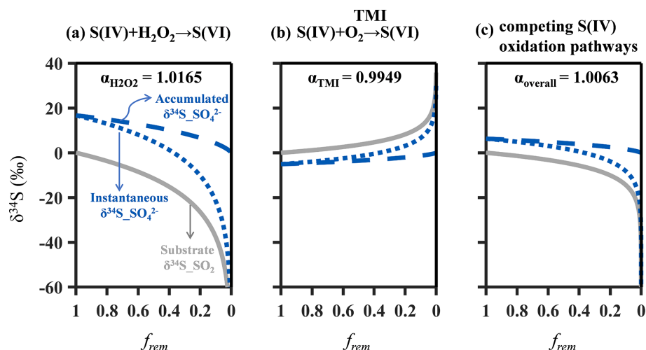
Figure 3. Rayleigh plot for sulfur isotope fractionations during SO 2 oxidation in a closed system with no external input and irreversible product removal. \delta^{34}\text{S} values of the residual reactant (solid black line), instantaneous product (blue dotted line), and accumulated product (blue dashed line) are shown as a function of the fraction of remaining reactant based on a Rayleigh equation, with the initial \delta^{34}\text{S} of SO 2 set to 0‰. Three scenarios are illustrated: (a) aqueous-phase H 2 O 2 oxidation ( \alpha^{34}\text{S} = 1.0165 at 0 °C), (b) aqueous-phase TMI-catalyzed oxidation ( \alpha^{34}\text{S} = 0.9949 at 0 °C), and (c) the net isotope effect under competing S(IV) oxidation pathways ( \alpha^{34}\text{S} = 1.0063 at 0 °C). The pathway contributions in panel (c) competing S(IV) oxidation pathways – gas-phase OH oxidation (42.6 %), aqueous H 2 O 2 oxidation (2.2 %), O 3 oxidation (1.3 %), TMI-catalyzed oxidation (27.2 %), and heterogeneous reactions (26.7 %) – are derived from GEOS-Chem simulations (Shao et al., 2019).
