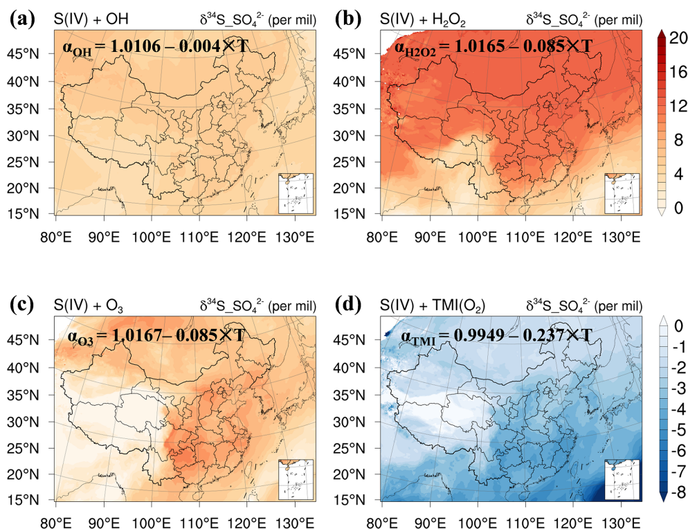
Figure 5. Same as Fig. 4, but for near-surface \delta^{34}\text{S}_{\text{SO}_4^{2-}} . Panels show sensitivity experiments with individual oxidation pathways active: (a) gas-phase OH, (b) aqueous-phase \text{H}_2\text{O}_2 , (c) aqueous-phase \text{O}_3 , and (d) TMI-catalyzed \text{O}_2 oxidation, all for December 2015 with \delta^{34}\text{S}_{\text{SO}_2} emission = 0‰. Positive values indicate ^{34}\text{S} enrichment in sulfate; negative values indicate depletion.
