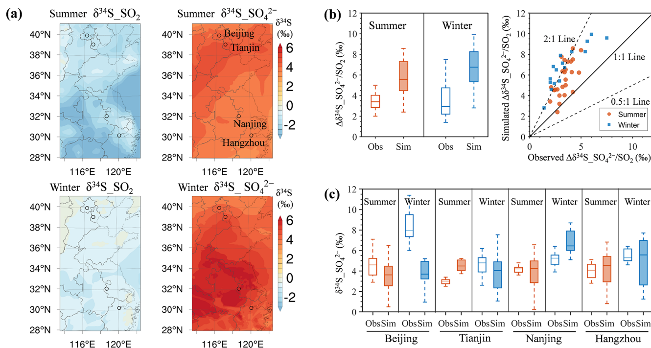
Figure 6. Comparison between simulated and observed sulfur isotope composition over eastern China. (a) Simulated seasonal mean spatial distributions of sulfur isotopic composition ( \delta^{34}\text{S}_{\text{SO}_2} , \delta^{34}\text{S}_{\text{SO}_4^{2-}} ) over eastern China for summer (June–August) and winter (December–February) of 2015. (b) Comparison of simulated and observed \delta^{34}\text{S}_{\text{SO}_2} , \delta^{34}\text{S}_{\text{SO}_4^{2-}} , and \Delta\delta^{34}\text{S}_{\text{SO}_4^{2-}}/\text{SO}_2 at Nanjing during the summer and winter 2014. \Delta\delta^{34}\text{S}_{\text{SO}_4^{2-}}/\text{SO}_2 primarily reflects oxidation-induced isotope fractionation and is less sensitive to the assumed \delta^{34}\text{S} of emission sources, providing a more direct evaluation of the oxidation isotope module. (c) Seasonal comparison of simulated and observed \delta^{34}\text{S}_{\text{SO}_4^{2-}} in \text{PM}_{2.5} across multiple cities in eastern China, simulated values correspond to the same seasonal periods as the observations at each site. In panels (b) and (c) , “Obs” denotes observation and “Sim” denotes simulation.
