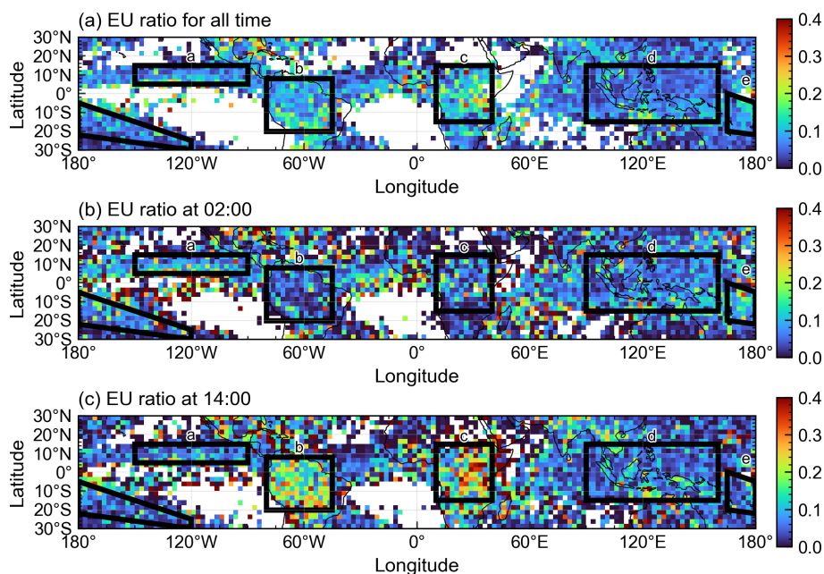
Figure 8. Spatial distribution of the occurrence of extreme-updraft (EU) columns. (a) Fraction of EU candidate columns (folded-column) relative to all convective columns in each grid box. (b, c) Same as (a) , but separated by local overpass time: (b) late night ( \sim 02:00 LT; ascending node) and (c) early afternoon ( \sim 14:00 LT; descending node). Grid boxes with fewer than 100 total columns are masked in (a)–(c) . Black rectangles labeled a–e indicate the regions used for the regional analyses (EPAC–ITCZ, Amazon, central Africa, Maritime Continent, and SPCZ).
