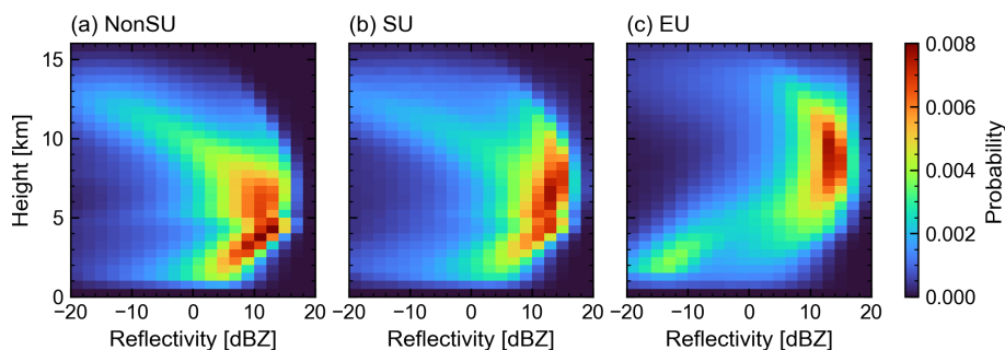
Figure 3. Normalized contoured frequency-by-altitude diagrams (CFADs) of EarthCARE/CPR radar reflectivity (Ref; dBZ) for (a) non-strong-updraft (NonSU) columns, (b) strong-updraft (SU) columns, and (c) extreme-updraft (EU) candidate columns. Reflectivity is binned in 2 dB intervals, and the vertical coordinate is binned in 500 m intervals. Each panel is normalized by its total number of height–reflectivity samples such that the color indicates probability (i.e., the sum over all bins in each panel equals 1).
