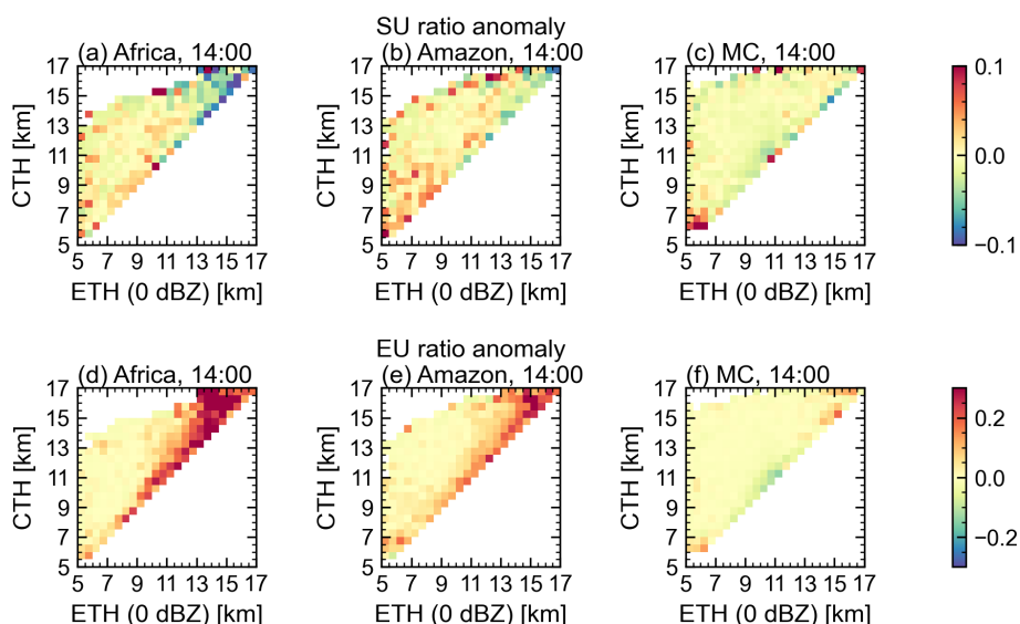
Figure 10. Deviations in Doppler-based occurrence ratios conditioned on cloud-top height (CTH) and the 0 dBZ echo-top height [ETH(0)] for early afternoon ( \sim 14:00 LT). Panels (a)–(c) show deviations in the \text{Max } V_d -based SU ratio, and (d)–(f) show deviations in the Doppler-velocity folded-column ratio, for (a, d) central Africa, (b, e) the Amazon, and (c, f) the Maritime Continent. Bin size is 0.5 km in both dimensions; only bins with N \geq 100 columns are shown.
