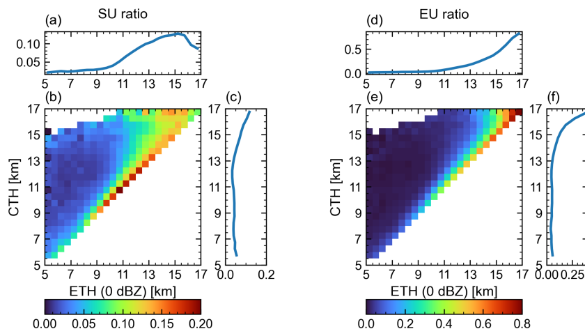
Figure 6. Occurrence ratios of SU columns and EU columns as functions of ETH(0) and CTH. (a–c) SU ratio and (d–f) EU ratio. The SU ratio is defined as the number of non-folded columns with \text{Max} V_d > 2.0 \text{ m s}^{-1} divided by the total number of selected convective columns in each bin. The EU ratio is defined as the number of folded columns divided by the same denominator. Note that the SU and EU panels use different color scales. Panels (b) and (e) show two-dimensional ratios in the CTH–ETH(0) phase space; marginal ratios are shown as functions of ETH(0) and CTH.
