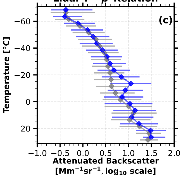
Lidar T - \beta Relation
