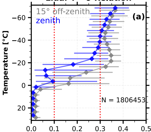
Lidar T - \delta Relation
