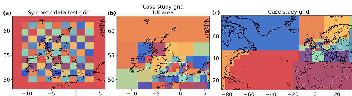
Figure 3. Spatial distributions of optimised regions, used in the (a) synthetic data tests and (b, c) case study. The centre (b) and right (c) plots are identical, with the centre plot a zoomed in section over the UK, showing how the quadtree algorithm places more regions in areas of greater sensitivity to emissions. The dashed white dashed line shows the area over which emissions are estimated during the case study – the south UK area (SUK). This is discussed in Sect. 3.2. Colours used in this plot have no meaning and are just used to differentiate between adjacent regions.
