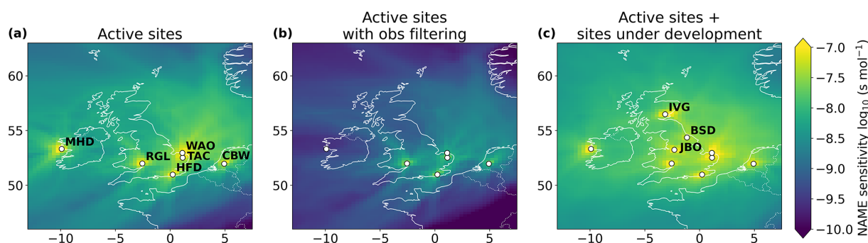
Figure 1. Example months of NAME sensitivity footprints for: (a) May 2023 with all observations from the current network of sites used in this work; (b) May 2023 with observations from the current network, filtered based on meteorological conditions, as used in the UK case study; and (c) May 2024 from the recently expanded network of sites as included in the synthetic study.
