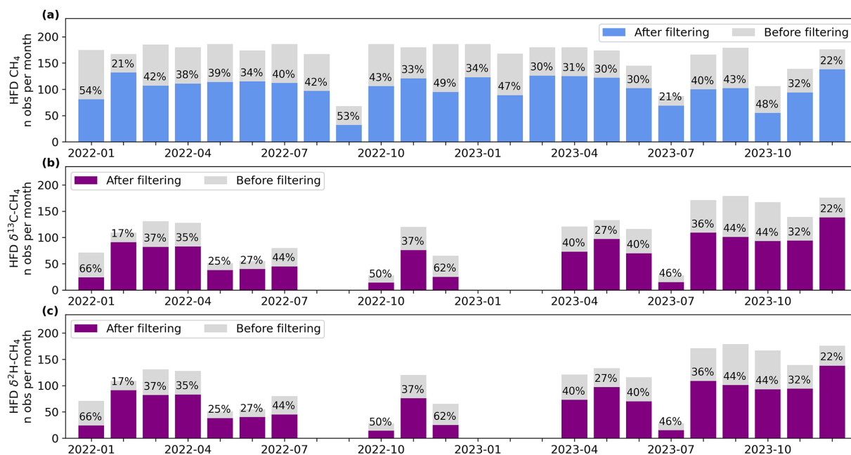
Figure B3. Number of 4-hourly averaged observations available from the Heathfield (HFD) site for each monthly inversion period before filtering (grey) and after filtering (coloured bar), for (a) methane, (b) \delta^{13}\text{C}\text{-CH}_4 and (c) \delta^2\text{H}\text{-CH}_4 . Annotated values give the percentage of observations that were removed by filtering based on meteorological conditions (see Sect. 2.4.3 for more information on this filtering).
