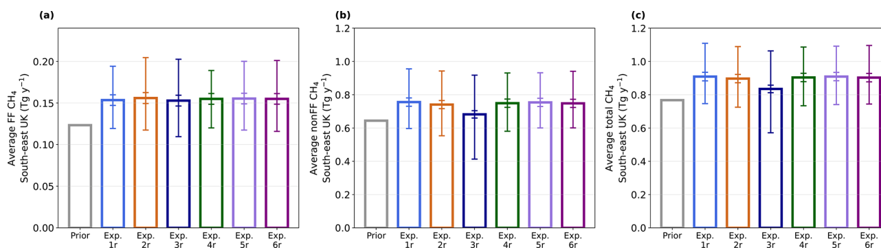
Figure 6. Posterior \text{CH}_4 flux estimates for the SUK area (as shown in Fig. 3) averaged across all 2022–2023 study months. Results for the (a) FF sector, (b) non-FF sector and (c) all sources, for the six different case study experiments are presented as a posterior mean across all months. With (narrower error bar) 1\sigma uncertainty of these posterior means and (wider error bar) RMSE of the posterior standard deviations across all monthly emission estimates. Descriptions for each experiment are given in Table 3.
