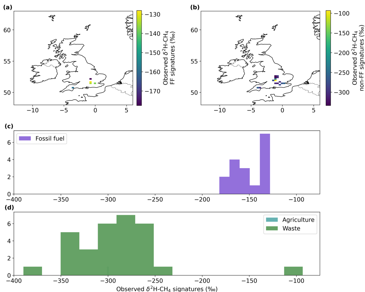
Figure B2. \delta^2\text{H}\text{-CH}_4 point source signatures compiled during the isoMET project (Dasgupta et al., 2025a, b) from (a, c) FF and (b, d) non-FF sources. Point source signatures have been averaged spatially and temporally to the 25 km resolution of the atmospheric transport model used in this study. The values are also presented as histograms. Only values for the waste sector are shown in the histogram, due to the lack of data for agriculture.
