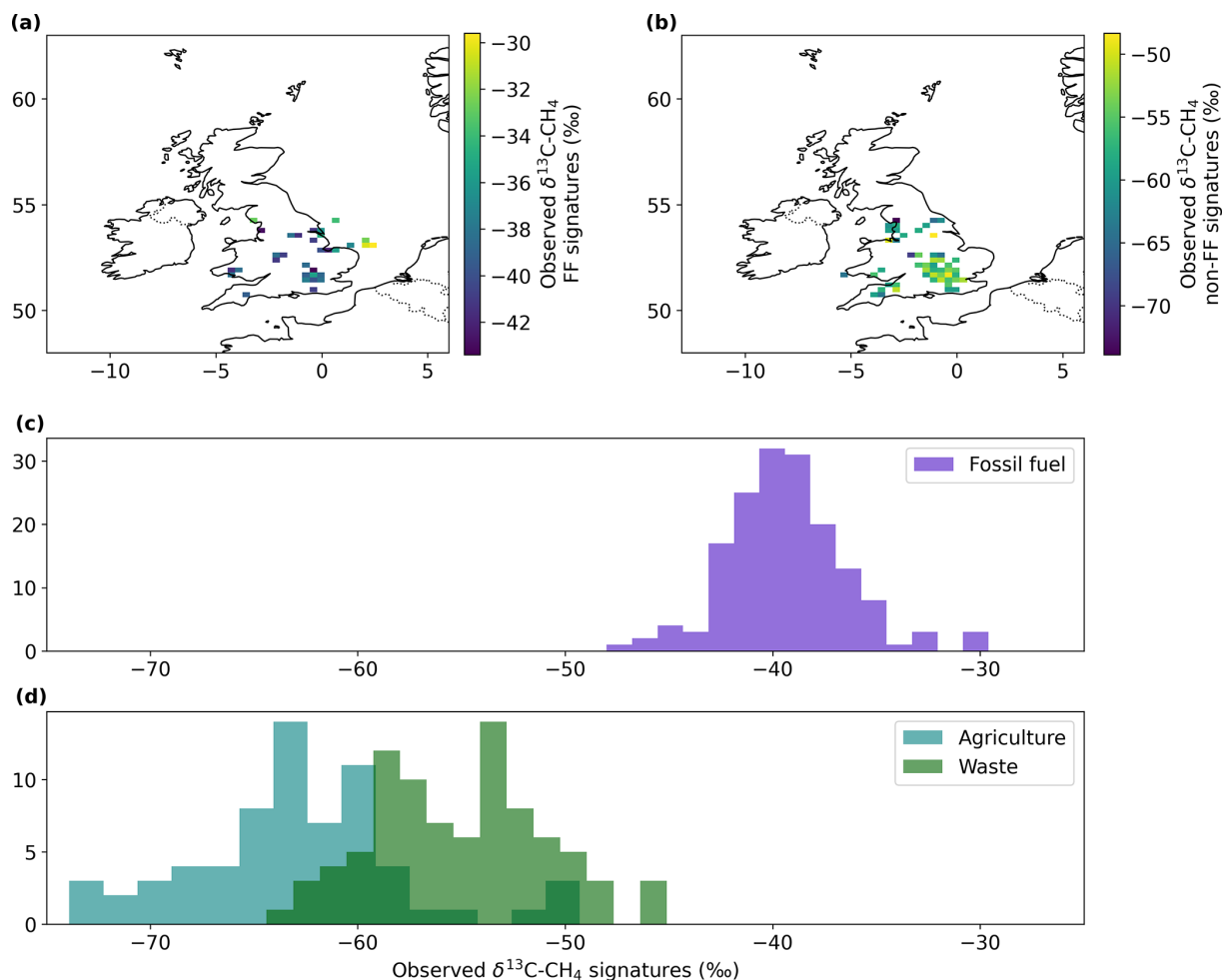
Figure B1. \delta^{13}\text{C-CH}_4 point source signatures compiled during the isoMET project (Dasgupta et al., 2025a, b) and observed by Royal Holloway during ground-based observation campaigns (Lowry et al., 2020; Menoud et al., 2022) from (a, c) FF and (b, d) non-FF sources. Point source signatures have been averaged spatially and temporally to the 25 km resolution of the atmospheric transport model used in this study. The same values are also presented as histograms, with non-FF sources split into (light blue) agriculture and (green) waste sources, showing the overlap between these two sectors.
