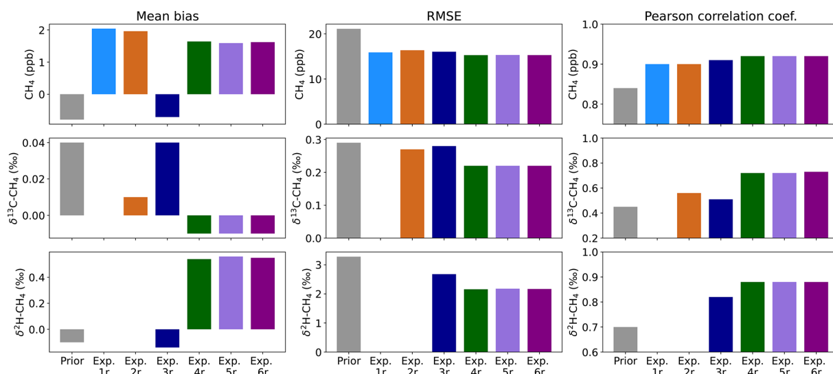
Figure B5. Statistics presenting the fit between observed and posterior mean modelled (top row) \text{CH}_4 mole fractions, (middle row) \delta^{13}\text{C}\text{-CH}_4 and (bottom row) \delta^2\text{H}\text{-CH}_4 for the six case study experiments (as described in Table 3). Statistics include: (left column) the bias between the posterior mean modelled and observed values, (middle column) the root mean square error (RMSE) between the posterior mean and observed values and (right column) the Pearson correlation coefficient of the posterior mean and observed values. The same statistics are given for the prior modelled mole fraction and isotope ratios, in grey.
