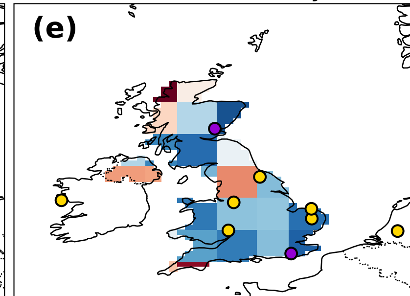
Exp. 5s: Uncertain region signatures 50% uncertainty
