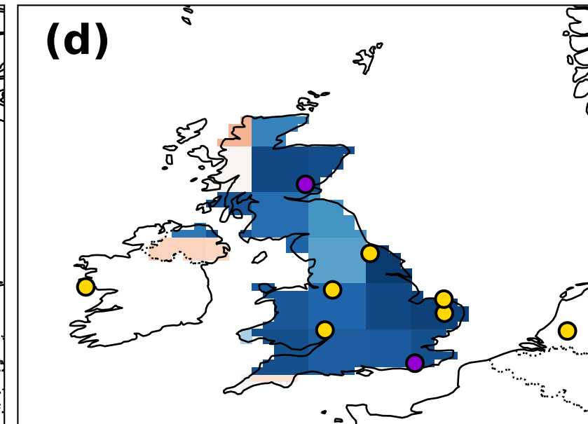
Exp. 4s: Uncertain sector signatures
