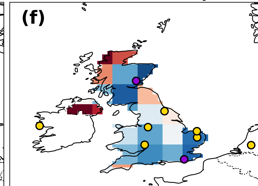
Exp 6s: Uncertain region signatures 100% uncertainty
