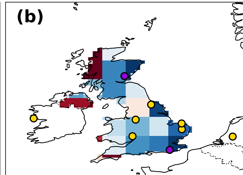
Exp. 2s: Known signatures no \delta^2\text{H}
