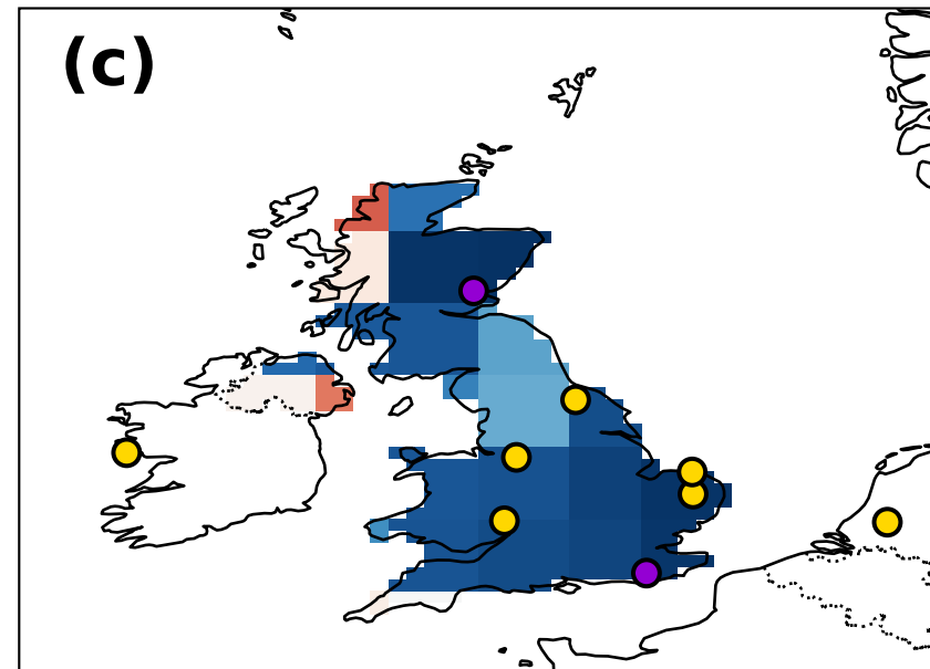
Exp. 3s: Known signatures ideal scenario
