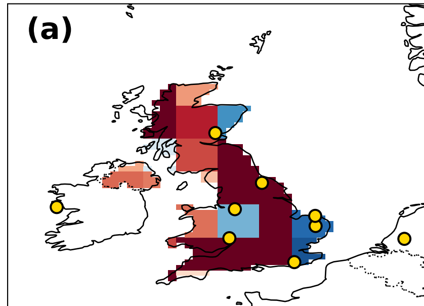
Exp. 1s: No isotopes
