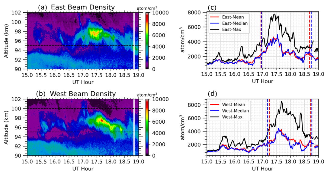
Figure 4. Time–height contours of SSL2 observed from the east beam (a) and west beam (b). Panels (c) and (d) show the corresponding time variations of sodium density within the altitude range of 95–100 km for the two beams. Red, blue, and black solid lines represent the mean, median, and maximum sodium densities, respectively. Vertical red and blue dashed lines indicate the onset and end times derived from mean and median sodium densities, defined as twice the background level.
