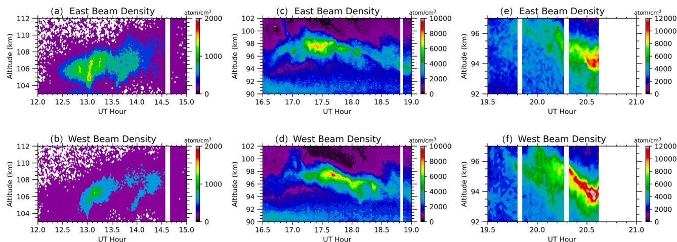
Figure 3. Time–height contours of SSL1 (a, b), SSL2 (c, d), and SSL3 (e, f). The upper panels show results from the east beam, and the lower panels show results from the west beam.
