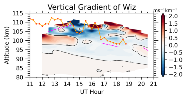
Figure 10. Time–height contour of vertical gradient of ion vertical drift derived from zonal wind measured by the USTC sodium lidar on 13 June 2013. Cold colors indicate negative dw_{iz}/dz (ion convergence region), while warm colors indicate positive dw_{iz}/dz (ion divergence region). The orange line denotes the altitude variation of the Es layer measured by the Wuhan ionosondes, and the dashed purple lines indicate the trajectories of the SSLs.
