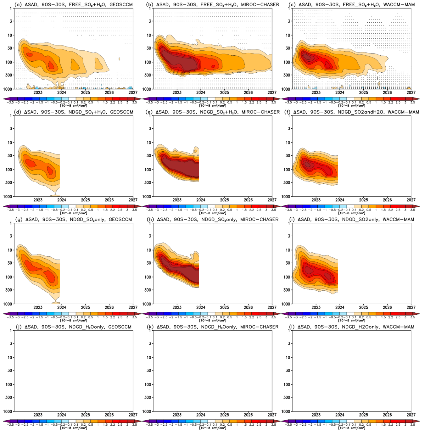
Figure S1. Pressure vs time changes (perturbed minus control) in the SH extratropical (90°S-30°S) aerosol SAD simulated in GEOSCCM (left), MIROC-CHASER (middle) and WACCM-MAM (right). Row 1 is for the free running experiment with simultaneous injection of SO 2 and H 2 O. Rows 2-4 are for the nudged simulations, either with SO 2 +H 2 O injection (row 2), SO 2 -only injection (row 3) or H 2 O-only injection (row 4). Stippling in row 1 marks regions where the response is not statistically significant (with the response taken as a significant if it exceeds \pm 2 standard errors in the difference in means). Note the aerosol SAD diagnostics used for GEOSCCM and MIROC included only sulfate while for WACCM-MAM this also included contribution from other aerosols (mostly in the troposphere); however, this will not affect the derived (perturbed minus control) response as the non-sulfate component should cancel out.
