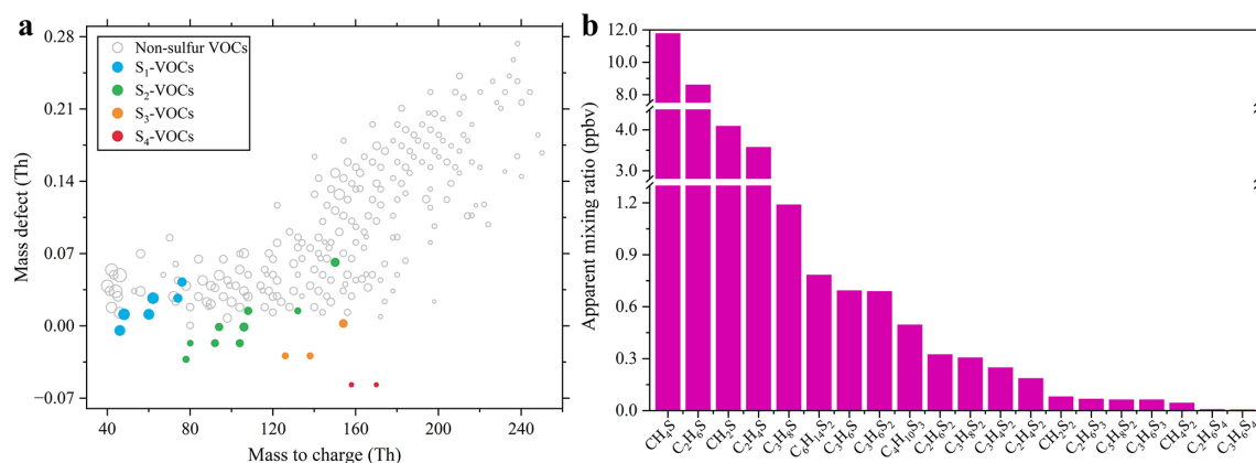
Figure 4. (a) Mass-defect plot of VOCs detected by Vocus-PTR-LToF-MS before oxidation. The 20 sulfur-VOCs are highlighted and grouped according to the number of sulfur atoms in their assigned molecular formulas, while non-sulfur VOCs are shown in gray. Marker size represents normalized PTR-MS signal intensity rather than calibrated concentration. (b) Semi-quantitative mixing ratios of the 20 sulfur-VOCs detected from the algal emissions.
