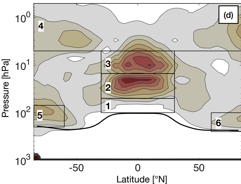
multi-model "full" standard deviation
