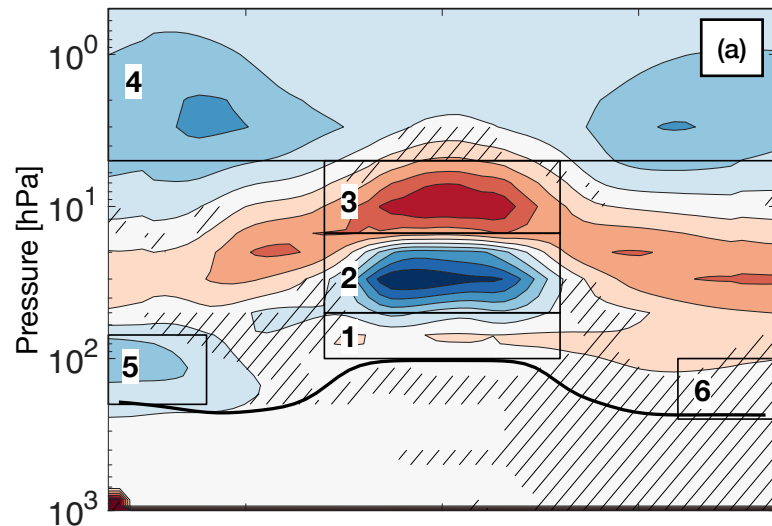
multi-model "full" standard deviation
