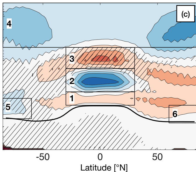
senD2-sai - senD2-chem ("dyn")
