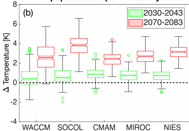
Tropopause cold point anomaly
