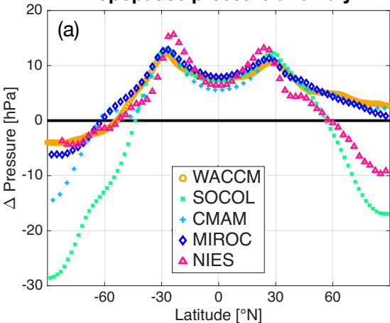
Tropopause pressure anomaly
