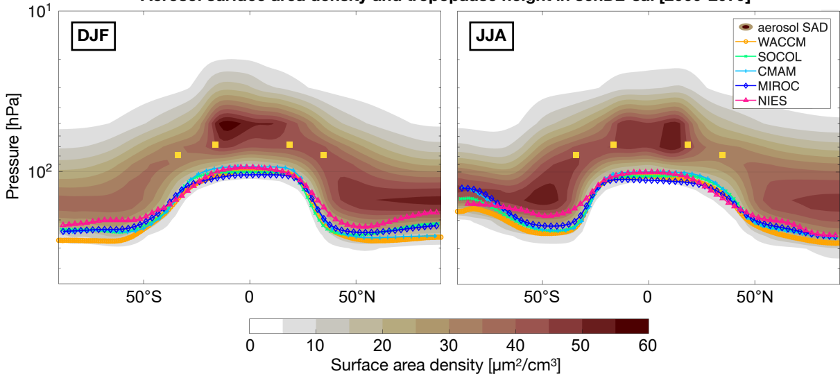
Aerosol surface area density and tropopause height in senD2-sai [2060-2079]
