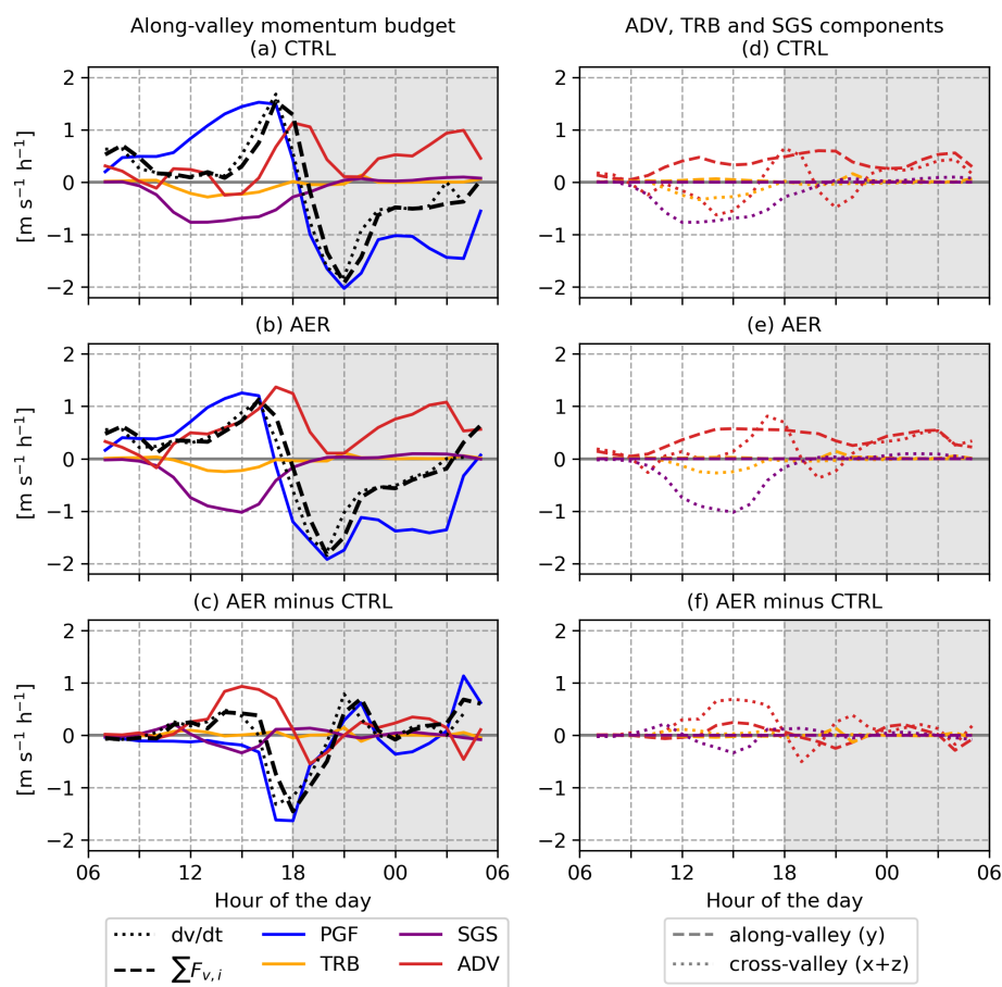
Figure 5. Along-valley momentum budget for the valley volume in (a) CTRL and (b) AER and (c) difference between the two cases. See Sect. 2.2 for details on the budget analysis. Left-hand-side of the Eq. (3) for along-valley momentum is shown on black dotted line and the sum of the terms on the right-hand-side as black dashed line, respectively. (d–f) Same as (a)–(c) but for the tendency due to mean advection, resolved turbulence and sub-grid-scale diffusion decomposed into along and cross-valley components. The cross-valley component includes the vertical one.
