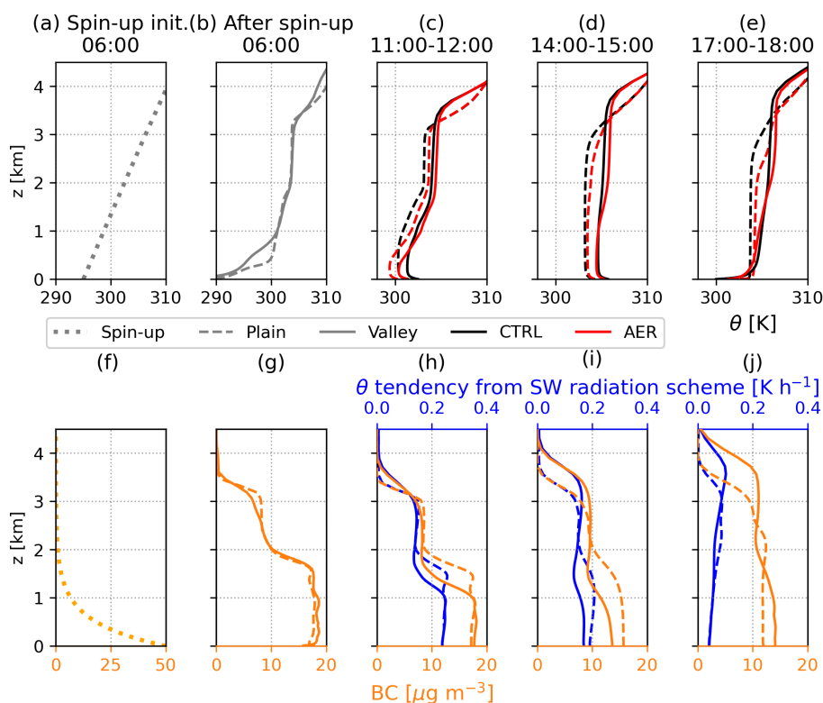
Figure 2. Top row: Vertical profile of potential temperature in both cases AER and CTRL. Bottom row: Vertical profile of black carbon and potential temperature tendency from the shortwave radiation scheme in case AER. (a, f) Horizontally uniform initial conditions of the spin-up run. (b, g) Initial condition of the cases AER and CTRL after the 24 h spin-up. Hourly averages between (c, h) 11:00–12:00 (d, i) 14:00–15:00 and (e, j) 17:00–18:00. Solid lines show the vertical profile averaged over the valley centre line ( y > 0 km, x = 0 km) and dashed lines above the plain ( y < 0 km, x = 0 km). Note the different temperature and black carbon concentration scales between the panels and that both cases AER and CTRL have the same spin-up and initial state shown in (a)–(b).
