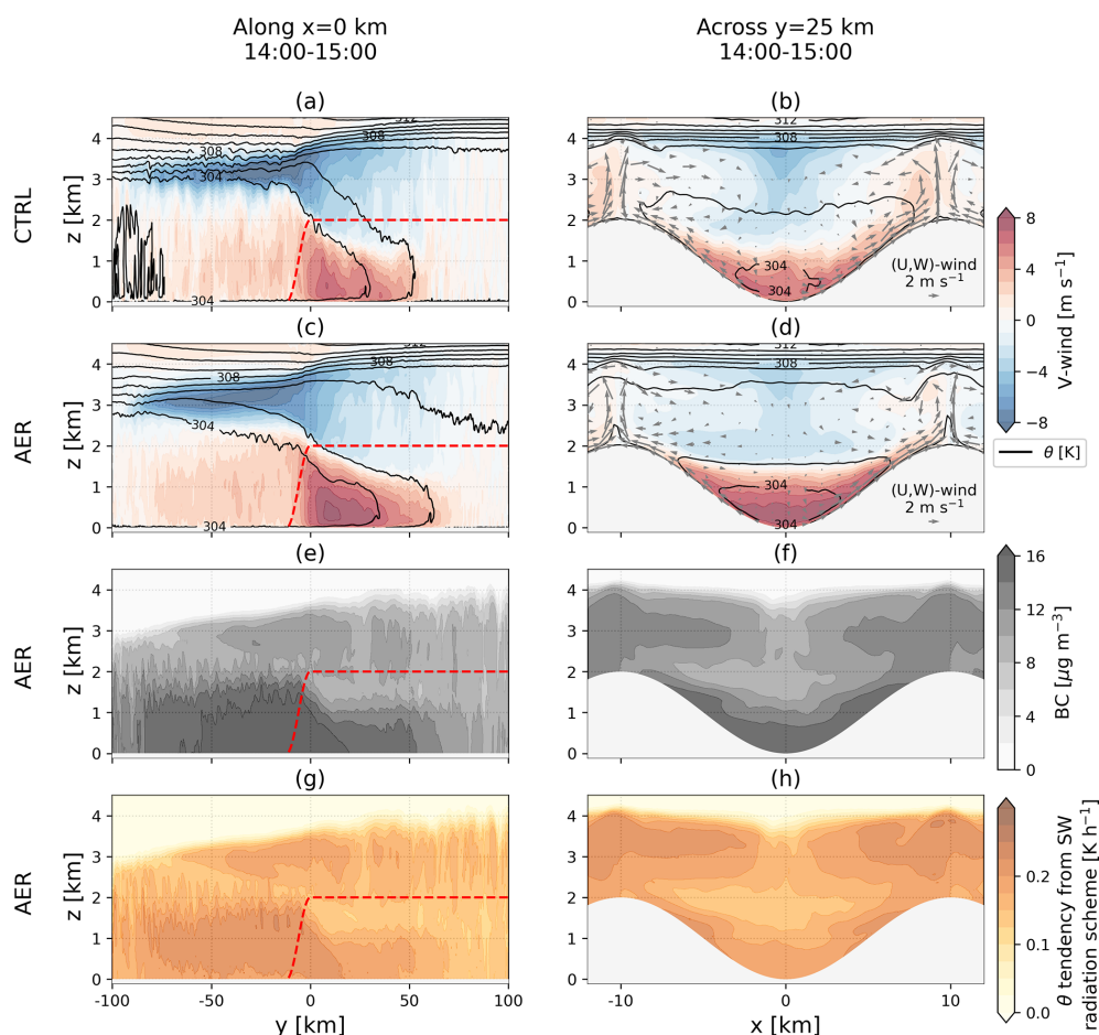
Figure 3. Cross-sections (a, c, e, g) along the valley centre line and (b, d, f, h) across the valley at y = 25 km averaged between 14:00 and 15:00. Panels (a)–(b) are from the case CTRL and panels (c)–(h) are from the case AER. (a)–(d) Along-valley wind speed (shaded) and potential temperature (black solid lines). Positive along-valley wind speed refers to up-valley hence right-ward wind in (a), (c). (e–f) Black carbon concentration. (g–h) Potential temperature tendency from shortwave radiation scheme. Red dashed line in (a), (c), (e), (g) show the ridge height at x = \pm 10 km.
