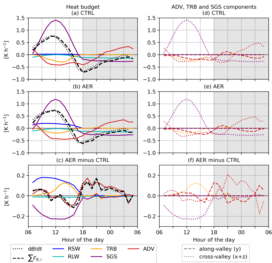
Figure 6. Heat budget for the valley volume in (a) CTRL and (b) AER and (c) difference between the two cases. See Sect. 2.2 for details on the budget analysis. Left-hand-side of the Eq. (3) for heat is shown on black dotted line and the sum of the terms on the right-hand-side on black dashed line, respectively. (d–f) Same as (a)–(c) but for the tendency due to mean advection, resolved turbulence and sub-grid-scale diffusion decomposed into along and cross-valley components. The cross-valley component includes the vertical one.
