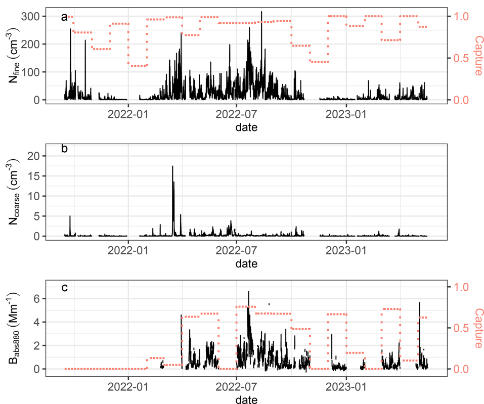
Figure 1. Time series of fine (a) and coarse (b) hourly PNC together with hourly aerosol absorption coefficient at 880 nm (c); right axis of panels (a) and (c) report the data capture of PNC and absorption coefficient measurements, respectively.
