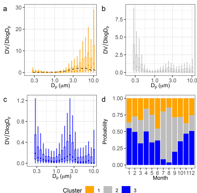
Figure 2. Particle volume size distribution corresponding to the three clusters ( a is cluster 1, b is cluster 2, and c is cluster 3): lines indicate 5th–95th percentile ranges, bars correspond to 25th–75 percentile ranges, while markers indicate median values; black dotted line in panel ( a ) is the average median size distribution corresponding to the intense dust event of March 2022. Panel ( d ) shows cluster monthly probability.
