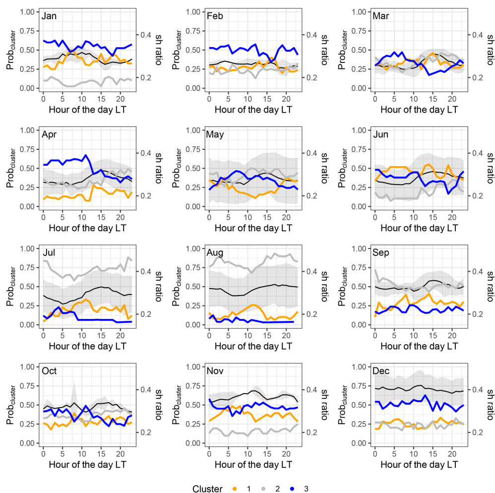
Figure 3. Monthly diurnal variability of cluster occurrence frequency (cluster 1 in orange, cluster 2 in gray, and cluster 3 in blue) together with diurnal variability of the specific humidity ratio (black line corresponds to the average while shaded area is the standard deviation range).
