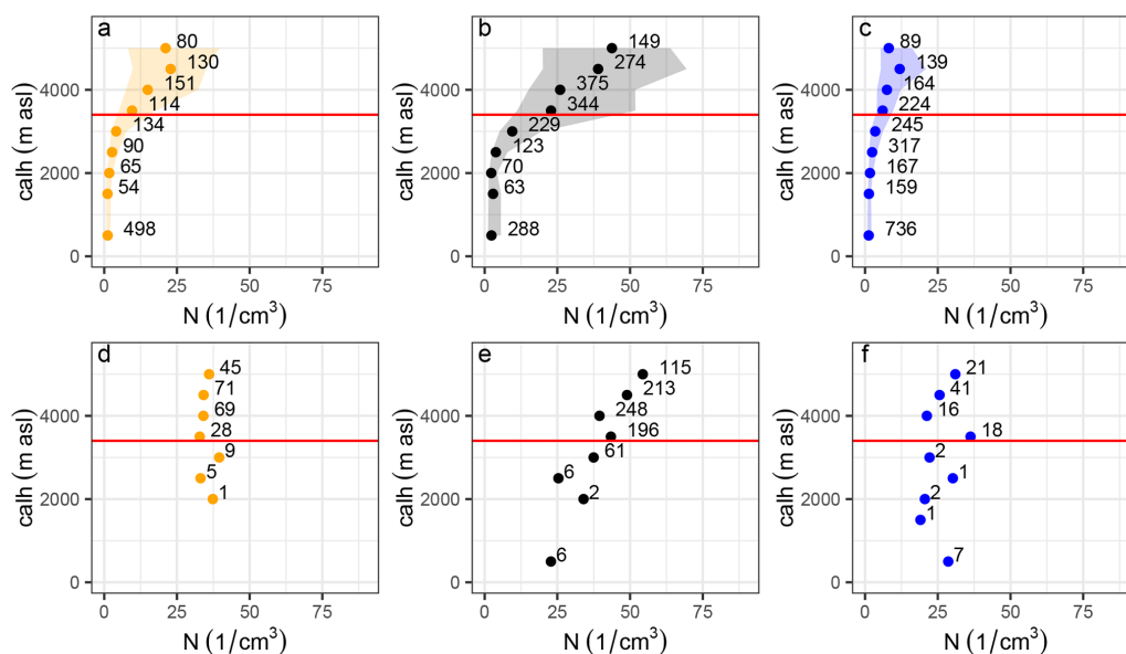
Figure 4. Average particle number concentration as a function of continuous aerosol layer height (calh) for the three different clusters during the entire observation period (panels a–c ) and when particle number concentration exceeded the 75th percentile (panels d–f ); the shaded areas indicate the 25th–75th percentile range, the number close to each marker indicate the number of observations corresponding to each altitude bin, while the red line indicates the altitude of the Testa Grigia observatory.
