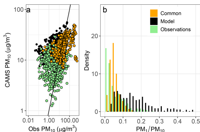
Figure 6. Panel (a): comparison between hourly \text{PM}_{10} concentration reconstructed from particle volume size distribution (Obs \text{PM}_{10} ) and modeled by CAMS (CAMS \text{PM}_{10} ) (in orange when dust presence is identified by both model and observations, in green when dust is identified exclusively by the observations, and in black when only CAMS detect dust transport); panel (b): frequency distribution of the \text{PM}_1 to \text{PM}_{10} ratio estimated from particle size distribution and corresponding to the types of events.
