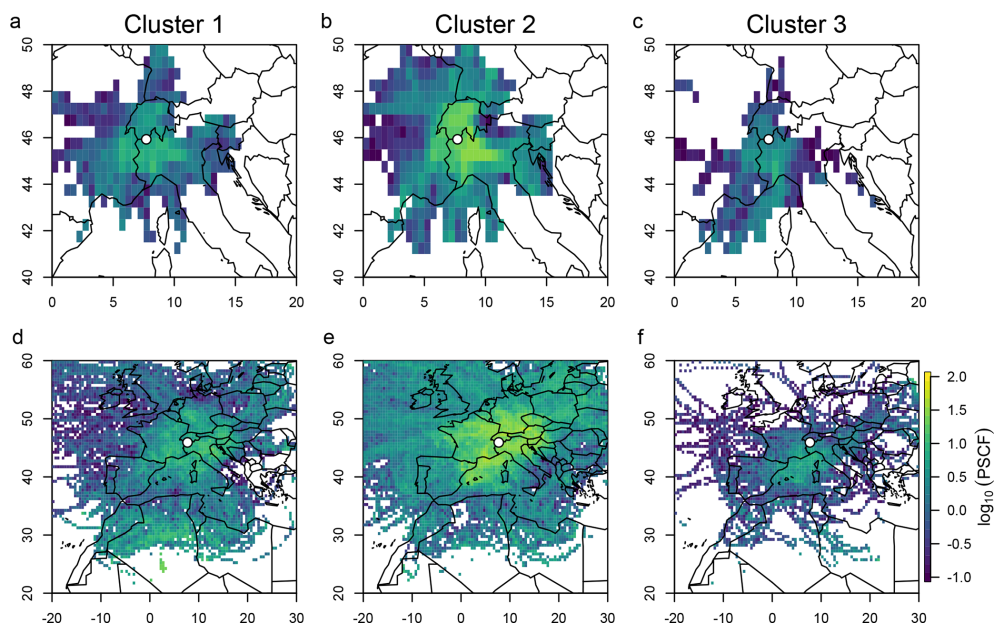
Figure 5. PSCF maps of 24 h back trajectories ( a–c ) and 7 d back trajectories ( d–f ) for cluster 1 ( a, d ), cluster 2 ( b, e ), and cluster 3 ( c, f ), when total particle number concentration was larger than the 75th percentile. The white circle indicates the position of the Testa Grigia observatory.
