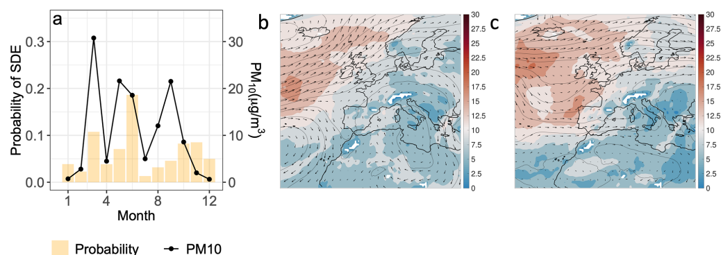
Figure 7. Monthly probability of SDE observed at Testa Grigia, together with the monthly medians of PM 10 concentration (a); maps of average geopotential heights (contour lines; every 20 dam), wind speeds (color; in m s -1 ) and averaged wind arrows over Europe and north Africa during SDE periods in March, May, and June (b) and in October and November (c).
