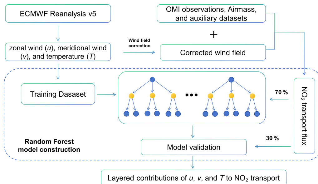
Figure 2. Schematic framework illustrating the computation of NO 2 transport fluxes, wind-field correction, and Random Forest-based diagnostic analysis.
