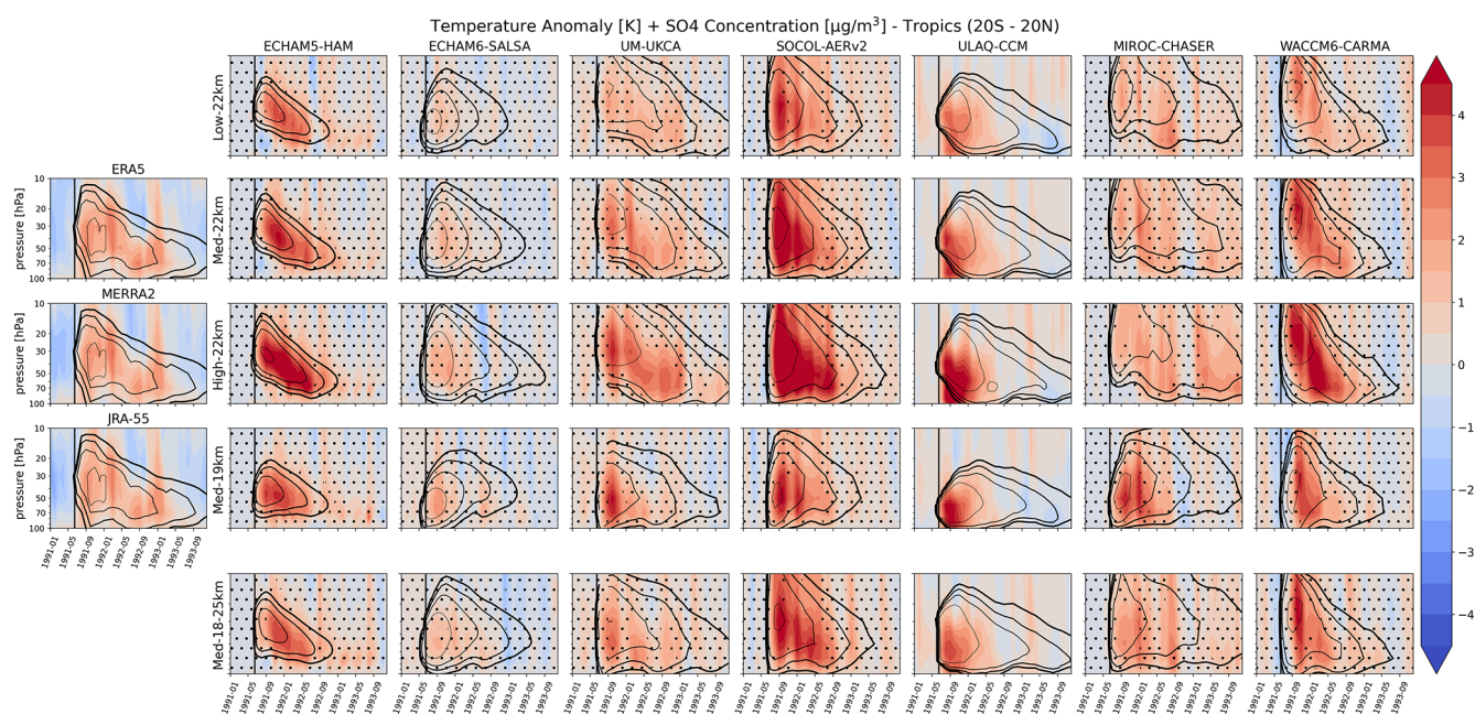
Figure A4. Vertical time evolution of the temperature anomalies for all experiments and models in the tropics (20° S–20° N). In all panels: SO 4 concentrations are shown as contours (levels are 0.5, 1, 2, 5 μg m -3 ), dots indicate non-significant areas ( p -value > 0.05) for reanalysis and models with the exception of ULAQ-CCM where only one ensemble member is available, and the thick black vertical line represents the Mt. Pinatubo eruption time.
