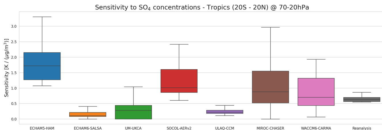
Figure 5. Stratospheric temperature sensitivity to \text{SO}_4 absorptive-heating of the ISA-MIP models and reanalysis in the tropics ( 20^\circ\text{S} – 20^\circ\text{N} ) between 70 and 20 hPa. The boxplots contain data for altitude weighted longitude–latitude pairs, obtained by regressing temperature anomalies against \text{SO}_4 concentrations over time.
