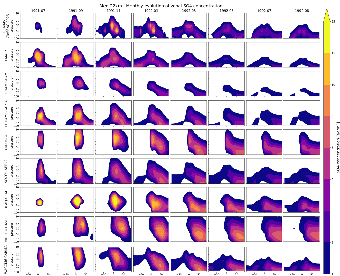
Figure 2. Vertical evolution of zonal mean \text{SO}_4 concentrations in experiment Med-22km for individual models, from July 1991 to August 1992 (bi-monthly; columns) in comparison with REMAP-GloSSAC-2023 observations (first row). Note, EMAC is flagged with * as it did not fully adhere to the ISA-MIP protocol, see Sect. 2.2.8.
