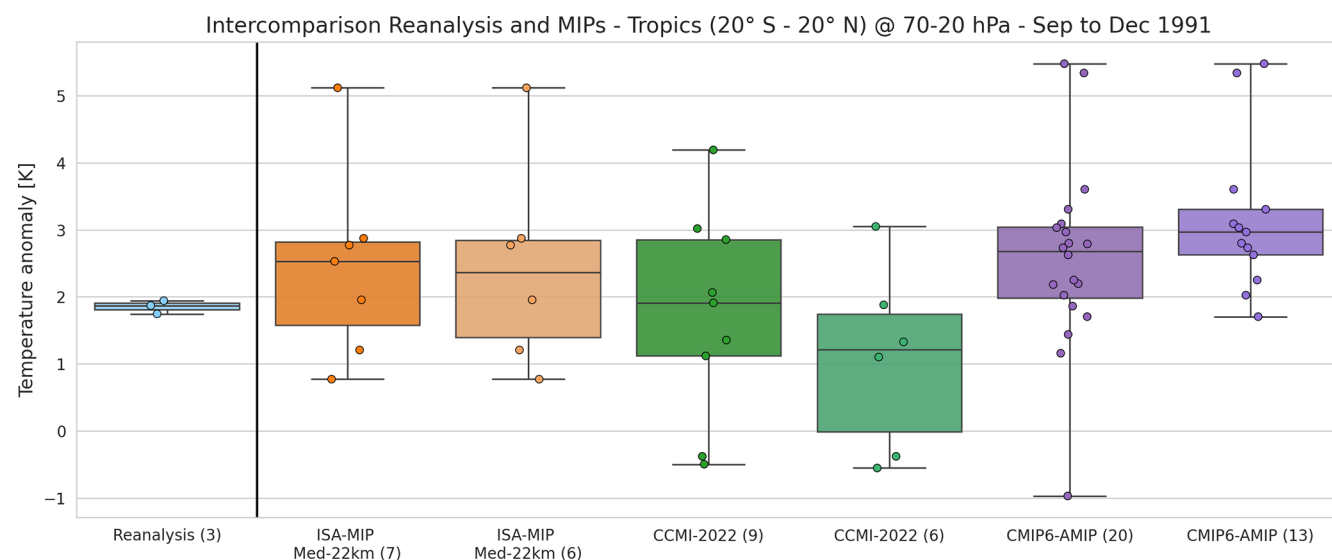
Figure 6. Temperature anomaly distributions for reanalyses (left), ISA-MIP and CCMI-2022 (center) and CMIP6-AMIP (right) in the tropics ( 20^{\circ}\text{S} – 20^{\circ}\text{N} ) averaged between 70 and 20 hPa in the period September to December 1991. The number in brackets indicates the number of models used. Solid vertical line separates reanalysis from models. Light orange, light green and light purple boxplots represent models with more than one ensemble member. Individual model results are provided as dots in the same colour of the corresponding MIP/sample. For convenient reference we note the order of ISA-MIP models in descending temperature anomaly: SOCOL-AERv2, ECHAM5-HAM, WACCM6-CARMA, ULAQ-CCM, UM-UKCA, ECHAM6-SALSA, MIROC-CHASER.
