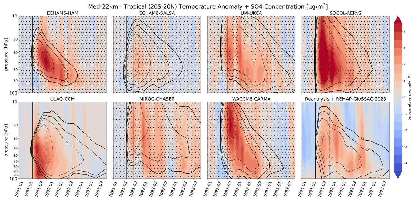
Figure 3. Time evolution of the vertical temperature anomalies in the tropics ( 20^{\circ}\text{S} – 20^{\circ}\text{N} ) in experiment Med-22km for individual models. In all panels: \text{SO}_4 concentrations are shown as contours (levels are 0.5, 1, 2, 5 \mu\text{g m}^{-3} ), dots indicate non-significant areas ( p -value > 0.05 ) for reanalysis and models with the exception of ULAQ-CCM where only one ensemble member is available, the thick black vertical line represents the Mt. Pinatubo eruption time while the thin vertical lines embed the time period September to December 1991. REMAP-GloSSAC-2023 \text{SO}_4 concentrations are shown as contours in the reanalysis panel.
