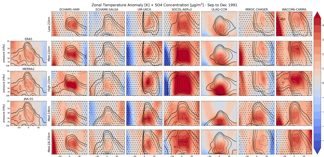
Figure A5. Vertical zonal temperature anomaly for all experiments and models for the period September to December 1991. In all panels: \text{SO}_4 concentrations are shown as contours (levels are 0.5, 1, 2, 5 \mu\text{g m}^{-3} ), dots indicate non-significant areas ( p -value > 0.05) for reanalysis and models with the exception of ULAQ-CCM where only one ensemble member is available, and the vertical lines embed the tropical region (20° S–20° N).
