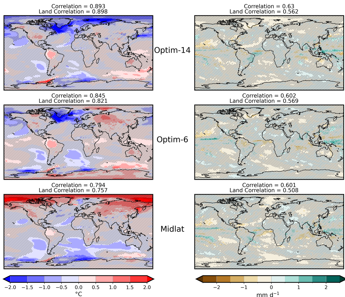
Figure 12. Difference in temperature and precipitation 2040s mean responses of Optim-14, Optim-6 and Midlat from the 2014–2033 target. Area-weighted spatial Pearson correlation scores, calculated both globally and over land, are annotated, with hatching showing non-significant grid points at the p < 0.05 level using a Student's t -test.
