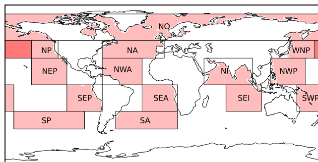
Figure 1. The locations of the 14 different regions where MCB is deployed in this study. The different regions are: Northern Ocean (NO), North Pacific (NP), North-East Pacific (NEP), South-East Pacific (SEP), South Pacific (SP), Western North Pacific (WNP), North-West Pacific (NWP), South-West Pacific (SWP), North Atlantic (NA), North-West Atlantic (NWA), South-East Atlantic (SEA), South Atlantic (SA), Northern Indian (NI), and South-East Indian (SEI). The red shading shows the open ocean grid points of a given box, showing where SSA are emitted. Note that the WNP and NP regions overlap, illustrated by the darker shading, as outlined in Table 1.
