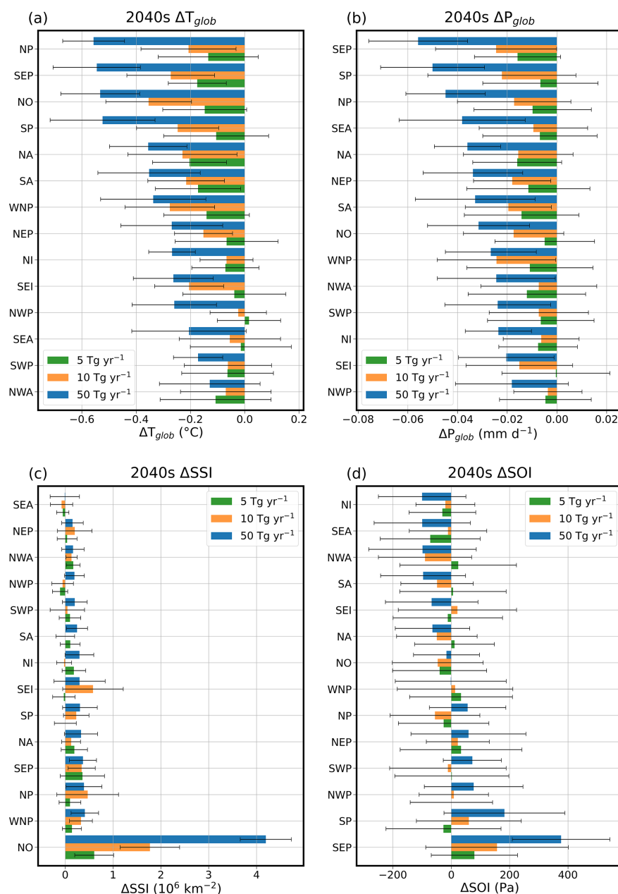
Figure 6. The 2040s mean responses of the patch simulations for global mean surface air temperature anomaly ( \Delta T_{glob} ), global mean precipitation anomaly ( \Delta P_{glob} ), Arctic September sea ice extent anomaly ( \Delta \text{SSI} ) and Southern Oscillation Index anomaly ( \Delta \text{SOI} ) are shown in panels (a)–(d) respectively. The 5, 10 and 50 Tg yr -1 responses are shown as green, orange and blue bars respectively. Error bars show one standard deviation of the annual mean responses.
