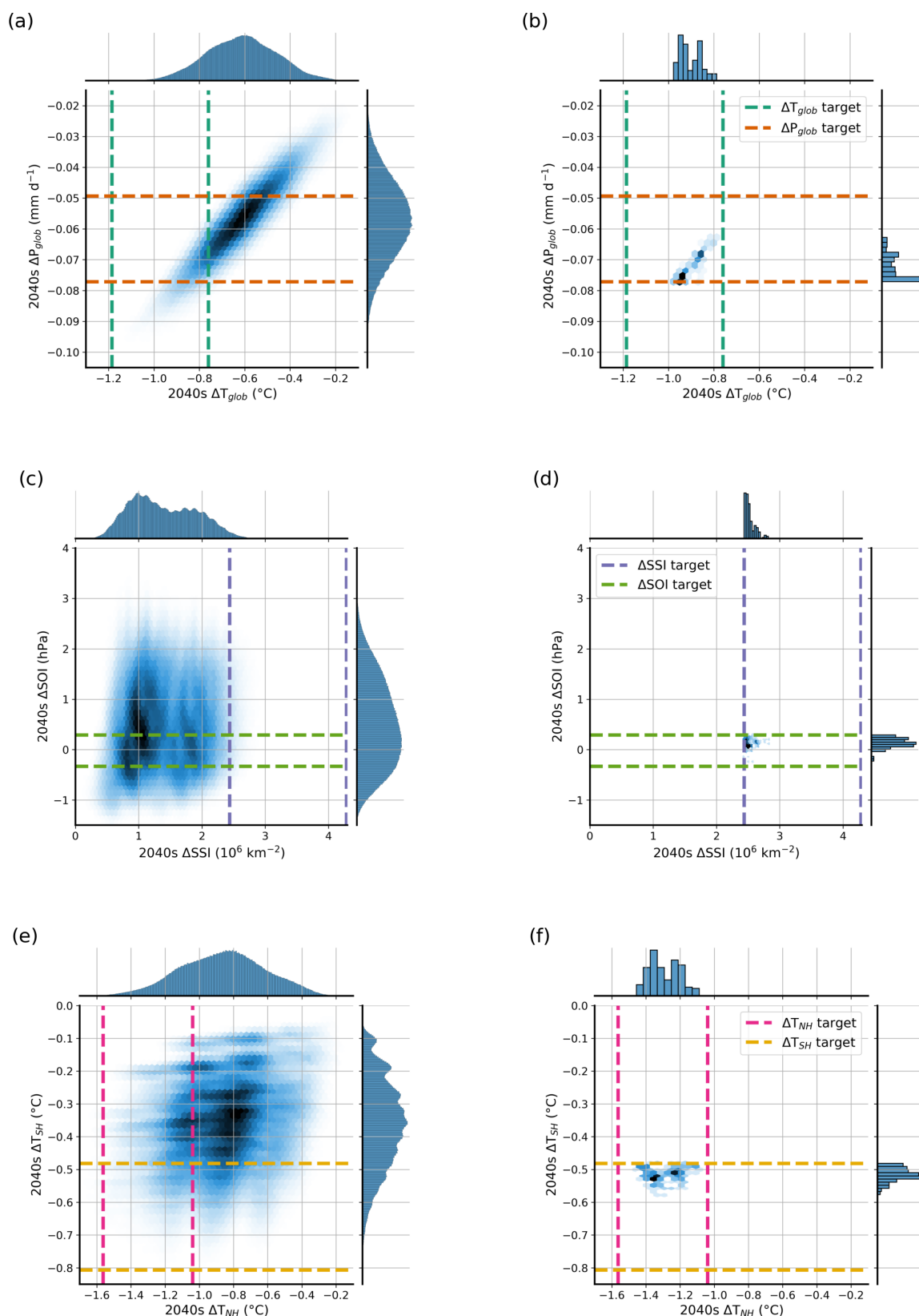
Figure 10. Heatmaps showing the narrowing down of the combinations based on climate response targets defined in Table 2. Panels (a), (c) and (e) show the heatmaps for the 1 144 066 combinations. Panels (b), (d) and (f) show the heatmaps for the remaining 172 combinations that satisfy all 6 climate response targets. Dashed lines show the upper and lower bounds of a given target.
