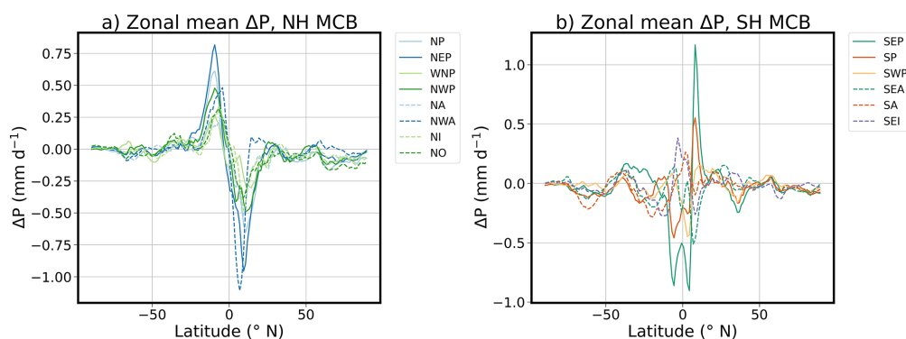
Figure 5. Zonal mean 2040s precipitation anomaly ( \Delta P ) for the 50 \text{ Tg yr}^{-1} patch simulations in (a) the Northern Hemisphere (NH) and (b) the Southern Hemisphere (SH) relative to SSP2-4.5.
