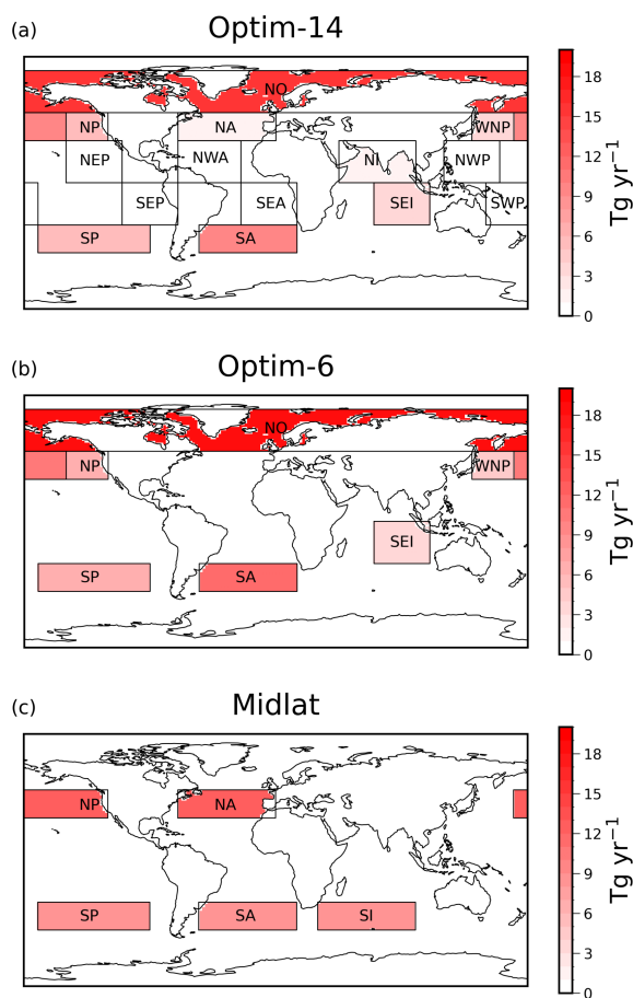
Figure 11. The distribution of the 50 \text{ Tg yr}^{-1} deployments for (a) Optim-14, (b) Optim-6 and (c) Midlat.
