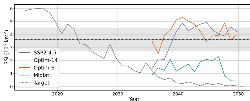
Figure 14. Arctic September sea ice extent (SSI) responses of Optim-14, Optim-6 and Midlat, compared to SSP2-4.5. The dashed line shows the 2014–2033 target and the shading shows the target range used in the methodology to produce Optim-14 and Optim-6, as described in Sect. 4.
