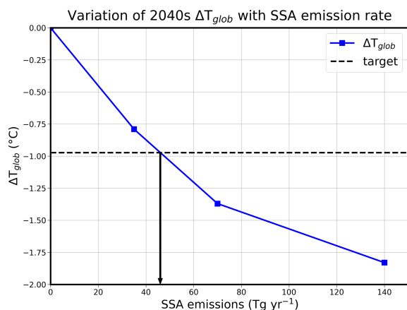
Figure 8. Variation of 2040s global mean surface air temperature anomaly ( \Delta T_{\text{glob}} ) with sea salt aerosol (SSA) emission rate for a 35, 70 and 140 \text{Tg yr}^{-1} MCB deployment with the SSA shared equally across the 14 regions. The dashed line indicates the target cooling required to restore the 2014–2033 \Delta T_{\text{glob}} . Linear interpolation suggests a 46 \text{Tg yr}^{-1} is required to achieve this cooling target.
