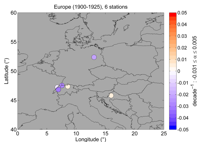
Figure 2. Spatial distribution of decadal BAOD trends based on annual means at six European sites over the period 1900–1925. The number of sites is shown at the top. The colour-coded bar indicates the magnitude of the BAOD trend, whose range is indicated on the side. \alpha represents the trend value computed with DLM.
