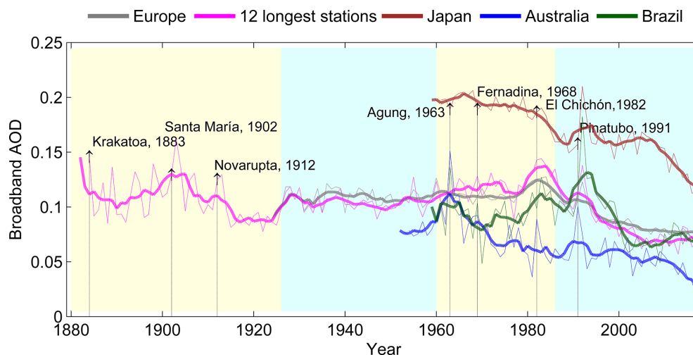
Figure 8. Overview of annual BAOD mean time series over Europe (gray line), 12 longest European stations (magenta line), Japan (brown line), Australia (blue line) and Southeast Brazil (green line). The period is from 1880 onwards.
