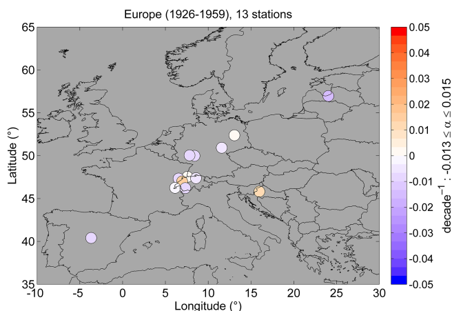
Figure 4. Spatial distribution of decadal BAOD trends based on annual means at 13 sites in Europe during the period 1926–1959. The colour-coded bar indicates the BAOD trend, whose range is indicated on the side. \alpha represents the trend value computed with DLM.
