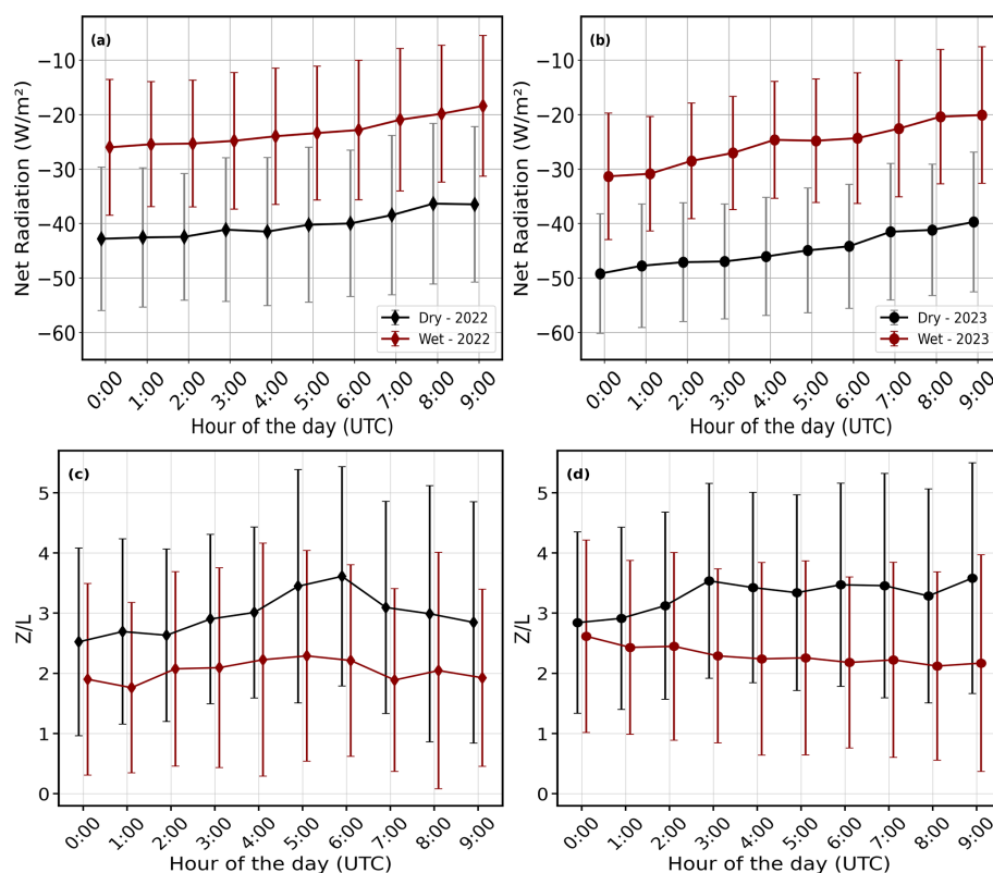
Figure 2. Hourly mean values of (a, b) net radiation ( R_n ) measured at 81 m and (c, d) stability parameter ( z/L ) calculated at 50 m for the Wet season (red) and the Dry season (black) during 2022 (left panels) and 2023 (right panels). The bars indicate the standard deviation.
