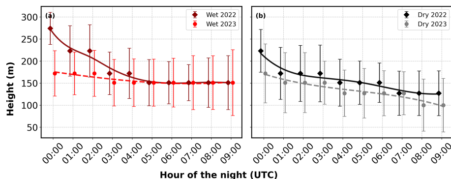
Figure 5. Mean values and standard deviation of h_n for (a) the Wet period of 2022 and 2023 and (b) the Dry period of 2022 and 2023. The curves represent smooth fits obtained by spline between the mean h_n values.
