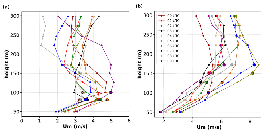
Figure 7. Hourly mean wind speed profiles for (a) 18 August 2022 and (b) 25 August 2022. The different colors indicate the different hours. The larger hollow circles mark the hourly estimates of the h_n .
