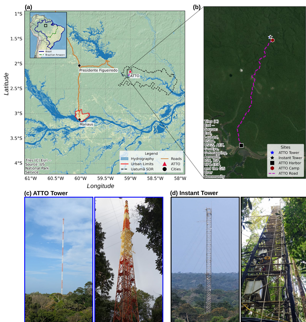
Figure 1. Geographic location and infrastructure of the Amazon Tall Tower Observatory (ATTO). (a) Regional map showing the position of ATTO northeast of Manaus, within the Uatuma Sustainable Development Reserve (SDR); (b) High-resolution zoom around the ATTO site based on Esri World Imagery, showing the ATTO Tower (blue star), Instant Tower (black star), ATTO harbor (black square), ATTO Camp (brown hexagon), and the ATTO access road (magenta dashed line); (c) Photographs of the ATTO Tower (325 m) from ground perspective and structural details of its metallic frame; (d) Photographs of the Instant Tower (80 m). All maps were generated using Python 3.11.6, in the WGS84 geographic coordinate system (EPSG:4326). Basemaps: Esri World Physical (a) and Esri World Imagery (b). Sources: Esri, TomTom, FAO, USGS | Powered by Esri.
