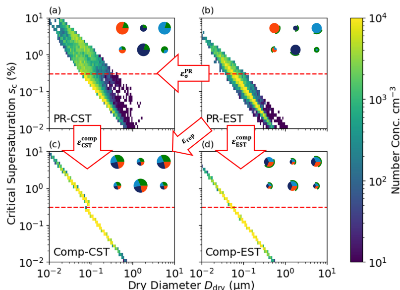
Figure 1. Schematic of the four aerosol representations considered in this study. The top row shows particle-resolved (PR) cases under constant surface tension (PR-CST, a ) and effective surface tension (PR-EST, b ). The bottom row shows composition-averaged (Comp) cases under constant surface tension (Comp-CST, c ) and effective surface tension (Comp-EST, d ). The red dashed line indicates the prescribed environmental supersaturation (0.3 %) used to diagnose CCN activation; particles with critical supersaturation below this threshold are classified as CCN-active. The schematic particles in the upper-right corner of each panel illustrate how individual aerosols are represented under each scenario: green denotes organic material and the other colors denote the inorganic species. Horizontal comparisons isolate surfactant effects, vertical comparisons isolate the impact of composition averaging, and the diagonal comparison between PR-EST and Comp-CST represents the bias of a modal-like representation relative to the particle-resolved reference.
