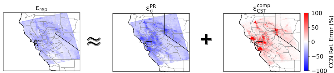
Figure 6. Spatial distribution of the primary model-relevant CCN bias, \epsilon_{rep} , and its decomposition into contributions from surfactant-induced surface tension effects ( \epsilon_{\sigma}^{PR} ) and composition averaging under constant surface tension ( \epsilon_{CST}^{comp} ) at s_{env} = 0.3\% .
