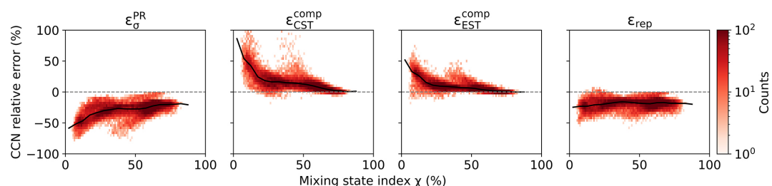
Figure 11. CCN relative differences ( \epsilon_{\sigma}^{\text{PR}} , \epsilon_{\text{CST}}^{\text{comp}} , \epsilon_{\text{EST}}^{\text{comp}} , and \epsilon_{\text{rep}} ) as a function of aerosol mixing state index \chi for all particles. Black lines indicate binned median values and the color scale represents data density on a logarithmic scale. To improve sampling across mixing states, data from two representative time steps (12:00 LST on 18 June and 00:00 LST on 19 June 2010) are combined.
