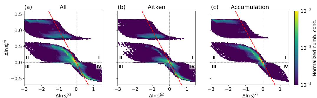
Figure 4. Particle-level decomposition of changes in critical supersaturation induced by composition averaging under the EST framework, with the x -axis showing the hygroscopicity contribution \Delta \ln s_c^{(\kappa)} = -\frac{1}{2} (\ln \kappa^{\text{comp}} - \ln \kappa^{\text{PR}}) and the y -axis showing the surface tension contribution \Delta \ln s_c^{(\sigma)} = \frac{3}{2} (\ln \sigma^{\text{comp}} - \ln \sigma^{\text{PR}}) (Eq. 7). Colors indicate the normalized particle number concentration. The origin corresponds to no change in activation properties; positive (negative) values indicate an increase (decrease) in s_c and thus suppressed (enhanced) activation. The four quadrants identify regimes where \kappa and \sigma effects reinforce (Quadrants I and III) or compensate (Quadrants II and IV). The red dashed line marks \Delta \ln s_c^{(\sigma)} = -\Delta \ln s_c^{(\kappa)} , where the \kappa and \sigma contributions exactly compensate and the net change in \ln s_c is zero. Panels show all particles and mode-separated subsets (Aitken and accumulation), highlighting the mode-dependent weighting of the compensating regime.
