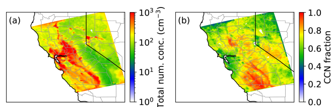
Figure 5. Spatial context of the WRF-PartMC case over California (12:00 LST, 18 June 2010) for the land grid cells analyzed in this study. Panel (a) shows the near-surface total particle number concentration, and panel (b) shows the CCN activation fraction at s_{\text{env}} = 0.3 \% .
