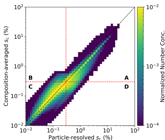
Figure 3. Same as Fig. 2 but evaluated within the effective surface tension (EST) framework. The x -axis shows particle-resolved s_c computed with EST ( s_c^{\text{PR,EST}} ), and the y -axis shows s_c after composition averaging, also evaluated with EST ( s_c^{\text{comp,EST}} ). The dashed black 1 : 1 line and red dashed s_{\text{env}} = 0.3\% threshold define the same gain-loss quadrants as in Fig. 2.
