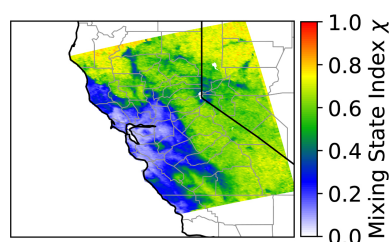
Figure 10. Spatial distribution of the aerosol mixing state index \chi for the near-surface land grid cells analyzed in this study. Low \chi regions correspond to more externally mixed aerosol populations, whereas high \chi regions indicate more internally mixed aerosol.
