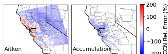
Figure 8. Mode-resolved spatial patterns of the primary model-relevant CCN bias \epsilon_{rep} at s_{env} = 0.3\% , shown separately for Aitken and accumulation modes.
