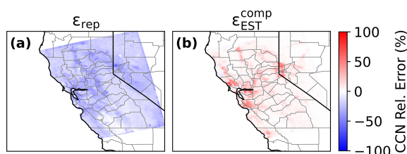
Figure 7. Comparison between the primary model-relevant bias \epsilon_{rep} and the composition-averaging-induced bias under effective surface tension, \epsilon_{EST}^{comp} , at s_{env} = 0.3\% . This comparison isolates the residual impact of composition averaging when surfactant effects are included.
