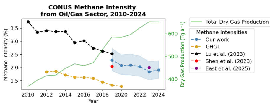
Figure 4. National methane intensity trends for the oil/gas sector in CONUS, 2010–2024. The 2019–2024 trend from this work (best posterior estimate and range from the ensemble) is compared to a 2023 TROPOMI inversion (East et al., 2025), a 2019 inversion of older TROPOMI retrievals (Shen et al., 2023), the 2010–2019 trend from an inversion of GOSAT and NOAA observations (Lu et al., 2023), and the GHGI trend extending to 2020. Total dry gas production of methane is from the U.S. Energy and Information Administration (U.S. EIA, 2025).
