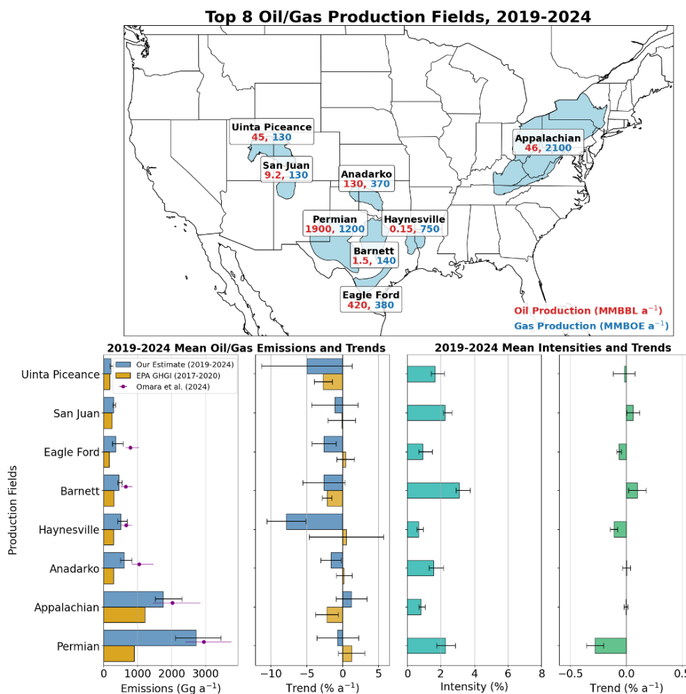
Figure 6. 2019–2024 mean oil/gas production, emissions, emission intensities, and trends for the top eight oil/gas production fields in CONUS. Emissions and emission intensities are from the mean of our posterior estimates, with error bars representing the ranges from the inversion ensemble (for the 2019–2024 mean panels) or the standard error on the regression slopes (for the trends). Emission estimates from Omara et al. (2024) are for 2021 emissions. Trends are calculated using OLS regression on results for individual years. Production data were derived from the Enverus prism platform (Enverus, 2025). MMBBL is million barrels of oil and MMBOE is million barrels of oil equivalent. Oil/gas field boundaries are based on definitions in Omara et al. (2024).
