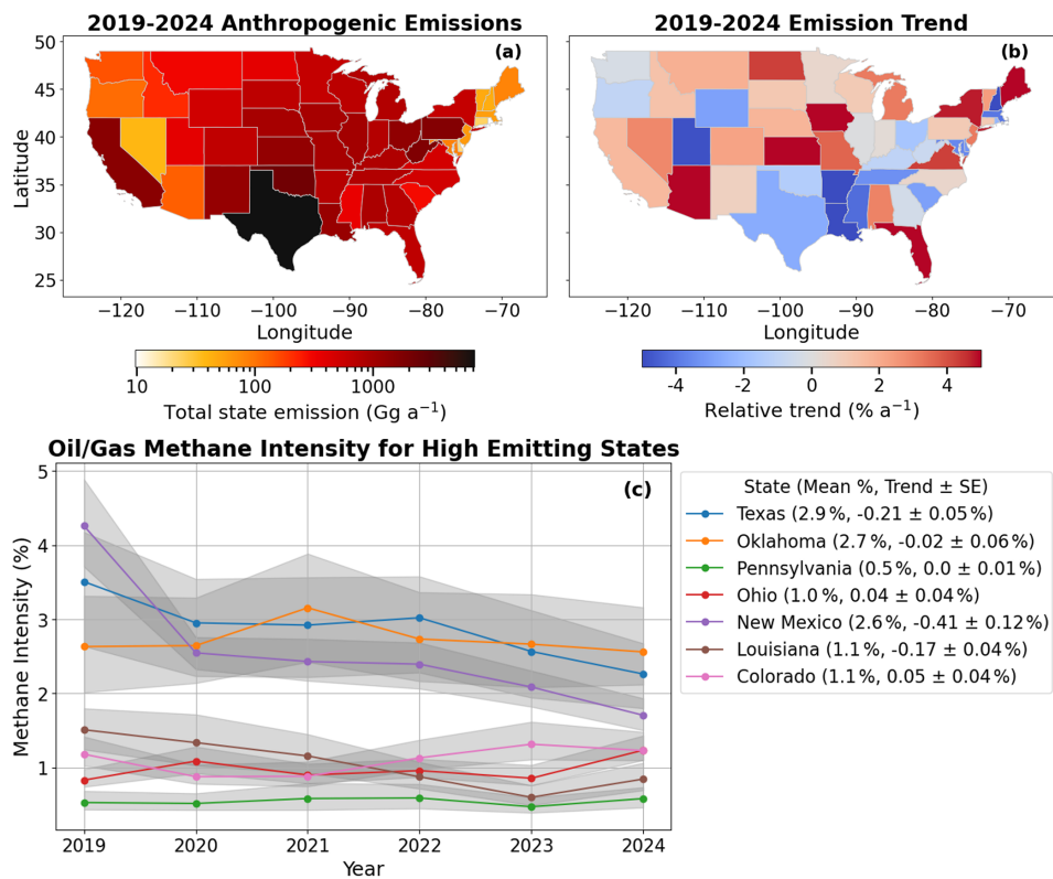
Figure 5. Mean 2019–2024 anthropogenic emissions, trends, and intensities for individual states. Panel (a) shows mean anthropogenic emissions on a log scale. Panel (b) shows the percent change per year from a linear regression of the emissions for each state. Panel (c) shows methane intensities from the oil/gas sector for the six states dominated by oil/gas emissions and Colorado. The trends and standard errors (SE) are from ordinary least squares regression of the mean intensity for each year. EIA data on individual state dry production for 2024 was unavailable at the time of writing, so we estimate dry production from marketed gas using the ratio of dry production to marketed gas in 2023.
