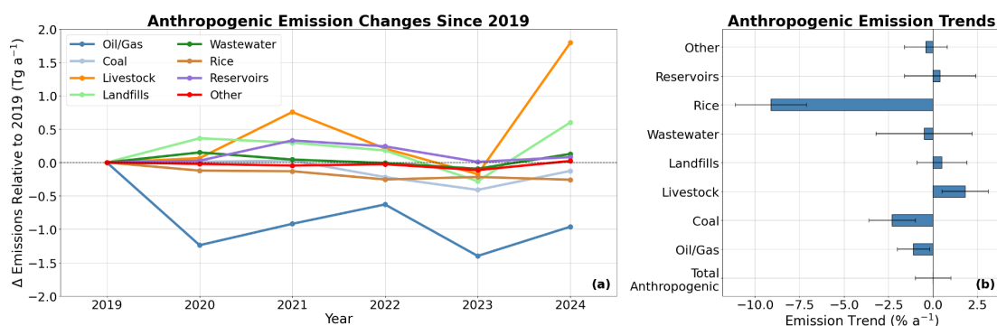
Figure 3. Changes in CONUS anthropogenic methane emissions relative to 2019 and trends by sector, 2019–2024. Values show the change in the annual mean posterior estimates relative to 2019. Trends are derived from ordinary least squares regression of emissions for individual years, and error bars are the standard error.
