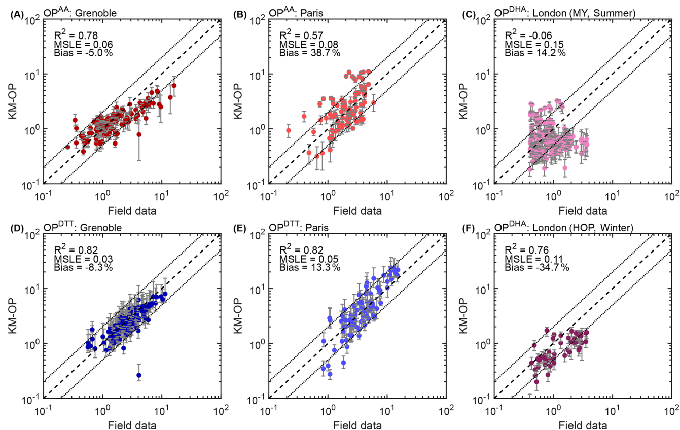
Figure 7. Correlation scatter plots of model-predicted and measured OP for particulate matter samples collected in three different sites across Europe: Grenoble (OP AA : A, and OP DTT : D), Paris (OP AA : B, and OP DTT : E), and OP DHA in London during the summer (C) and during the winter (F). Data shown in blue indicate OP DTT (in units of \text{nmol min}^{-1} \text{m}^{-3} ), while the red and pink data show OP AA (in units of \text{nmol min}^{-1} \text{m}^{-3} ) and OP DHA (in units of \text{nmol min}^{-1} \text{m}^{-3} ). The dashed lines indicate the 1 : 1 line. The dotted lines indicate the 2 : 1 and 1 : 2 lines. The error bars indicate the maximum and minimum values from the ensemble fits.
