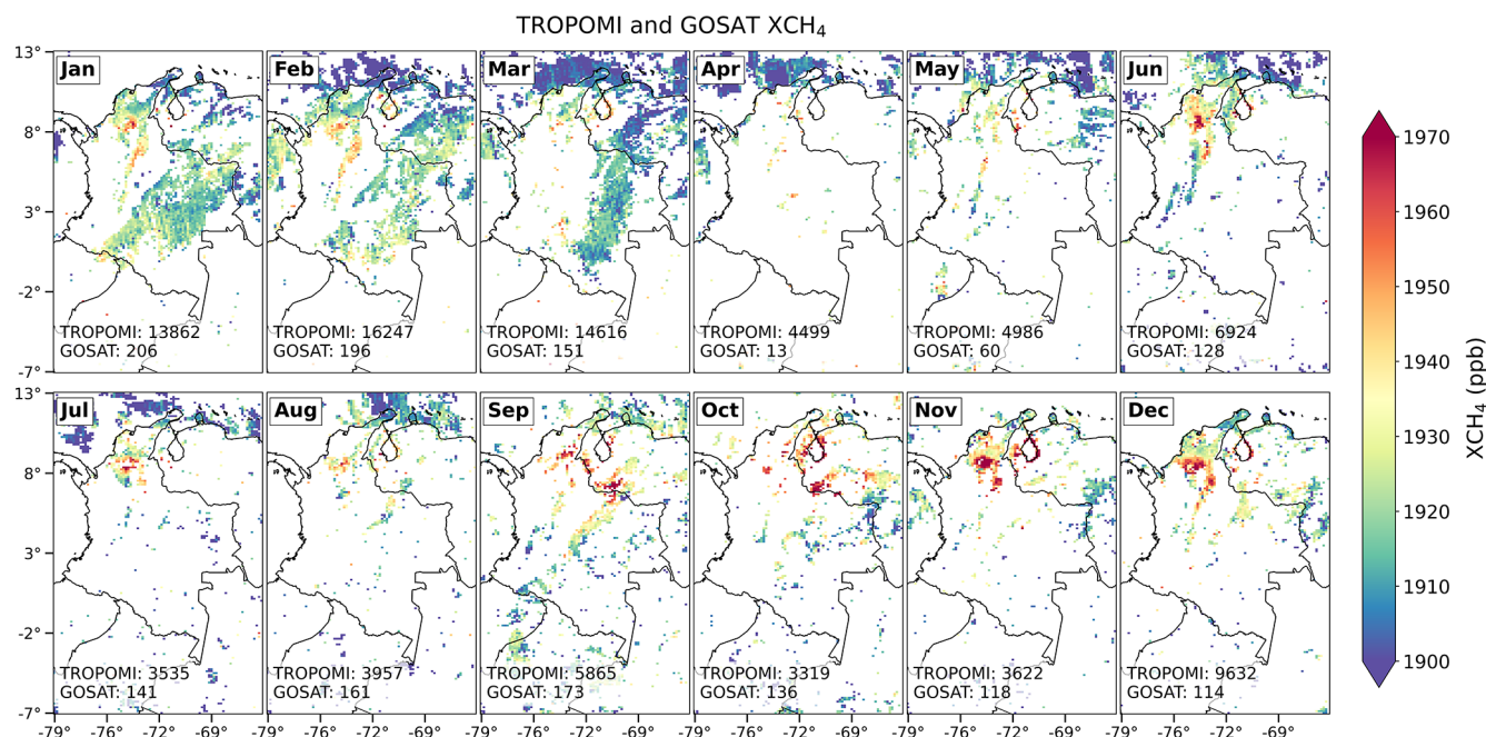
Figure 5. Atmospheric methane concentrations from TROPOMI and GOSAT over the inversion domain in 2023. Mean dry-column methane mixing ratios (XCH 4 ) are shown on the native inversion grid ( 0.125^\circ \times 0.15625^\circ ) for each month, with the number of observations given in each panel.
