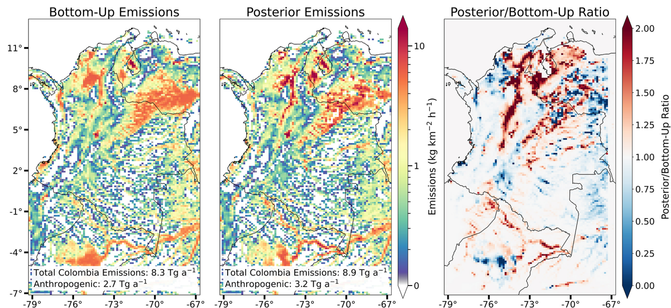
Figure 6. Optimization of 2023 methane emissions over Colombia on the 0.125^\circ \times 0.15625^\circ grid. Prior bottom-up emissions for Colombia are as given in Table 1 and shown in Fig. 3 for anthropogenic sectors and Fig. 4 for wetlands (GLWD + LPJ). Anthropogenic emissions outside Colombia are from GFEIv3 for fuel, EDGARv7 for livestock, ResME for hydroelectric reservoirs, and EDGARv8 for all other sectors. Posterior emissions are from our base inversion of TROPOMI observations. Total Colombia emissions and their anthropogenic component are inset. The right panel gives the ratio of posterior to prior bottom-up emissions. Grid cells with near-zero bottom-up emissions are shown in white in all panels.
