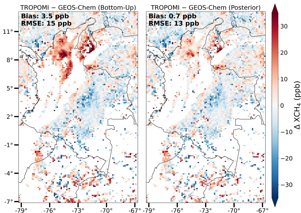
Figure 7. Differences between methane dry-column mixing ratios ( \Delta\text{XCH}_4 ) observed by TROPOMI and simulated by GEOS-Chem with bottom-up emissions (left panel) and posterior emissions (right panel). The mean bias and root-mean-square errors (RMSEs) are given inset. Grid cells with no satellite observations are shown in white.
