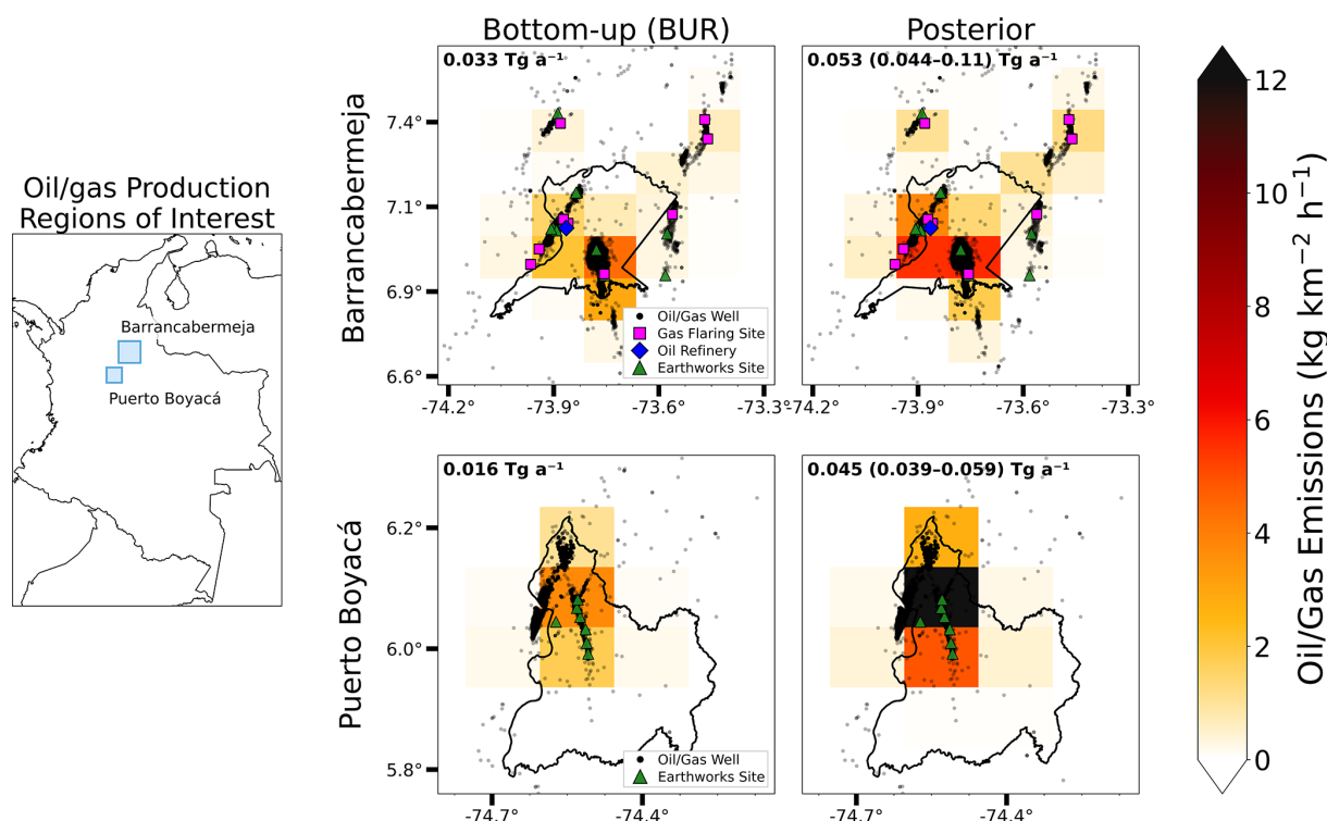
Figure 11. Bottom-up (BUR) and posterior oil/gas emissions in the oil production regions of Barrancabermeja and Puerto Boyacá that account for 82 % of the national upward adjustment to oil/gas emissions in the inversion. Totals shown are for all oil/gas emissions in each domain (6.6 to 7.6° latitude, -74.25 to -73.25^\circ longitude for Barrancabermeja, 5.7 to 6.4° latitude, -74.8 to -74.1^\circ longitude for Puerto Boyacá). Black dots, pink squares, and blue diamonds indicate the locations of wells, gas flaring sites, and oil refineries, respectively, identified from the OGIM database (Omara et al., 2023). Green triangles indicate the locations of leaking, venting, or flaring infrastructure documented by Earthworks using shortwave infrared (SWIR) cameras (Earthworks, 2023).
