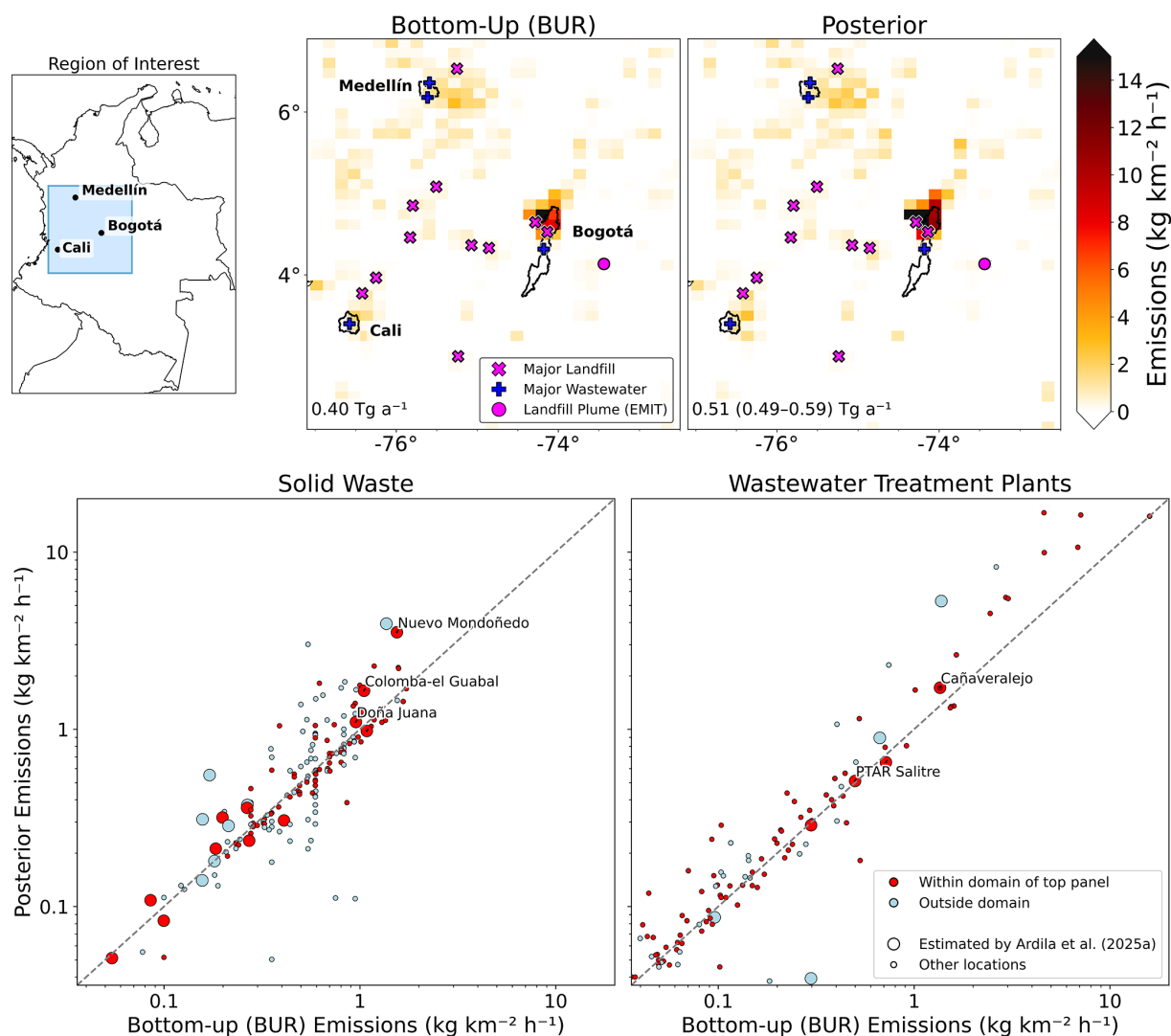
Figure 10. Emissions from solid waste and wastewater treatment plants in Colombia on the 0.125^{\circ} \times 0.15625^{\circ} grid of the inversion. The top panels show bottom-up (BUR) and posterior emissions for the west-central region including Bogotá, Medellín, and Cali, which accounts for 65 % of national posterior emissions. Pink and blue crosses and pluses mark major landfills and wastewater treatment plants, respectively, identified by Ardila et al. (2025a); a pink dot indicates a landfill plume observed by EMIT. Region totals inset represent all waste emissions in the plotted domain ( 2.1 to 6.9^{\circ} latitude, -77.1 to -72.5^{\circ} longitude), with parentheses indicating the range across the inversion ensemble. The bottom panels are scatterplots of posterior versus bottom-up solid waste and wastewater emission estimates for individual grid cells, generally representing individual facilities. Facilities with emissions estimated by Ardila et al. (2025a) have larger symbols; additional sites from the Superintendent of Public Services and EDGARv8 are shown in red (if within the Bogotá–Medellín–Cali domain) or light blue (if outside). Major Ardila et al. (2025a) facilities within the Bogotá–Medellín–Cali domain with emissions above 0.5 \text{ kg km}^{-2} \text{ h}^{-1} are labeled.
