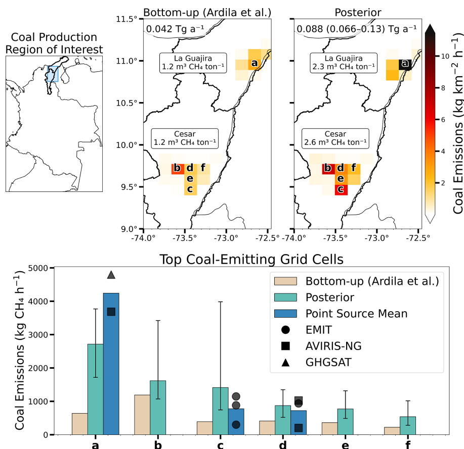
Figure 12. Coal mine emissions in the Cesar and La Guajira departments. Posterior emissions on the 0.125^\circ \times 0.15625^\circ inversion grid are compared to the Ardila et al. (2025a) bottom-up inventory, which updates the BUR to account for declining coal production, and to point source observations. All emissions are from open-pit mines. The letters (a–f) shown on the maps correspond to the locations of the emissions shown on the bottom panel bar chart. Error bars on the posterior estimates show the ranges across the inversion ensemble. The blue bars indicate the means of multiple point source observations in a grid cell.
