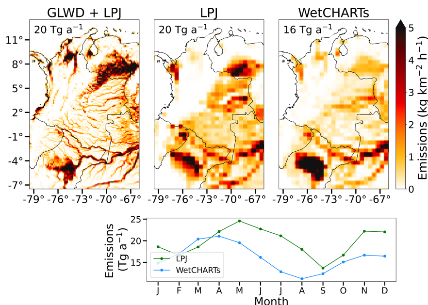
Figure 4. Bottom-up wetland emission estimates from GLWD + LPJ, LPJ, and WetCHARTs. LPJ is driven by meteorological data from NASA MERRA-2 for 2023 (Zhang et al., 2018). WetCHARTs is the 2010–2019 mean from the nine high-performance members (Ma et al., 2021). GLWD + LPJ is on the \sim 12 \times 12 \text{ km}^2 grid of the inversion, while LPJ and WetCHARTs are on a \sim 50 \times 50 \text{ km}^2 grid. The bottom panel shows the mean LPJ and WetCHARTs seasonalities of emissions for the domain shown in the Figure.
