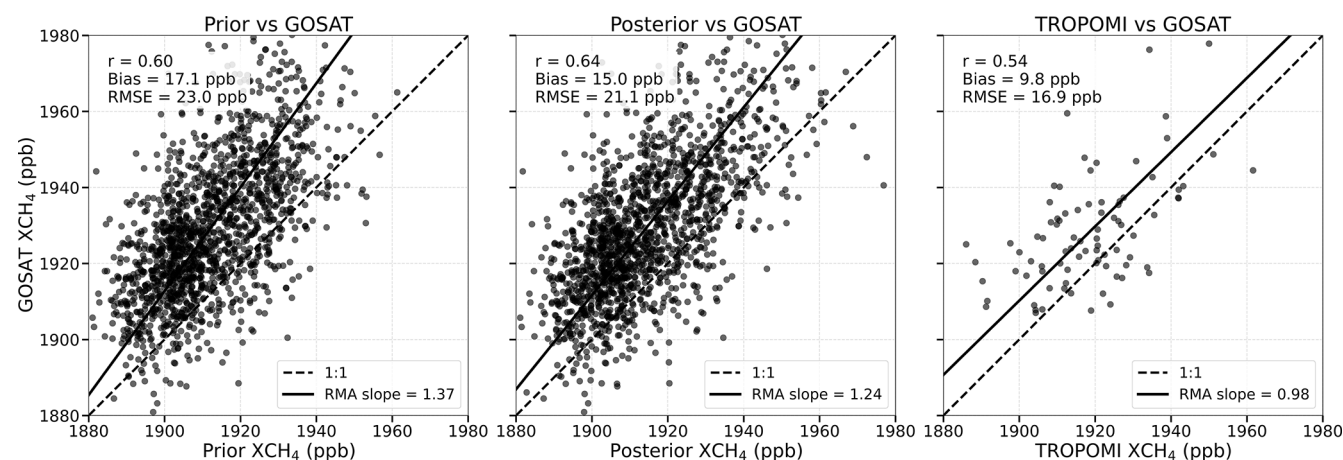
Figure 8. Comparison of GOSAT \text{XCH}_4 observations over the inversion domain with collocated prior simulation \text{XCH}_4 (left), posterior simulation \text{XCH}_4 constrained by TROPOMI observations (center), and TROPOMI \text{XCH}_4 observations (right). For comparison with GOSAT, the prior and posterior simulations were sampled using the GOSAT observation operator. Dashed lines show the 1 : 1 relationship and solid lines show reduced major axis (RMA) regressions. Correlation coefficients, mean biases, and root-mean-square errors (RMSEs) relative to GOSAT are given inset.
