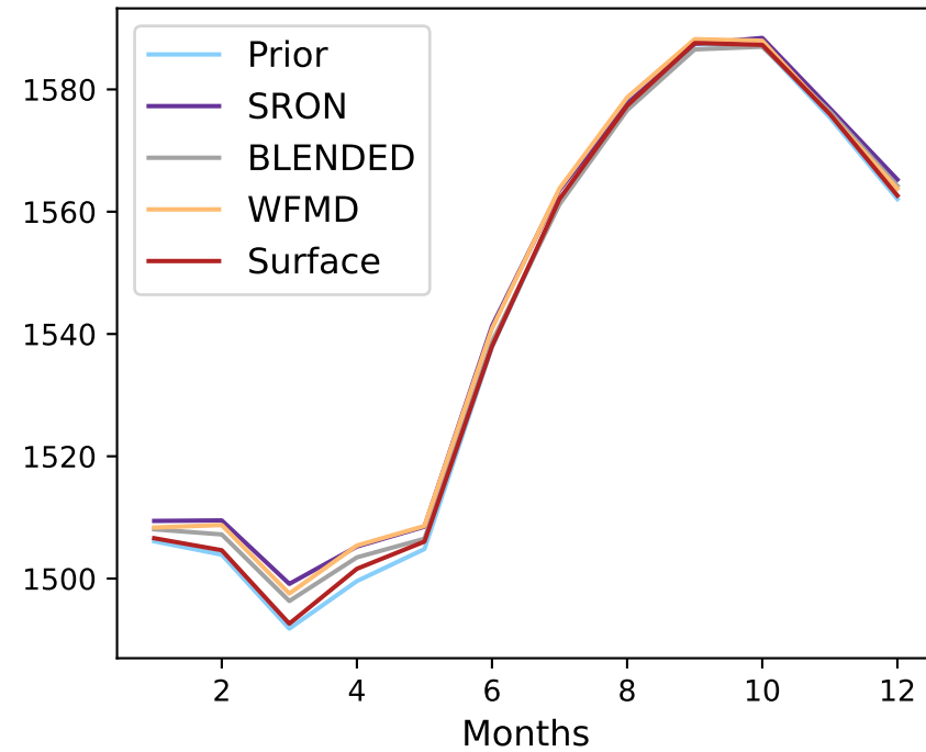
Stratosphere
