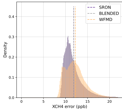
(c) XCH 4 error after scaling
