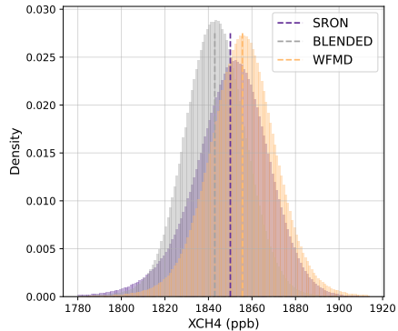
(a) XCH 4 total column
