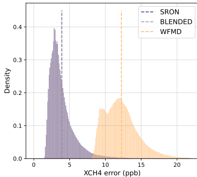
(b) XCH 4 error before scaling
