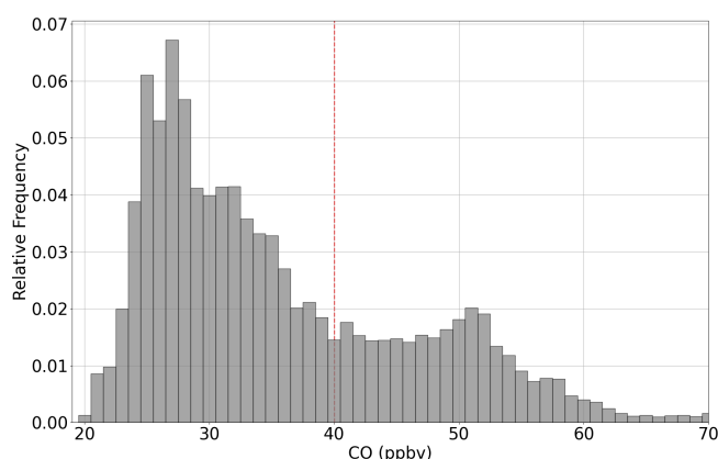
Figure 3. The relative frequency distribution of CO mixing ratios is based on data from all flights. Only data points with an \text{N}_2\text{O} threshold of < 336 ppbv for stratospheric signatures (Riese et al., 2025) were considered. The distribution exhibits two distinct regimes. A CO value of approximately 40 ppbv (red dashed line) was chosen as a practical separation point between these regimes. This threshold is consistent with the visual minimum between the two distributions and aligns well with ranges reported in previous studies (e.g., Müller et al., 2016). This threshold was used to differentiate between the undisturbed and polluted lower stratospheric air mass.
