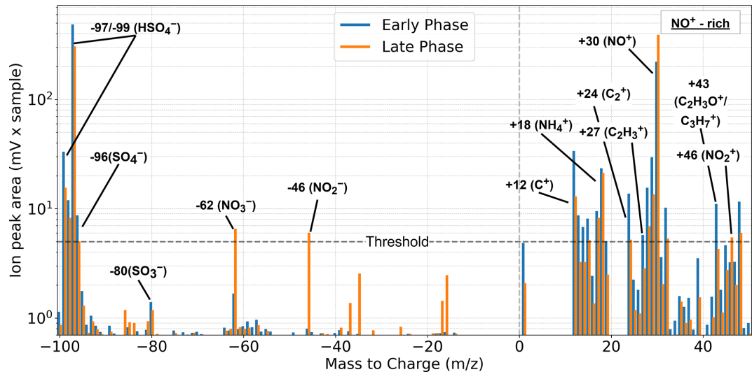
Figure 2. Bipolar mean spectra of the ERICA-LAMS NO + -rich particle type: Comparison between the Early and Late Phases. The Early Phase average is based on 1302 NO + -rich particles, whereas the Late Phase average includes 9182 NO + -rich particles. In total, 10 484 NO + -rich particles out of 37 401 analyzed aerosol particles were considered for this study, all of which were included in the ExLS background air mass during the Early and Late Phase. Further detailed information about the classification and threshold (5 mV · samples) of the spectra is given in the Supplement Sect. S3.2 and S3.3.
