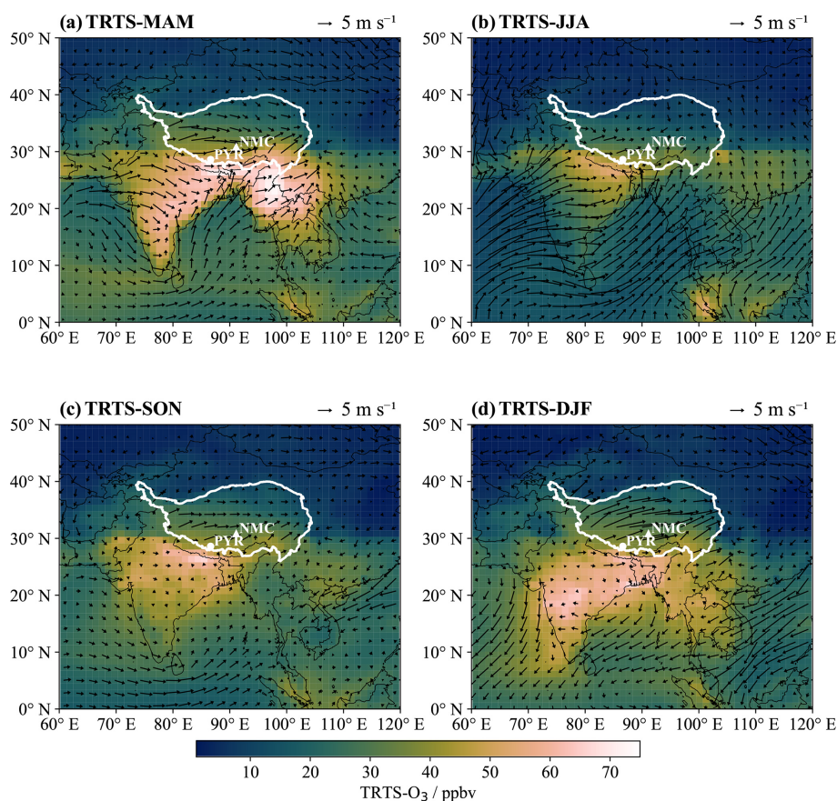
Figure 8. EMAC simulated regional distributions of surface TRTS- \text{O}_3 and boundary layer average wind field over a larger area covering the Tibetan Plateau, South Asia, and Southeast Asia in different seasons averaged over the period 2010–2012: (a) Spring, (b) Summer, (c) Autumn, (d) Winter. Color shading denotes TRTS- \text{O}_3 volume mixing ratio (units: ppbv), and black arrows represent the wind field (units: \text{m s}^{-1} ). White lines highlight the Tibetan Plateau area, and white dots mark the locations of the PYR (circle) and NMC (triangle) stations.
