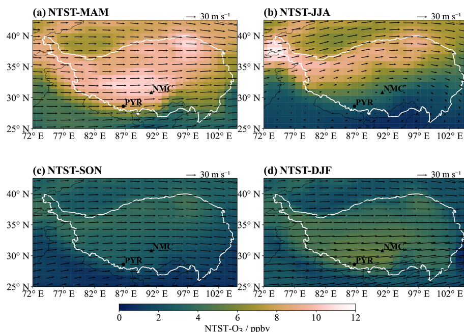
Figure 4. EMAC simulated regional distributions of surface NTST- \text{O}_3 and 200 hPa wind field over the Tibetan Plateau in different seasons during 2010–2012: (a) Spring, (b) Summer, (c) Autumn, (d) Winter. Color shading denotes NTST- \text{O}_3 volume mixing ratio (units: ppbv), and black arrows represent the wind field (units: \text{m s}^{-1} ). White lines refer to the 3 km terrain height contour, highlighting the Tibetan Plateau area. White dots mark the locations of the PYR (circle) and NMC (triangle) stations.
