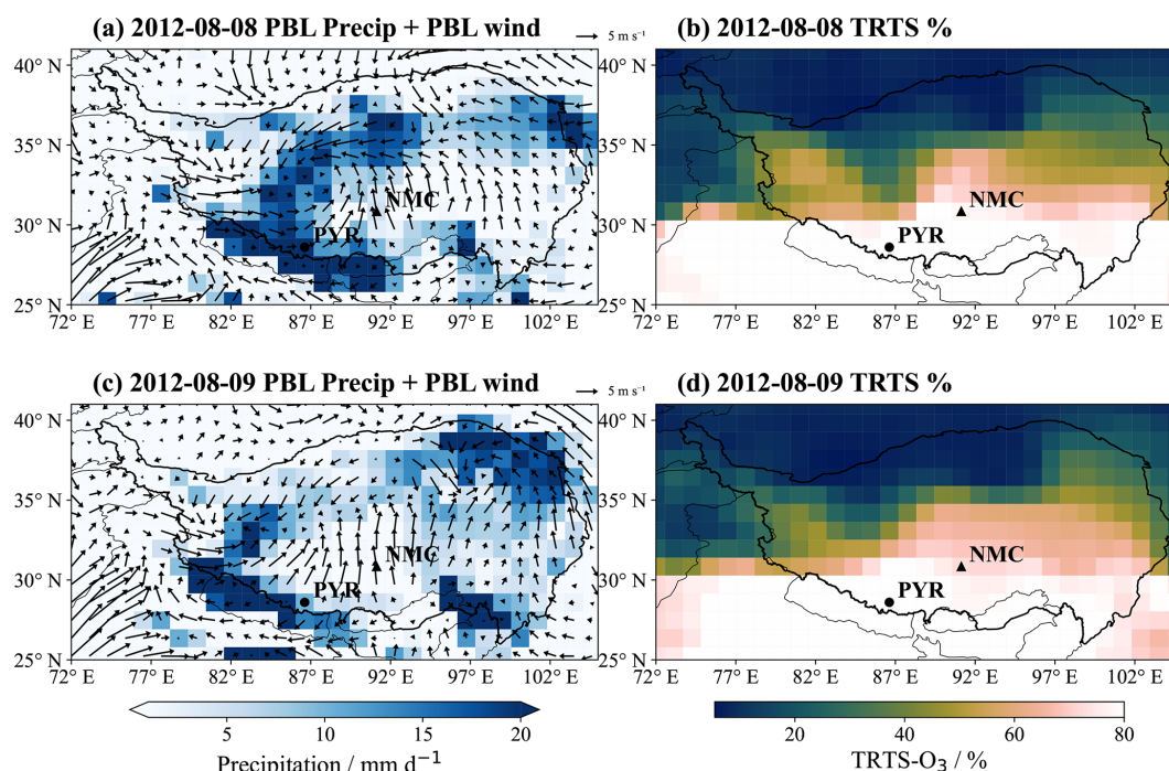
Figure 11. EMAC simulated changes in the regional distribution of surface TRTS- \text{O}_3 for a typical TRTS- \text{O}_3 transport event during the 2012 Asian summer monsoon: Row 1 ( a , b ) corresponds to 8 August 2012, and Row 2 ( c , d ) corresponds to 9 August 2012. Column 1 ( a , c ) shows the regional distributions of daily accumulated precipitation (color shading, units: \text{mm d}^{-1} ) overlaid with the boundary layer average wind field (arrows, units: \text{m s}^{-1} ). Column 2 ( b , d ) presents the regional distributions of surface TRTS- \text{O}_3 (units: ppbv). Black lines highlight the Tibetan Plateau area, and black dots mark the locations of the PYR (circle) and NMC (triangle) stations.
