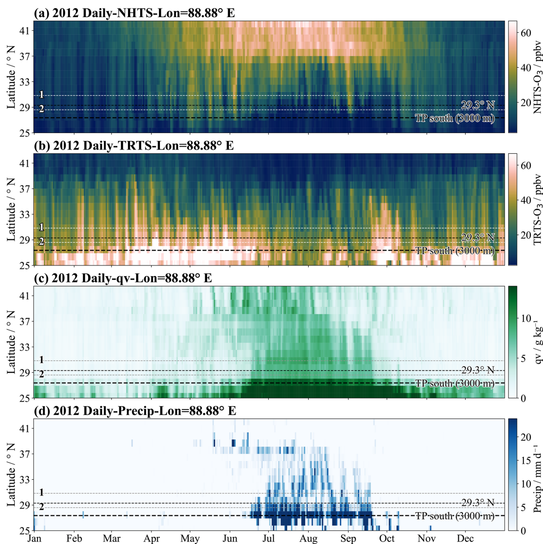
Figure 9. Time series of daily average surface (a) NHTS- \text{O}_3 mixing ratio (units: ppbv), (b) TRTS- \text{O}_3 mixing ratio (units: ppbv), (c) specific humidity ( q_v , units: \text{g kg}^{-1} ), and (d) precipitation (units: \text{mm d}^{-1} ) over the Tibetan Plateau at 88.88^\circ \text{E} longitude (the midpoint of the longitudes of the two stations, NMC and PYR) in 2012, simulated by the EMAC model. The latitude 29.3^\circ \text{N} (the boundary between the NHTS and TRTS source regions) is marked by a black dashed line, and dashed gray lines with numbered labels indicate the latitudes of the two stations (with “1” for NMC and “2” for PYR). The thick black dashed line indicates the southern boundary of the Tibetan Plateau at this longitude.
