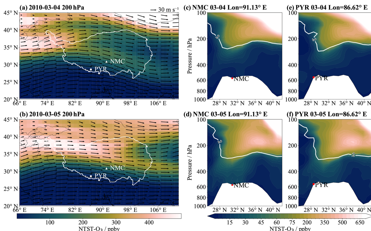
Figure 5. Upper-level tracer distribution and vertical dynamical structure of a stratospheric intrusion event in spring 2010 simulated by the EMAC model: Row 1 ( a , c , e ) corresponds to 4 March 2010, and Row 2 ( b , d , f ) corresponds to 5 March 2010. Column 1 ( a , b ) shows the regional distributions of NTST-O 3 at 200 hPa (color shading) overlaid with wind fields (arrows); White lines highlight the Tibetan Plateau area, and white dots mark the locations of the PYR (circle) and NMC (triangle) stations. Column 2 ( c , d ) and Column 3 ( e , f ) present the meridional cross-sections of NMC (Lon = 91.13° E) and PYR (Lon = 86.62° E), respectively; thick white solid lines denote 2 PVU isopleths, red dots indicate the station locations, and color shading represents NTST-O 3 volume mixing ratio (units: ppbv).
