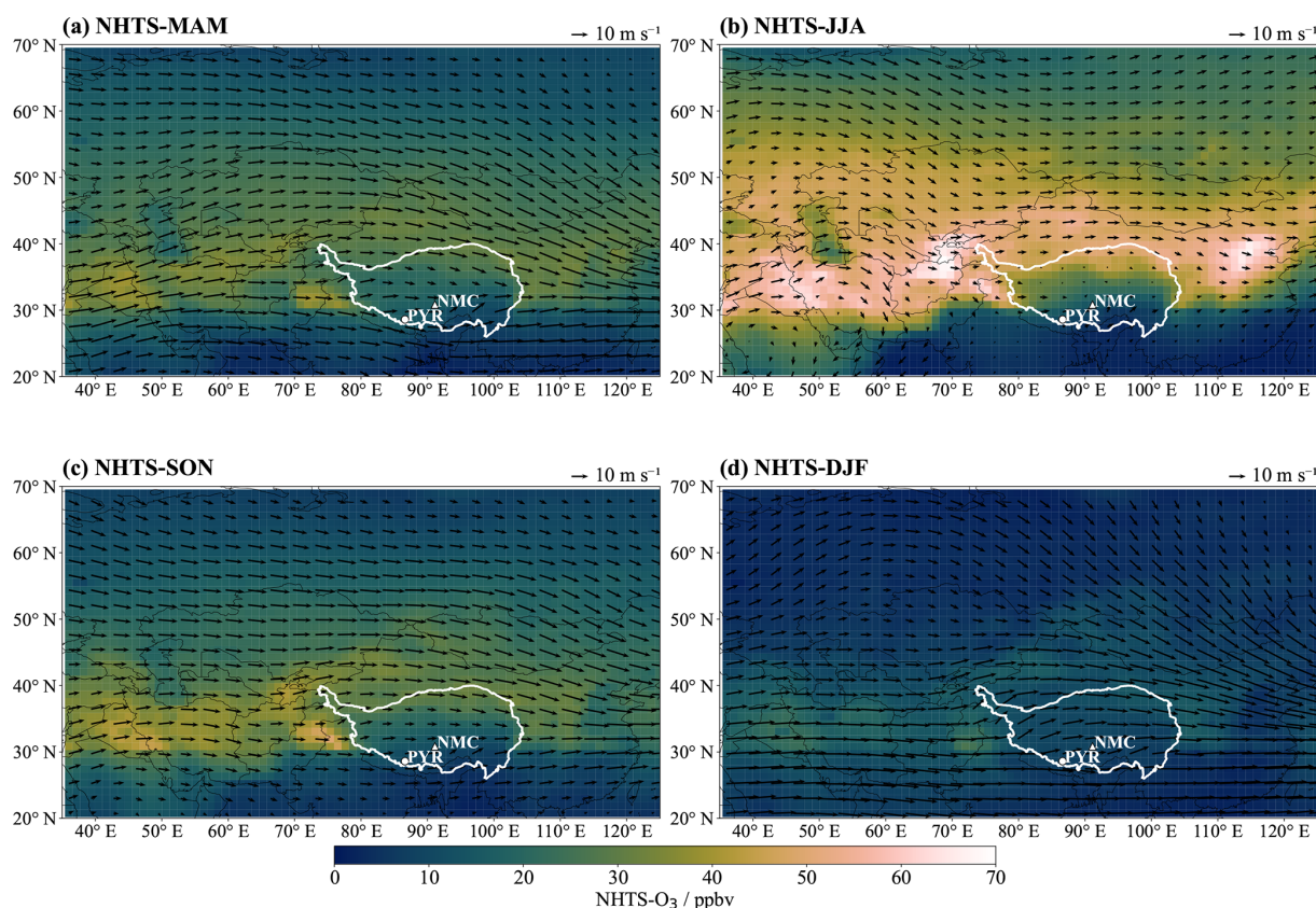
Figure 7. EMAC simulated regional distributions of surface NHTS- \text{O}_3 and 500 hPa wind field over parts of Eurasia ( 35\text{--}125^\circ\text{E} , 20\text{--}70^\circ\text{N} ) in different seasons averaged over the period 2010–2012: (a) Spring, (b) Summer, (c) Autumn, (d) Winter. Color shading denotes NHTS- \text{O}_3 volume mixing ratio (units: ppbv), and black arrows represent the wind field (units: \text{m s}^{-1} ). White lines highlight the Tibetan Plateau area, and white dots mark the locations of the PYR (circle) and NMC (triangle) stations.
