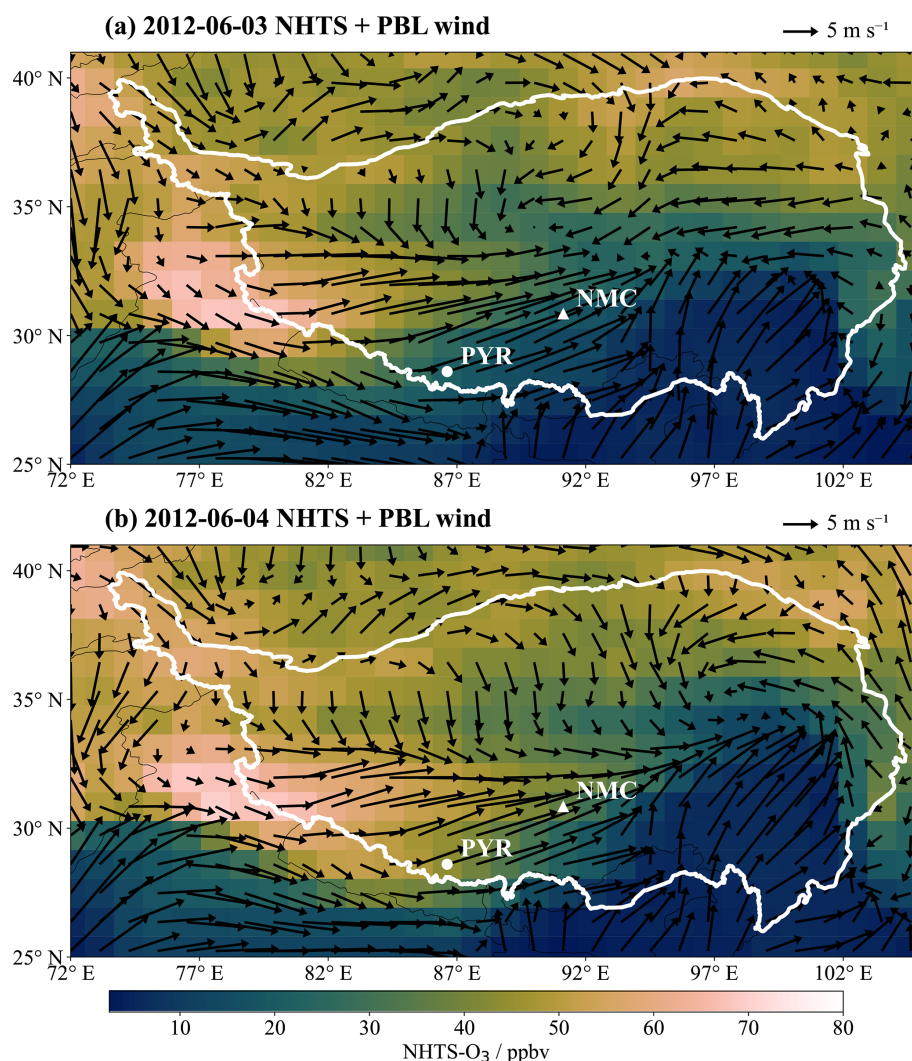
Figure 10. EMAC simulated changes in the regional distribution of surface NHTS- \text{O}_3 (color shading, units: ppbv) and the boundary layer average wind field (arrows, units: \text{m s}^{-1} ) during a typical NHTS- \text{O}_3 transport event over the Tibetan Plateau: (a) corresponds to 3 June 2012, and (b) corresponds to 4 June 2012. White lines highlight the Tibetan Plateau area, and white dots mark the locations of the PYR (circle) and NMC (triangle) stations.
