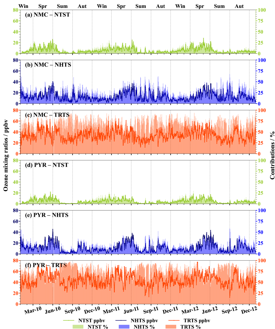
Figure 3. Daily absolute (solid lines) and relative (shaded bars) contributions of O 3 produced in the three source regions (TRTS: red, NHTS: blue, NTST: green) to surface O 3 at NMC (a–c) and PYR (d–f) during 2010–2012, simulated by the EMAC model.
