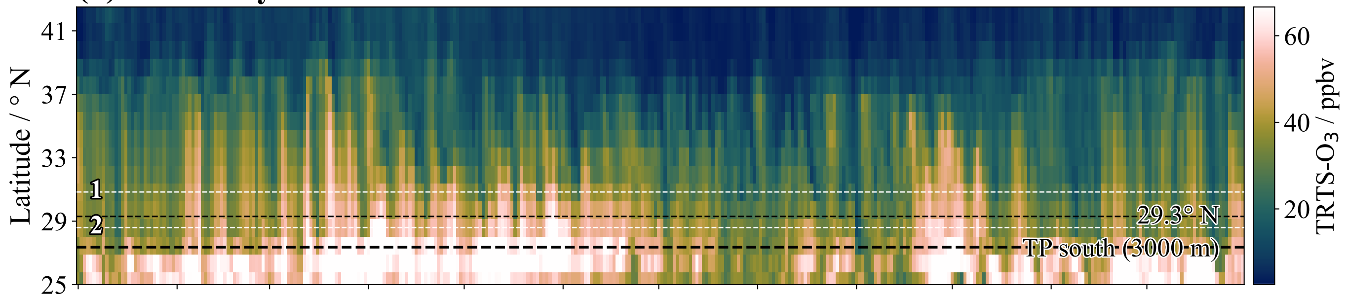
(c) 2012 Daily-qv-Lon=88.88° E
