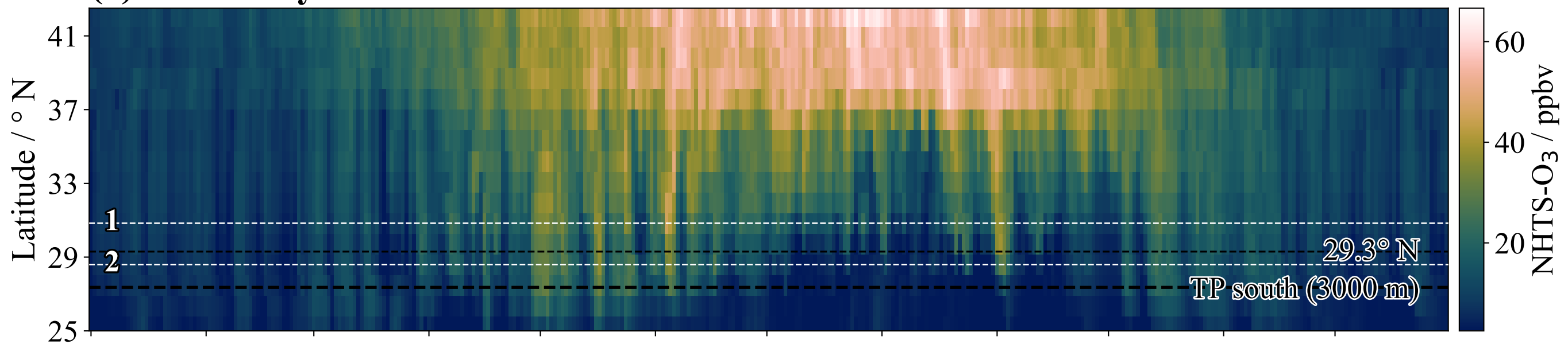
(b) 2012 Daily-TRTS-Lon=88.88° E
