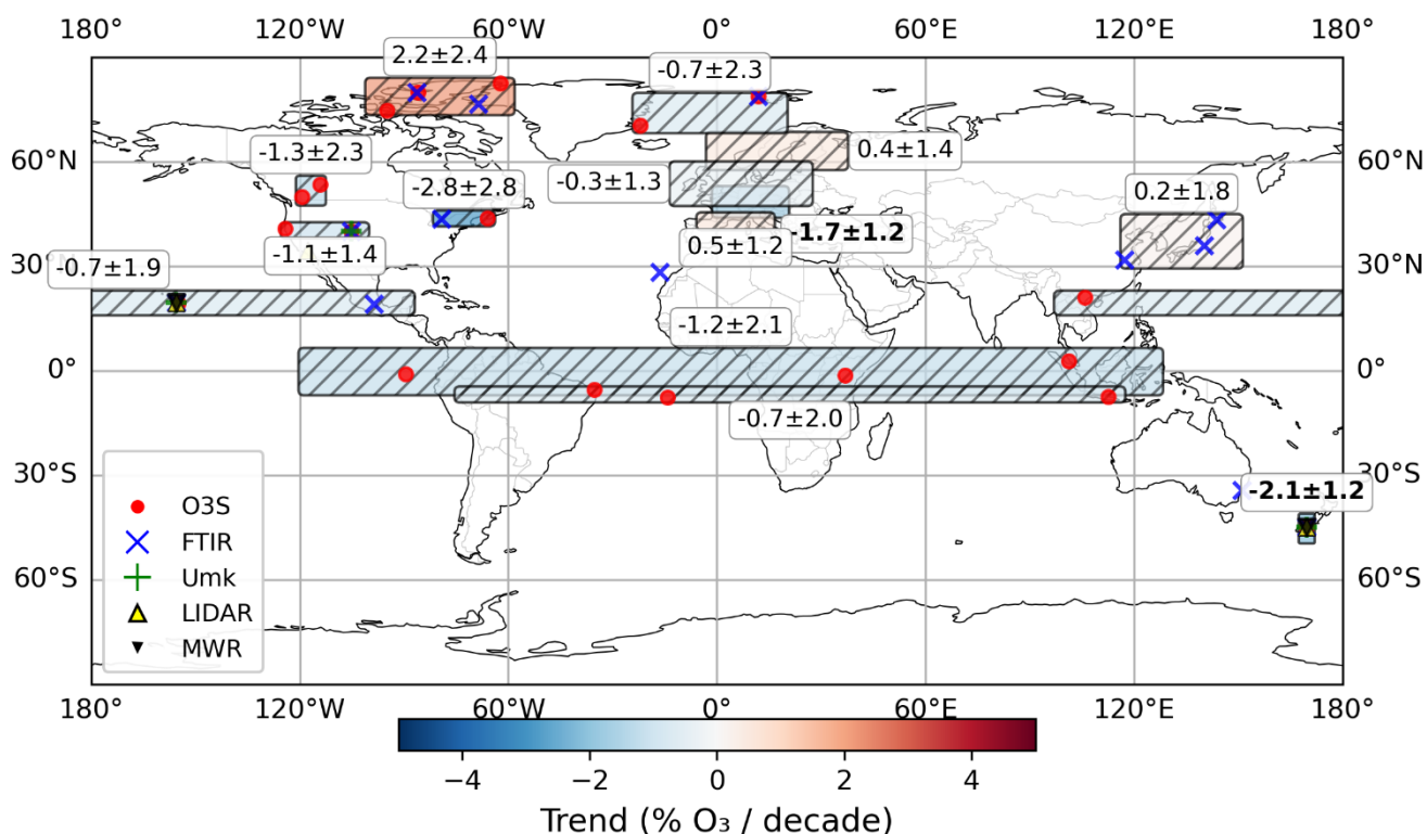
30 Figure S4: Ozone trends for the regional groups in the alternative middle stratosphere (aMS). Bold numbers indicate significant trends. The colour scale indicates the trend magnitude: red for positive and blue for negative values. Regions are hatched where trends are not significant at the 95% confidence level (2 sigma). The locations of the instruments merged into the composite are indicated by markers, except in Europe for readability.
