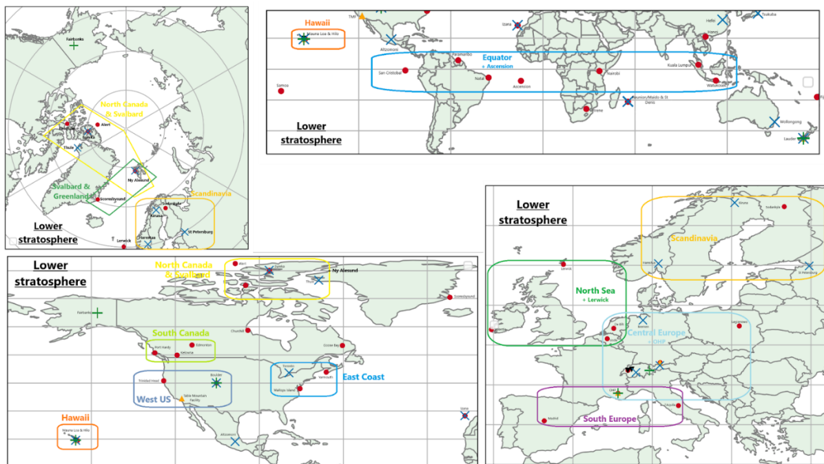
Figure S7: Maps with the groups in LS and UTLS
