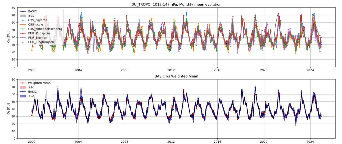
Figure S1: Time series for regional group Central Europe, in TROPO. Top: time series of the group members, plotted with
