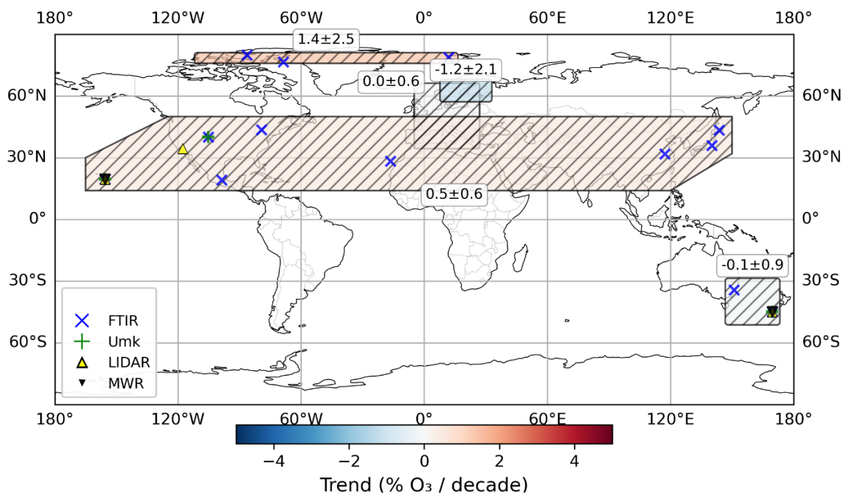
25 Figure S3: Ozone trends for the regional groups in the alternative upper stratosphere (aUpS). Bold numbers indicate significant trends. The colour scale indicates the trend magnitude: red for positive and blue for negative values. Regions are hatched where trends are not significant at the 95% confidence level (2 sigma). The locations of the instruments merged into the composite are indicated by markers, except in Europe for readability.
