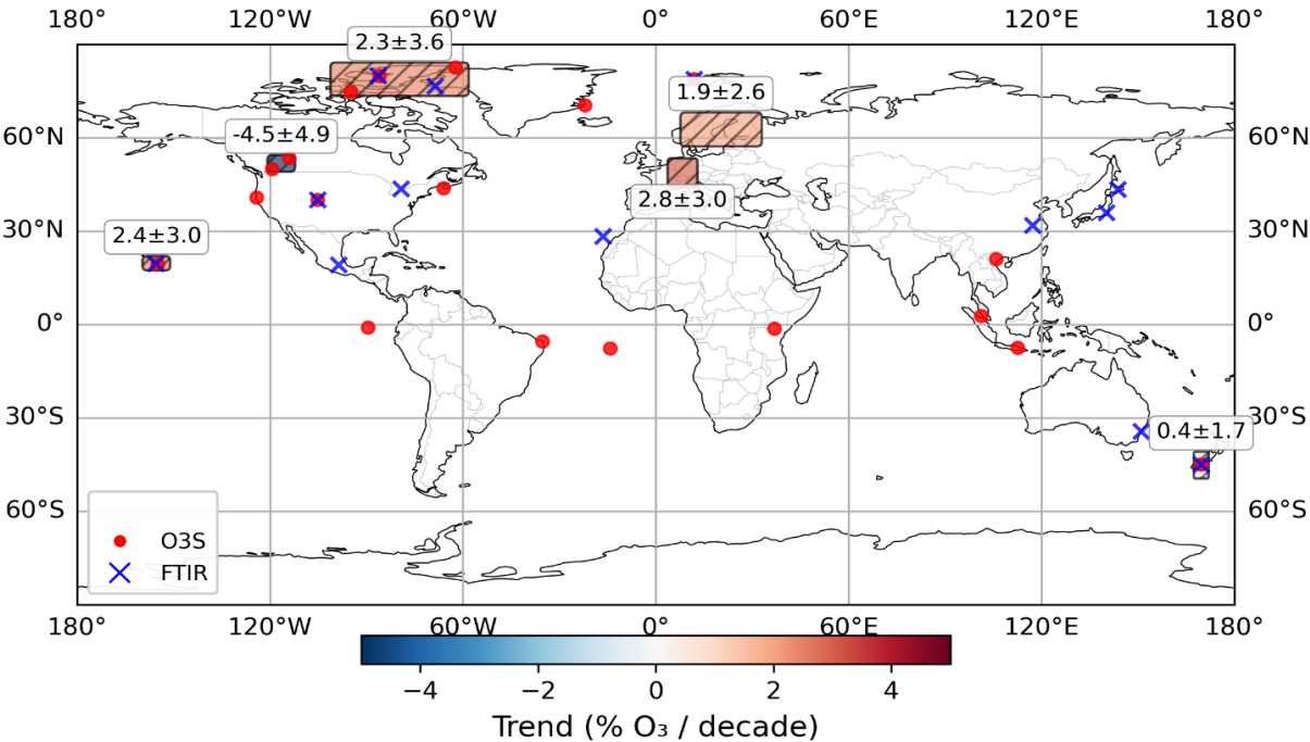
20 Figure S2: Ozone trends for the regional groups in the troposphere (TROPO). Bold numbers indicate significant trends. The colour scale indicates the trend magnitude: red for positive and blue for negative values. Regions are hatched where trends are not significant at the 95% confidence level (2 sigma). The locations of the instruments merged into the composite are indicated by markers, except in Europe for readability.
