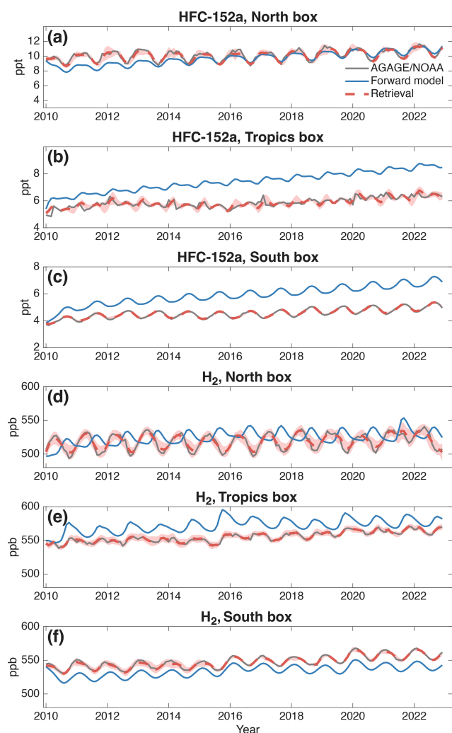
Figure 3. Comparison of the forward model (blue line), observations (gray line), and the retrieval fit (dashed red line) of HFC-152a and H 2 over 2010–2022. HFC-152a for the North box (20–90° N), Tropics box (20° S–20° N), and South box (20–90° S) are shown in panels (a), (b), and (c) respectively. Similarly, for H 2 in panels (d), (e), and (f). The retrieved fit is shown for the 35 % prior uncertainty case along with the posterior standard deviation (shaded region). For the North and South boxes, AGAGE data is used for both HFC-152a and H 2 . For the Tropics box, AGAGE Cape Matatula data is used for HFC-152a, and NOAA data is used for H 2 (see Sect. 2).
