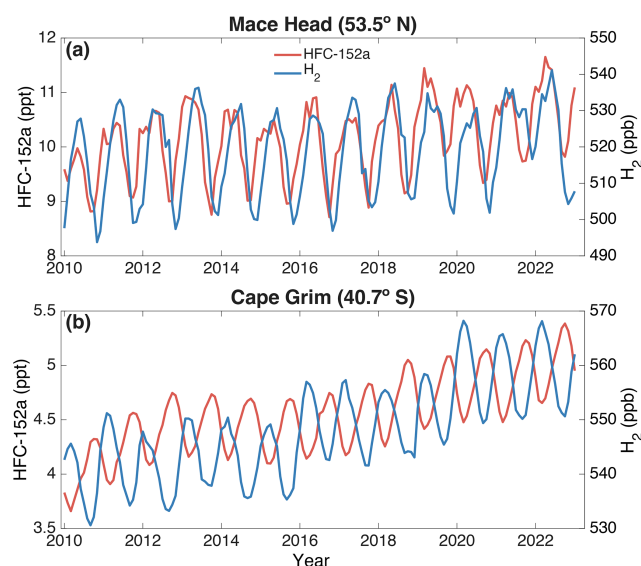
Figure 1. Comparison of HFC-152a and \text{H}_2 AGAGE time series at (a) Mace Head and (b) Cape Grim highlighting the different seasonal cycles and interhemispheric gradients.
