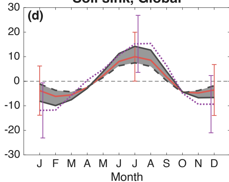
Soil sink, Global
