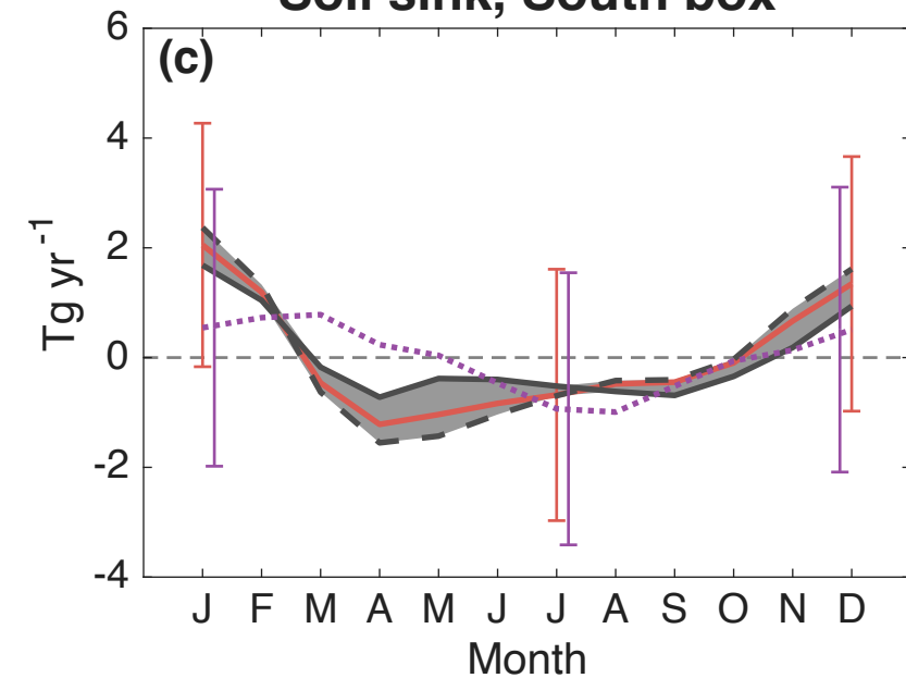
Soil sink, South box
