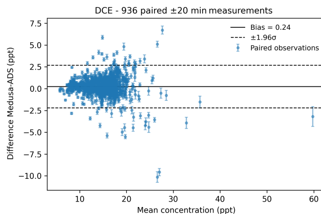
Figure D3. Blant–Alman plot showing the difference between temporally matched ( \pm 20 min) 1,2-dichloroethane (DCE) measurements using the Monte Cimone (CMN) Medusa-GC/MS and Adsorption Desorption System (ADS), as a function of concentration (mole fraction).
