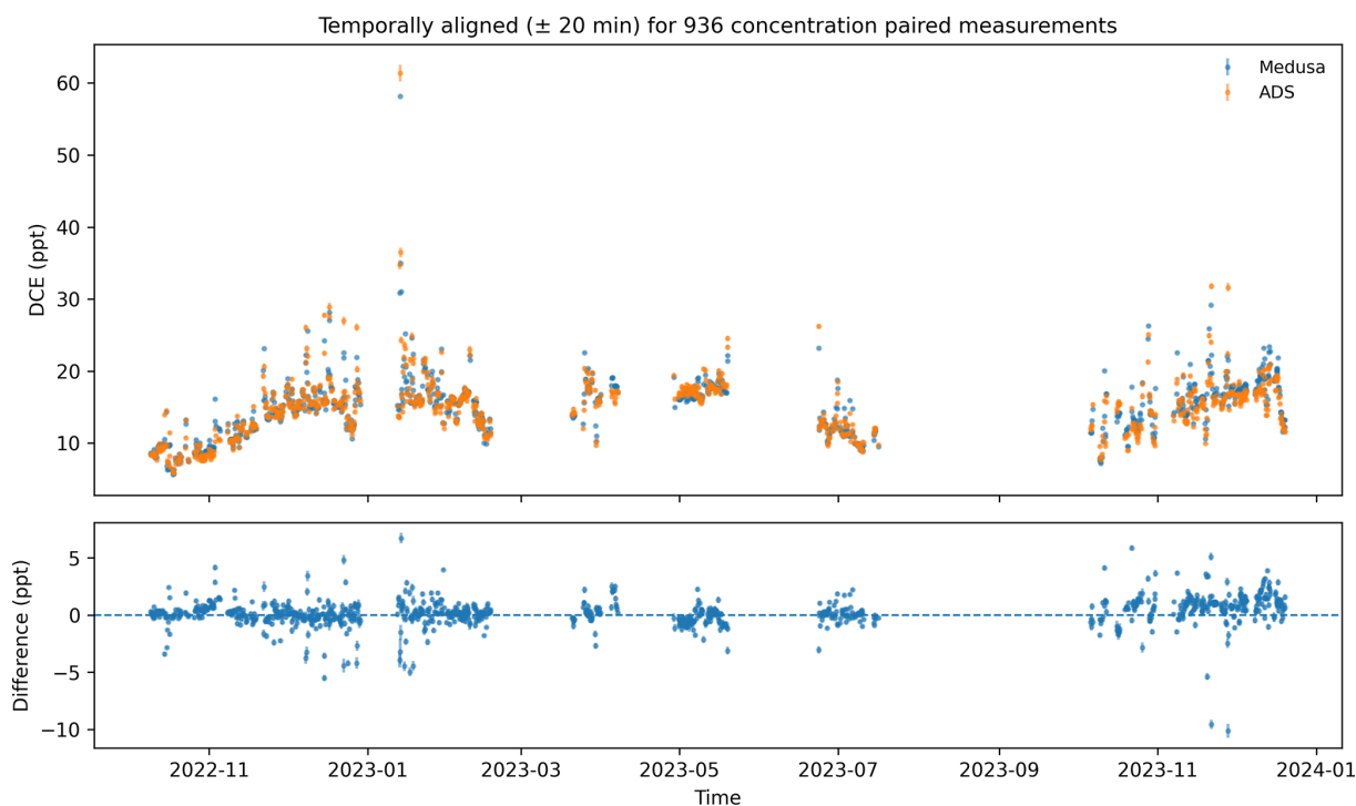
Figure D1. In situ observations of 1,2-dichloroethane (DCE) at Monte Cimone (CMN), Italy, while running two instruments, a Medusa-GC/MS and an Adsorption Desorption System (ADS), in parallel. Temporally matched ( \pm 20 min) measurements are shown, as well as the mole fraction difference between the measurements of the two instruments.
