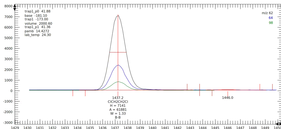
Figure C1. Example chromatogram of DCE, x axis in seconds, y axis in arbitrary units, from the analysis of 2 L of a working standard (18.7 ppt) with a Medusa-GC/MS instrument. The target ion with mass/charge ( m/z ) 62 (black line), and two qualifier ions with m/z 64 (blue line) and m/z 98 (green line) were detected at the retention time of 1437.2 s.
