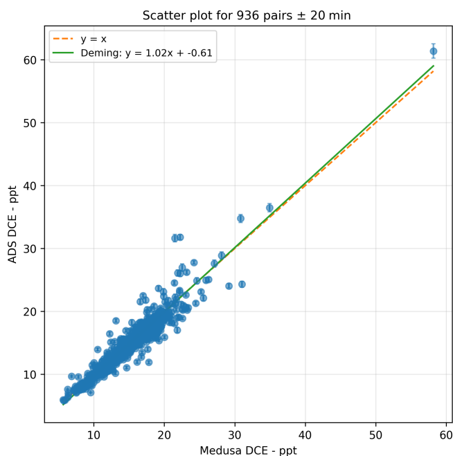
Figure D2. Orthogonal (Deming) regression scatter plot of the temporally matched ( \pm 20 min) in situ measurements of 1,2-dichloroethane (DCE) at Monte Cimone (CMN), Italy, while running two instruments, a Medusa-GC/MS and an Adsorption Desorption System (ADS), in parallel.
