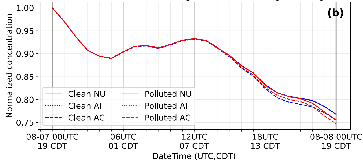
Normalized concentration averaged at 1500 m height in Aug 7 case
