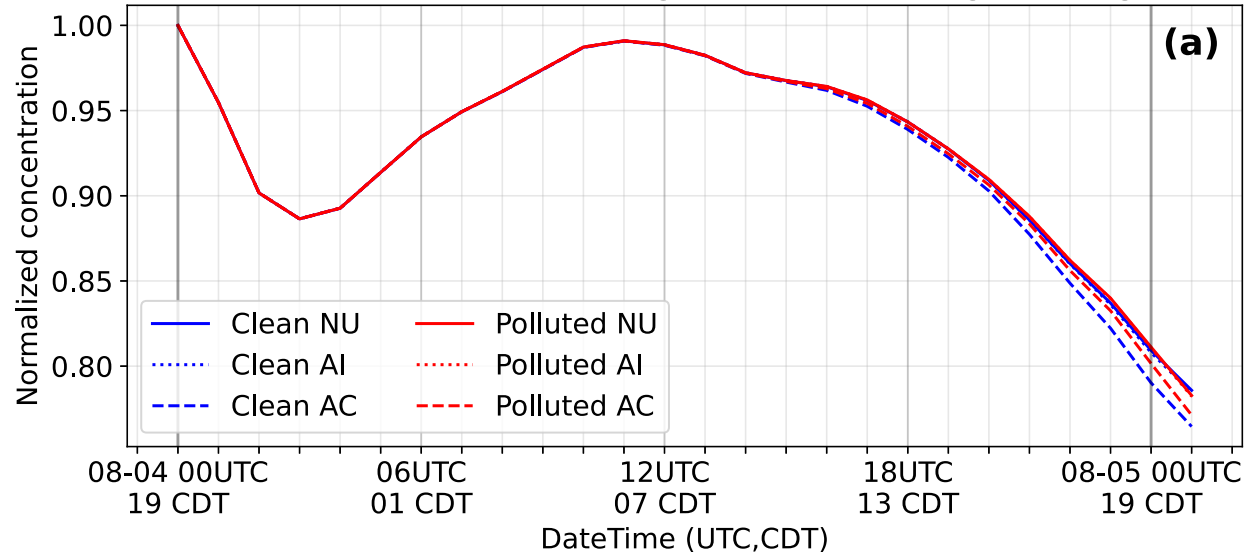
Normalized concentration averaged at 1500 m height in Aug 4 case
