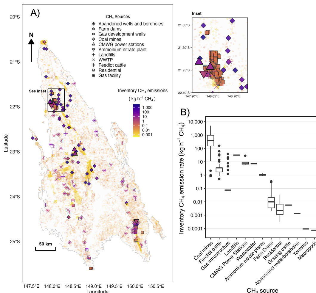
Figure 2. (A) Location and CH 4 emission strength of sources within the UNSW inventory across the Bowen Basin, Queensland, Australia. Sources with non-fixed or spatially diffuse locations (e.g. grazing cattle, termites, macropods, and transportation-related emissions) are included in the UNSW inventory but are not spatially represented. The inset (black box) shows a magnified view of an area of dense source overlap. (B) Distribution of CH 4 emission rates (kg h -1 ) for discrete source categories within the UNSW inventory. Gas infrastructure includes coal seam gas and conventional gas facilities and associated infrastructure. Emission rates for grazing cattle are expressed on a per-head basis, whereas feedlot emissions are reported at the facility scale and therefore vary according to feedlot capacity. Further details on source classification and inventory construction are provided in S2.
