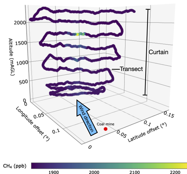
Figure 3. Three-dimensional visualisation of measured downwind \text{CH}_4 enhancements from a flight performed by the in-situ aircraft on 28 September 2023. The red dot marks a quantified coal mine, and the colour bar indicates measured \text{CH}_4 mole fractions downwind of the coal mine.
