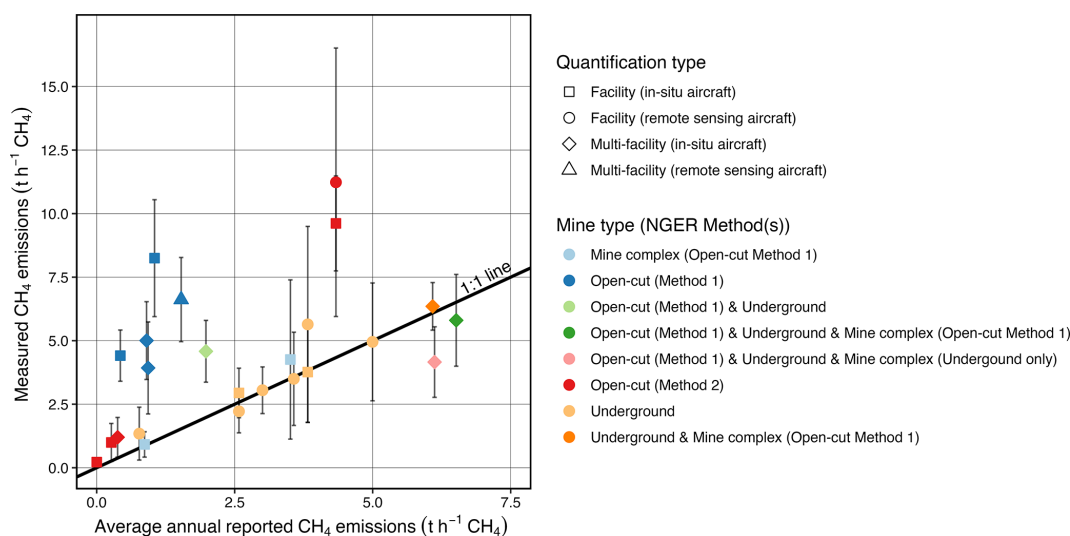
Figure 5. Comparison between mean airborne emission rates and reported mean annual CH 4 emission rates, distinguished by mine type and NGER method. Each data point represents a mean emission rate ( \pm 2\sigma ) estimate derived from one or more quantifications of a single mine or mine grouping (see Table 1 for full details).
