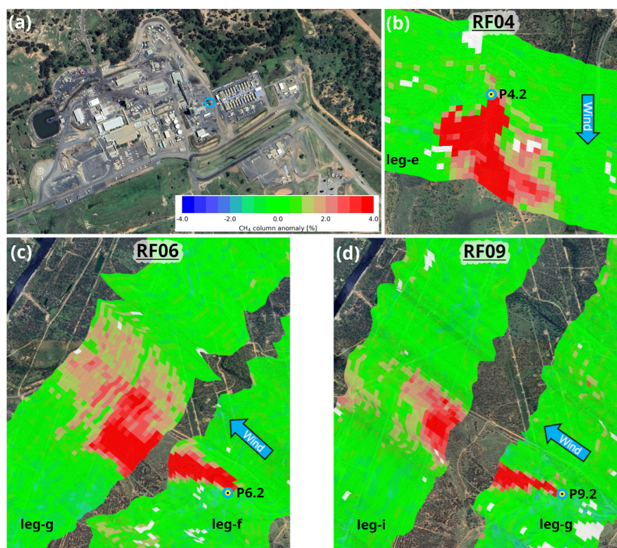
Figure 4. MAMAP2DL \text{CH}_4 column observations over a ventilation shaft (cyan circle). (a) Google Earth imagery showing the shaft location. (b–d) Five of eleven flight legs acquired during research flights on 5, 9, and 16 September 2023, showing downwind \text{CH}_4 plume enhancements. Winds were from the north on 5 September and from the south-east on 9 and 16 September. Base map data © Google, Imagery © 2026 CNES/Airbus.
