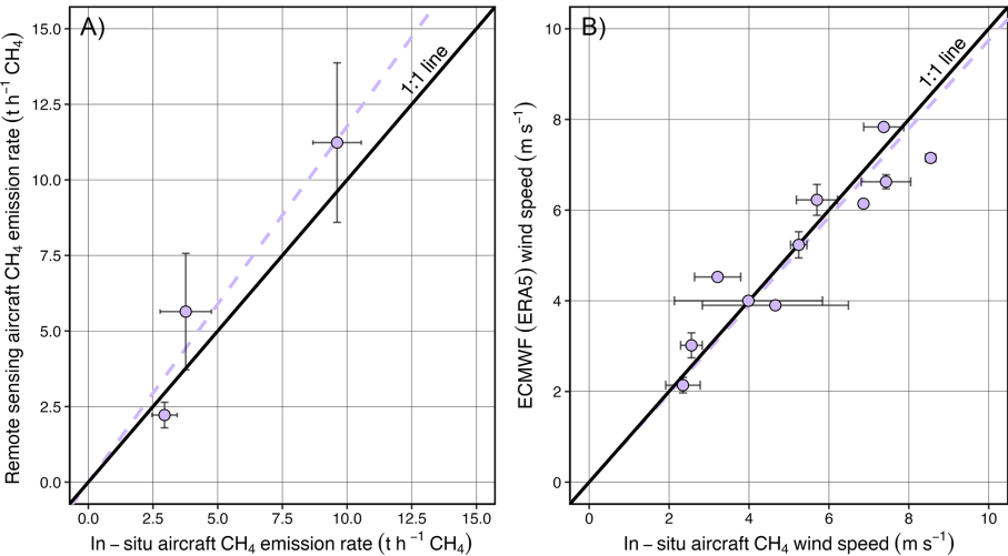
Figure 8. (A) Comparison of remote sensing and in-situ aircraft emission rate estimates from the same coal mine facility. Error bars represent ±1σ uncertainty of each estimate. Data from Borchardt et al. (2025) are used as one of the data points. (B) Comparison of ECMWF (ERA5) modelled wind speeds used in the remote sensing aircraft flux analysis and those measured onboard the in-situ aircraft during the sampling of curtains during the 11 flights undertaken on the same day. Error bars represent 1 standard deviation of mean winds speeds used to model individual quantifications on each day.
