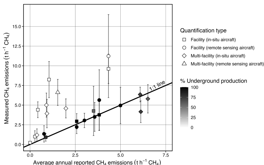
Figure 6. Comparison between mean airborne emission rates and reported mean annual CH 4 emission rates ( \pm 2\sigma ), coloured according to percentage of underground ROM coal production for FY24 (Queensland Government, 2025a; S1).
