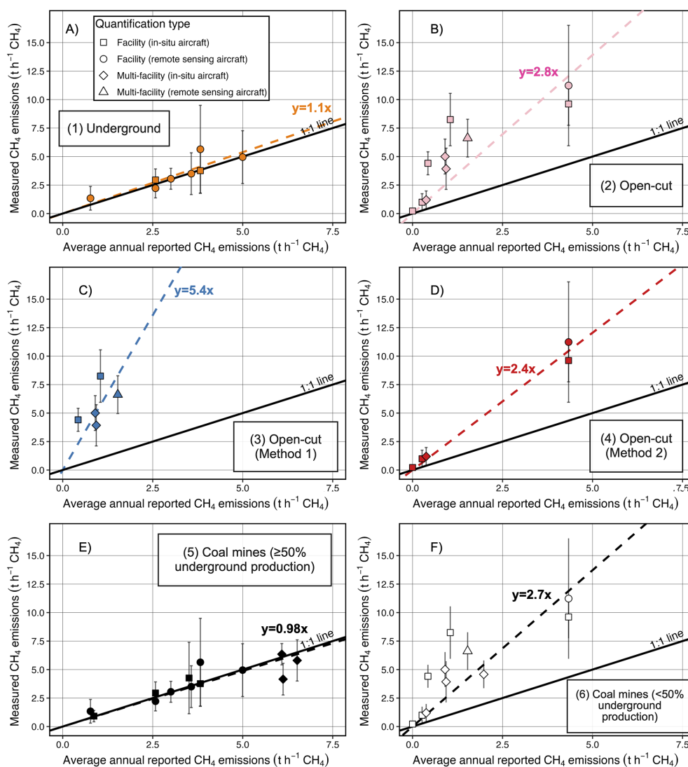
Figure 7. Comparison between mean airborne emission rates ( \pm 2\sigma ) and reported mean annual \text{CH}_4 emission rates for: (A) exclusively underground coal mines; (B) exclusively open-cut coal mines; (C) exclusively open-cut coal mines estimated using Method 1; (D) exclusively open-cut coal mines estimated using Method 2; (E) coal mines with \geq 50\% underground production; and (F) coal mines with < 50\% underground production. The fixed-origin linear regression analysis model is indicated by the dashed line and the slope is indicated in each panel. Symbol shapes are as in Figs. 5 and 6.
