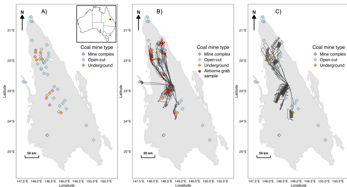
Figure 1. (A) Open-cut, underground and coal mining complexes operational in the Bowen Basin, Australia, during FY24. (B) Flight paths (black lines) and the location of airborne grab samples (red dots) for all in-situ aircraft flights. (C) Flight paths for all remote sensing aircraft flights. Bowen Basin boundary data © Queensland Government (2025b).
