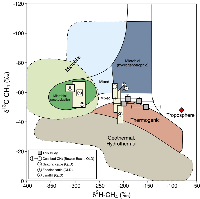
Figure 9. \delta^{13}\text{C-CH}_4 vs \delta^2\text{H-CH}_4 plot after Whiticar (1990) and Haghnegahdar et al. (2023). Coal bed CH 4 data from the Bowen Basin are from Golding et al. (2013; labelled 1), Hamilton et al. (2020; labelled 2), Kinnon et al. (2010; labelled 3) and Draper and Boreham (2006; labelled 4). CH 4 isotopic signatures from grazing cattle (labelled 5), feedlot cattle (labelled 6) in Queensland are taken from Lu et al. (2021). CH 4 isotopic signatures from landfill (labelled 7) are taken from Obersky et al. (2018). Error bars represent the 95 % CI bounds on the Keeling plot intercept.
