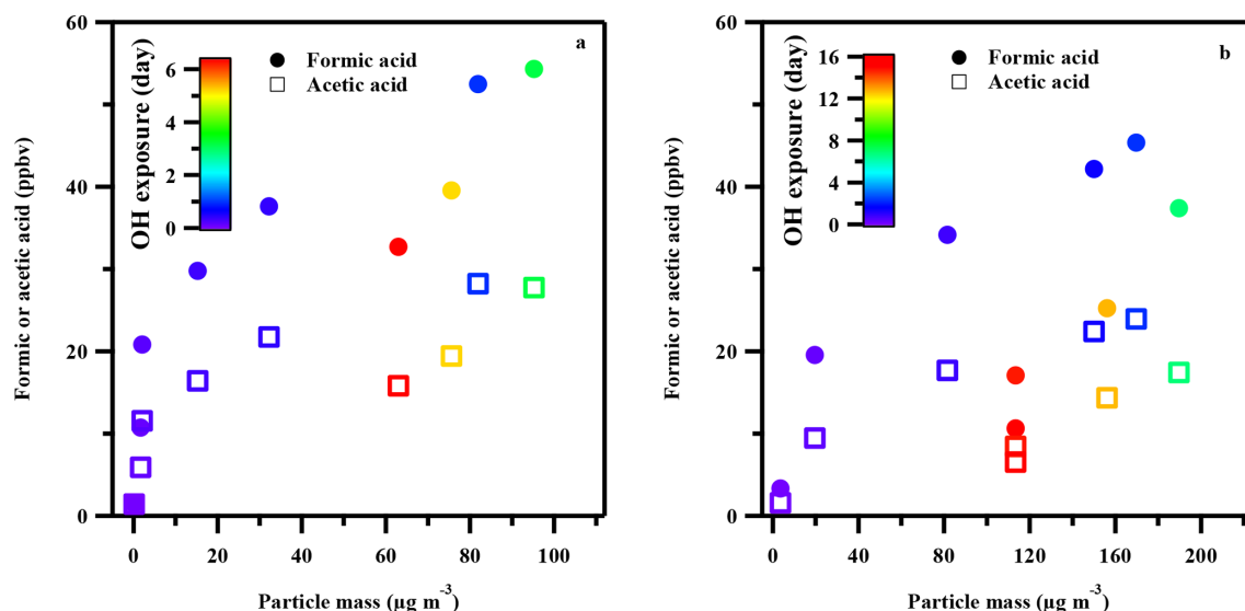
Figure 5. Correlations of particle mass concentration with gas-phase formic acid and acetic acid during the photooxidation of toluene at different \bullet\text{OH} exposure. (a) 20 % RH; (b) 70 % RH. Marker color represents different \bullet\text{OH} exposure levels.
