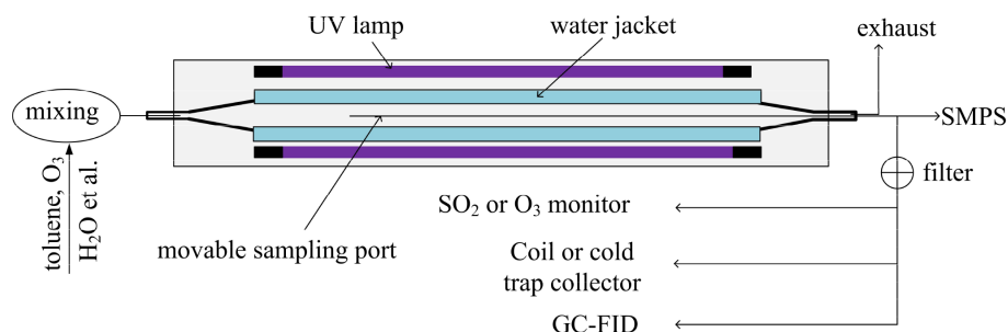
Figure 1. Schematic diagram of the experimental setup.
