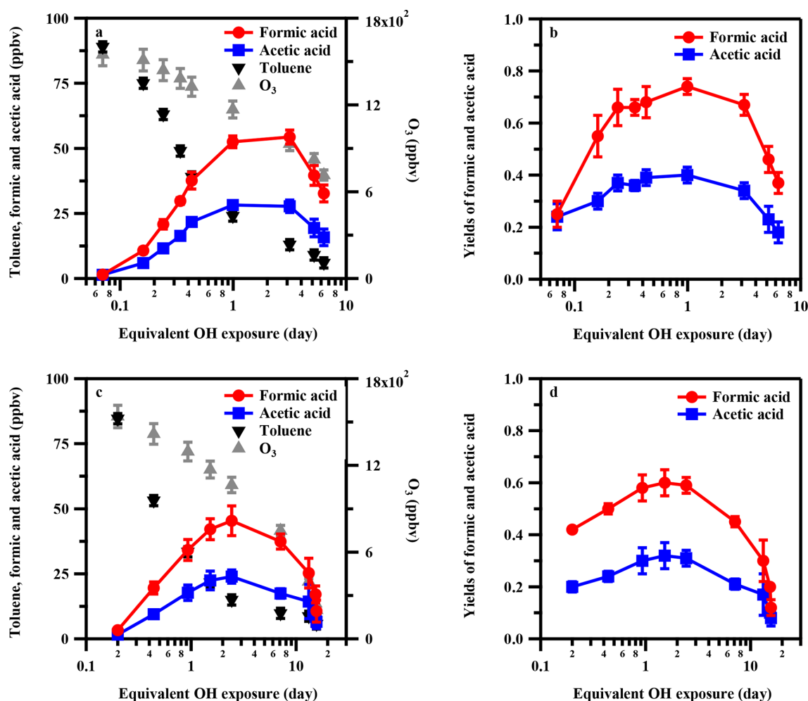
Figure 2. Production of formic acid and acetic acid during the photooxidation of toluene as a function of \bullet\text{OH} exposure. Panels (a) and (b) correspond to 20 % RH, and panels (c) and (d) correspond to 70 % RH. The initial toluene concentration was \sim 94 ppbv. Error bars represent standard deviations of repeated experiments under identical conditions. Note that the first data point in each panel corresponds to a condition where measurable toluene consumption has already occurred, with \bullet\text{OH} exposures of 0.07 equivalent days at 20 % RH and 0.2 equivalent days at 70 % RH, respectively.
