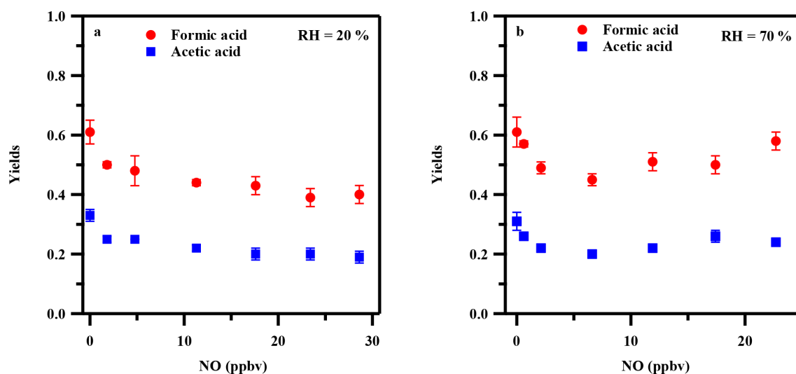
Figure 3. \text{NO}_x dependence of formic acid and acetic acid yields under 20 % RH (a) and 70 % RH (b) conditions. Error bars represent standard deviations from repeated experiments under identical conditions.
