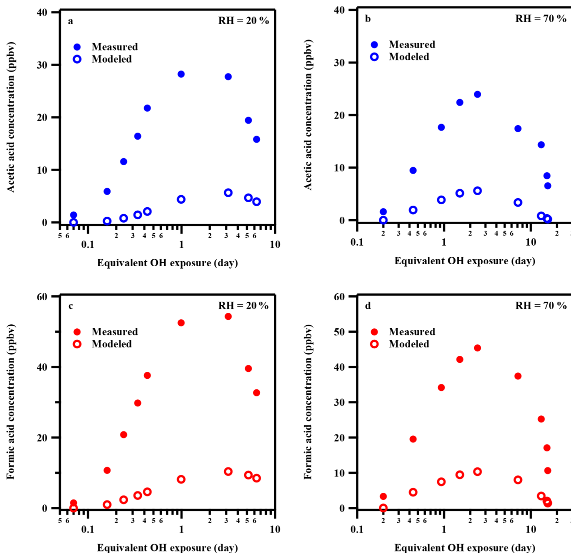
Figure 4. Comparison of measured and modeled concentrations of formic acid and acetic acid at different \bullet OH exposures. (a) Acetic acid at 20 % RH; (b) Acetic acid at 70 % RH; (c) Formic acid at 20 % RH; (d) Formic acid at 70 % RH.
