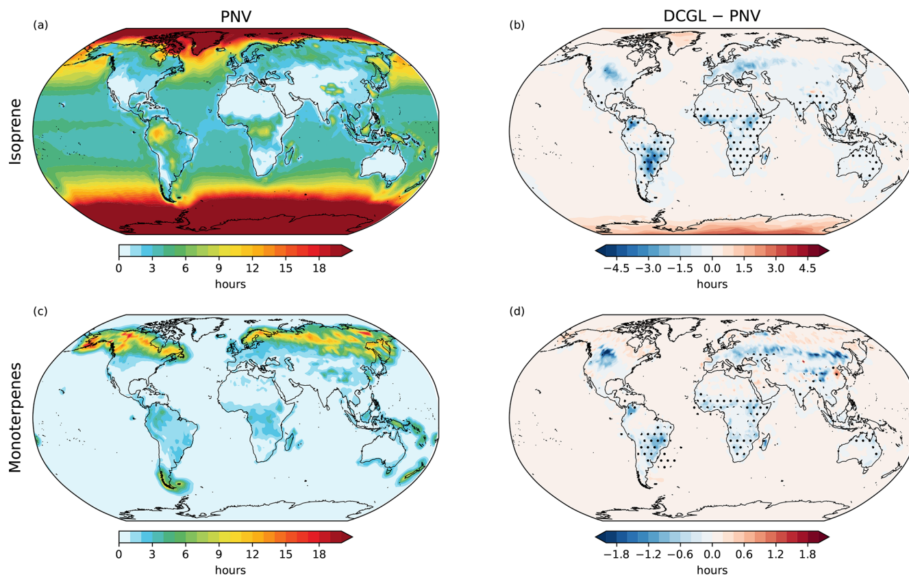
Figure 3. Spatial distribution of isoprene (a) and monoterpene (c) chemical lifetime against OH and O 3 oxidation at the surface. Panels (b) and (d) show the changes (DCGL – PNV) in isoprene and monoterpene lifetimes, respectively. Dot hatching indicates a statistically significant change based on a two-tailed Student's t test with 95 % confidence.
