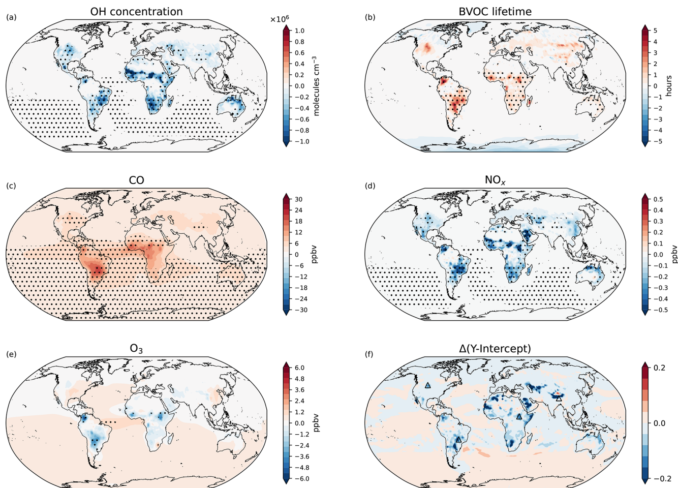
Figure 9. Absolute changes in atmospheric states resulting from the restoration of present-day grazing land (DCGL – DCL). Maps show variations in (a) surface OH concentration, (b) BVOC lifetime, (c) CO surface mixing ratio, (d) NO x surface mixing ratio, (e) O 3 surface mixing ratio, and (f) changes in O 3 production sensitivity. Dot hatching indicates a statistically significant change based on a two-tailed Student's t test with 95 % confidence.
