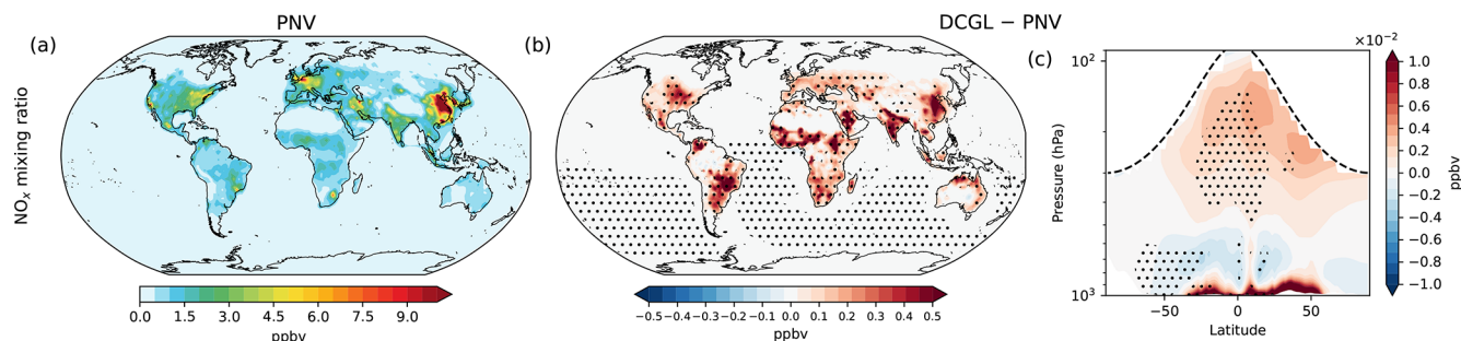
Figure 5. Same as Fig. 4a–c but for NO x .
