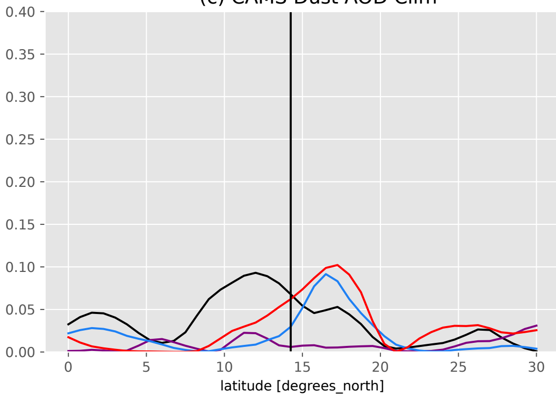
(c) CAMS Dust AOD Clim
