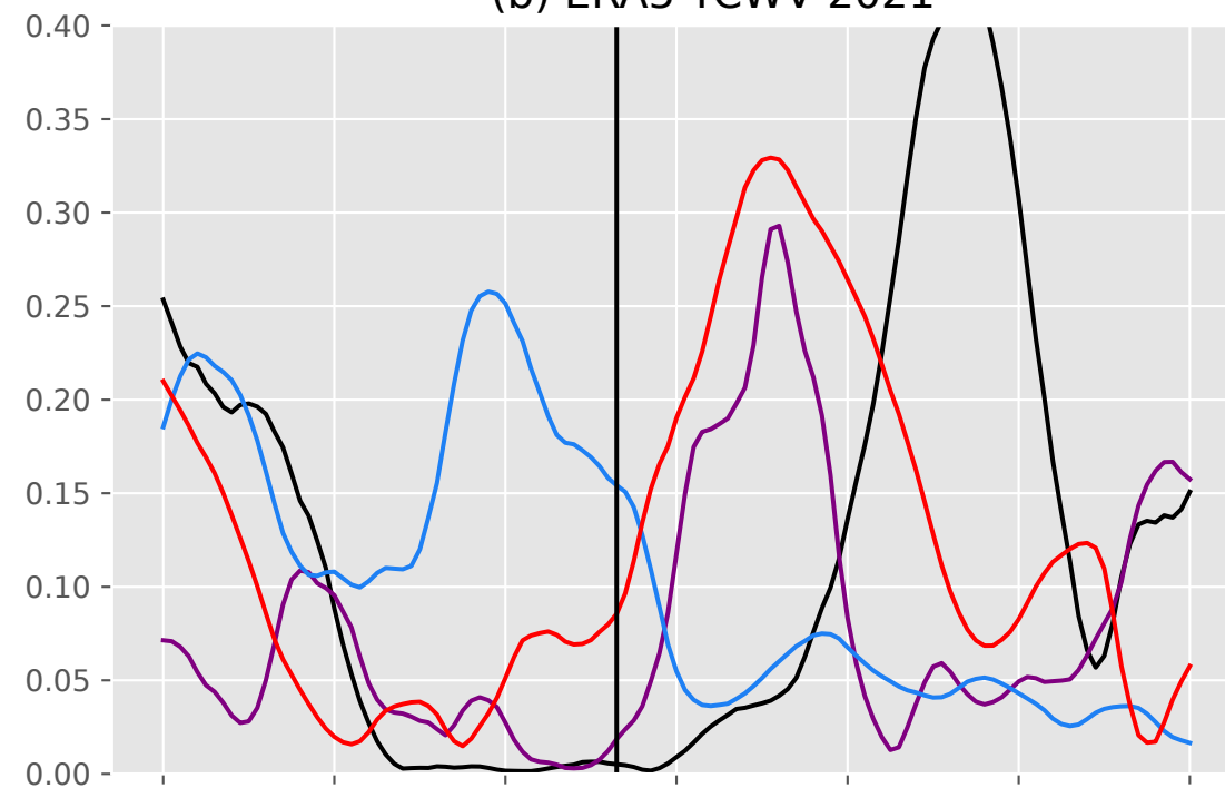
(b) ERA5 TCWV 2021
