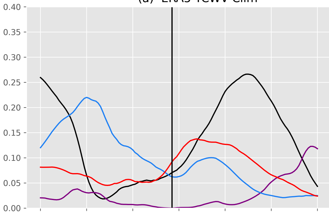
(a) ERA5 TCWV Clim
